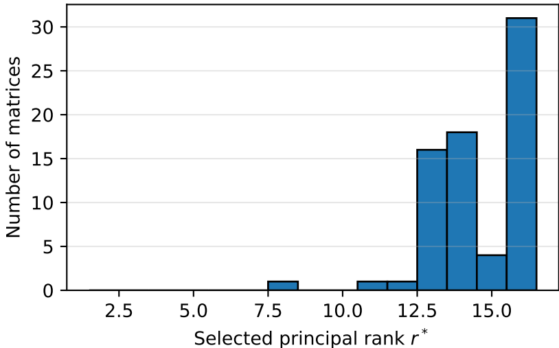
Distribution over 72 q_proj/v_proj matrices
