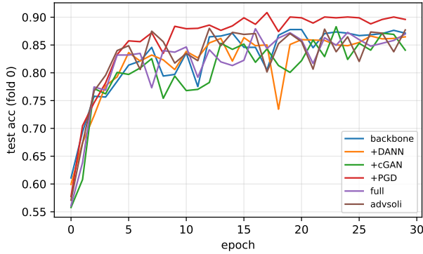
Figure 4. Test accuracy versus epoch on fold 0 for each ablation variant. PGD-only is the most stable. DANN-containing variants oscillate the most.
