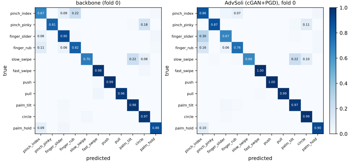
Figure 3. Row-normalized confusion matrices on fold 0. The biggest remaining error after AdvSoli is finger_slider \rightarrow pinch_index (0.30 vs 0.06 for the backbone), which is the cost of using cGAN augmentation on this small dataset.
