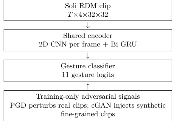
Figure 1. AdvSoli architecture. A compact 2D-CNN+Bi-GRU encoder feeds the gesture classifier. During training, PGD creates adversarial inputs and a conditional GAN supplies additional fine-grained radar clips. At test time, only the encoder and classifier are used.
