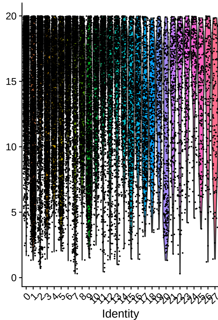
percent.mt
