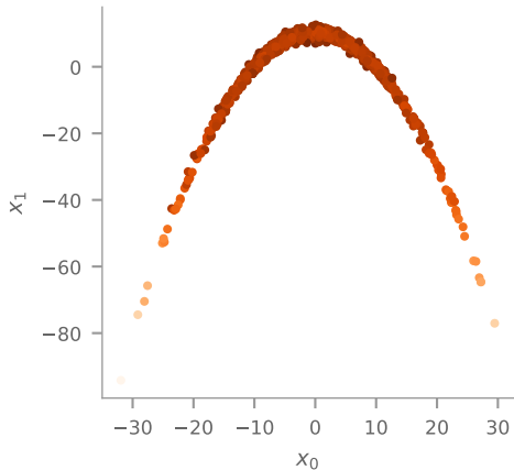
single-Gaussian reference: residual spans 23 nats
