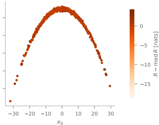
learned transport atlas: residual spans 4 nats
