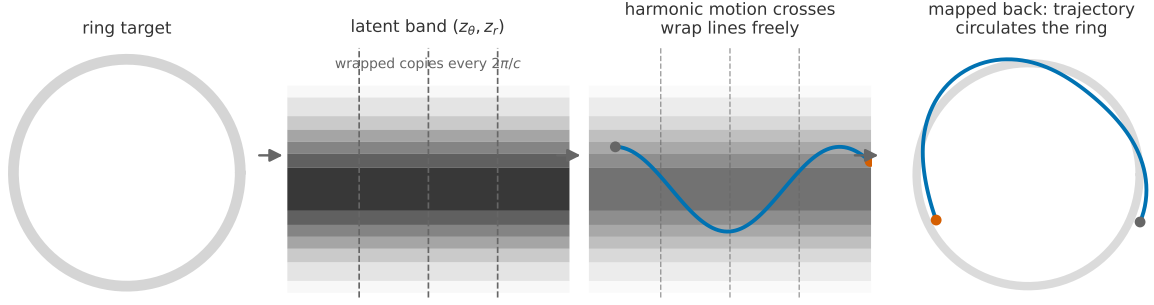
Figure 3: The winding chart, step by step. A closed ridge is unwrapped into a latent band on which the angular coordinate repeats every 2\pi/c ; harmonic motion travels freely along the band, and mapping back yields a trajectory that circulates the ring—the geometry that defeats arc-by-arc mixtures of local charts. Exactness under the non-injective map requires the fiber-summed density (2) and branch-sampled inversion (15) (Lemma 3).
