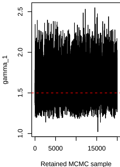
gamma_1 convergence
