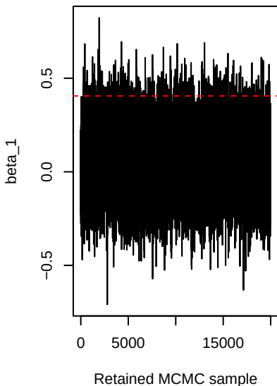
beta_1 convergence
