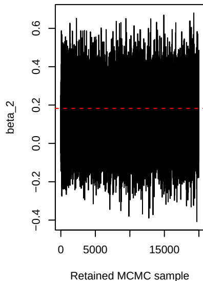
beta_2 convergence
