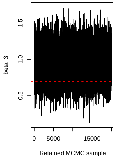
beta_3 convergence
