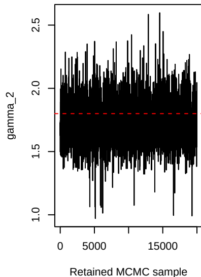
gamma_2 convergence
