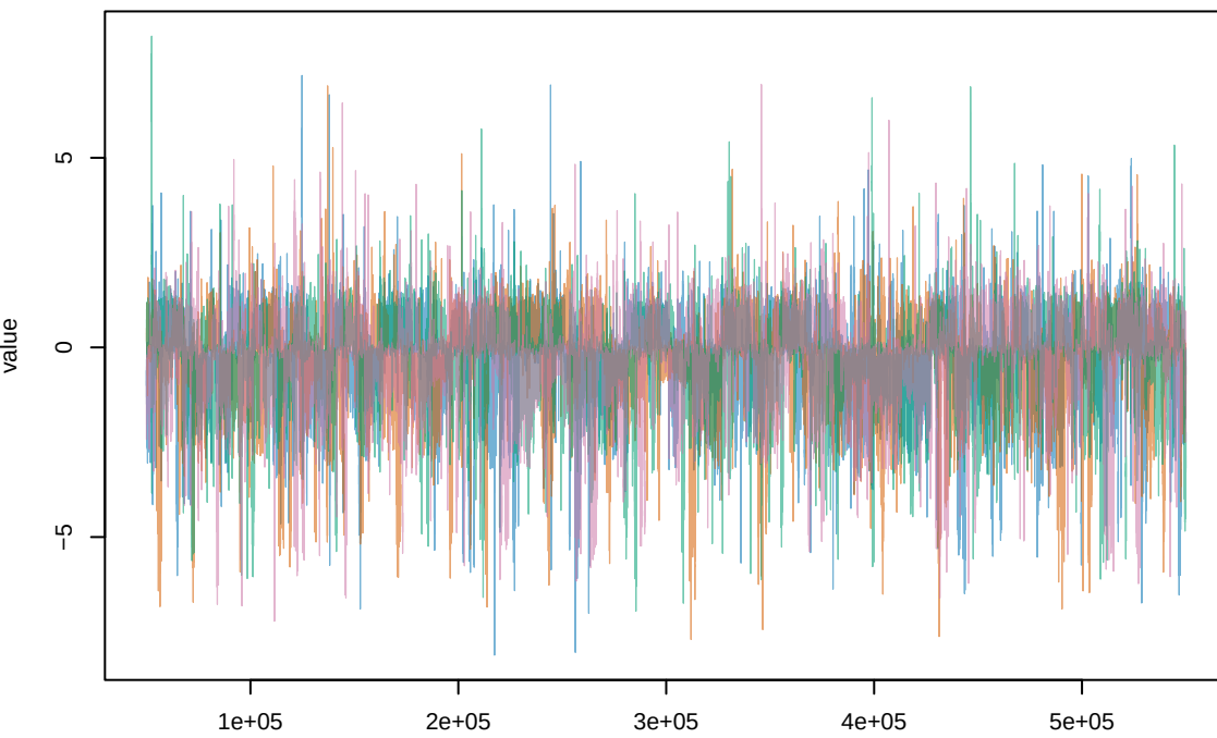
beta_treatment
