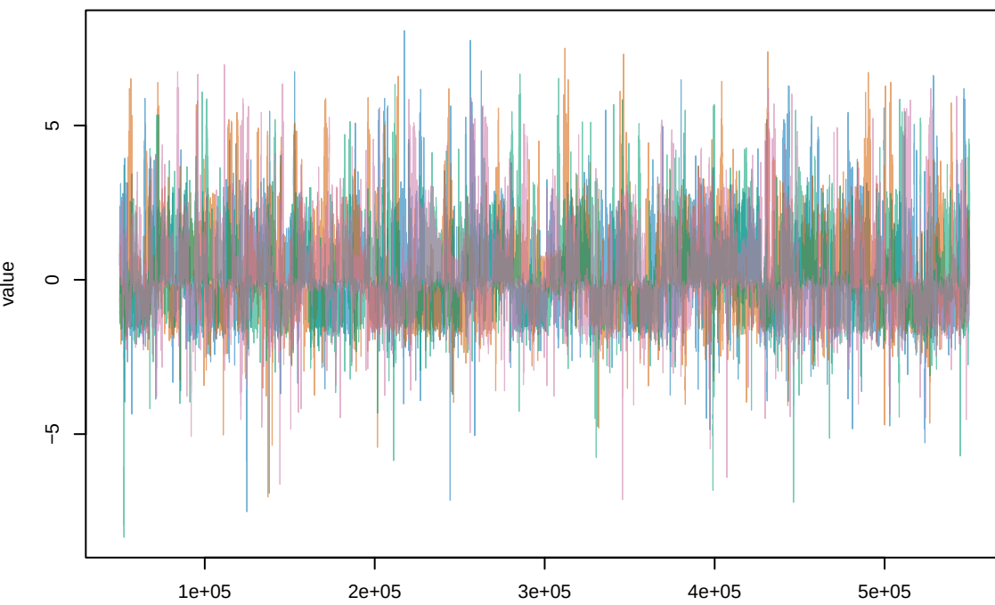
beta_treatment_x_subgroup
