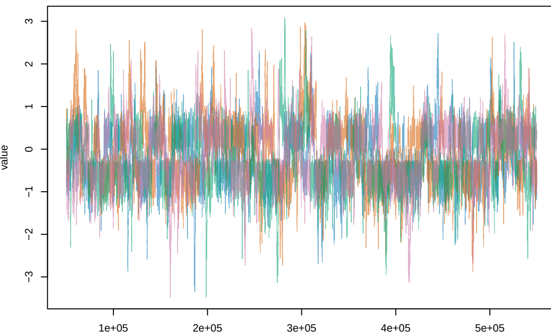
gamma_bio37
