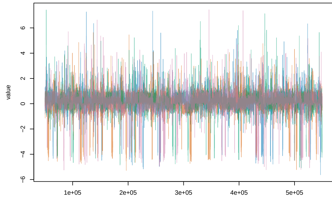
beta_subgroup
