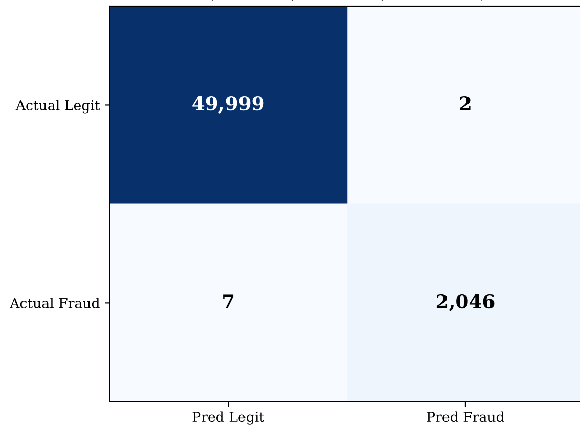
(c) Confusion Matrix — Hybrid (P=0.999, R=0.997, F1=0.998)
