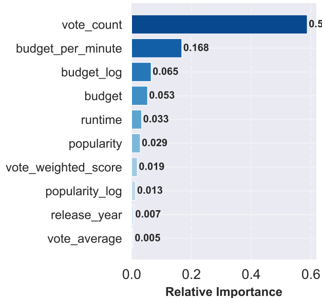
(b) Gradient Boosting
