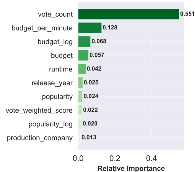
(a) Random Forest (Tuned)
