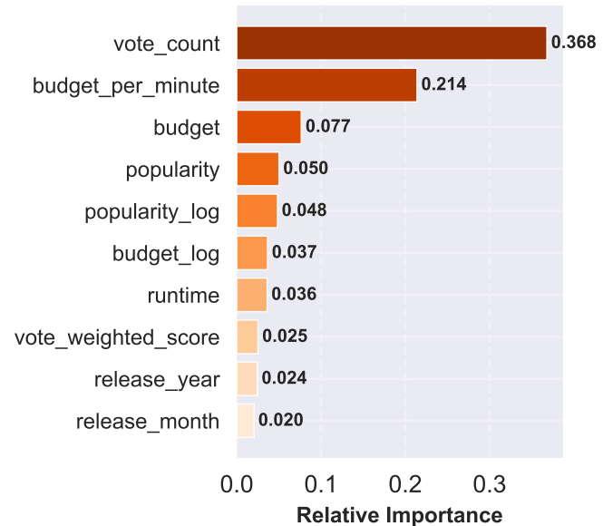
(c) XGBoost (Tuned)
