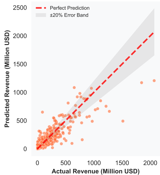
(a) XGBoost (Tuned)
