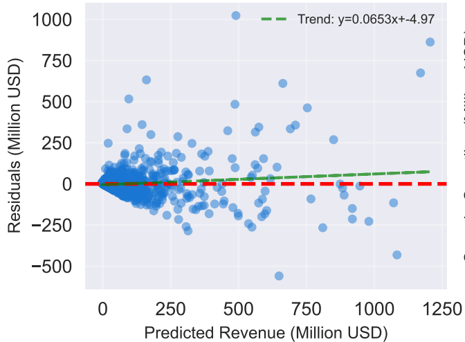
(a) Residual Distribution
