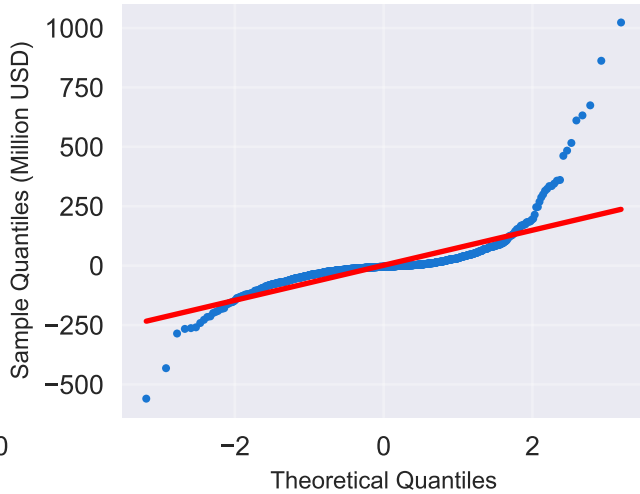
(b) Normality Assessment (Q-Q Plot)
