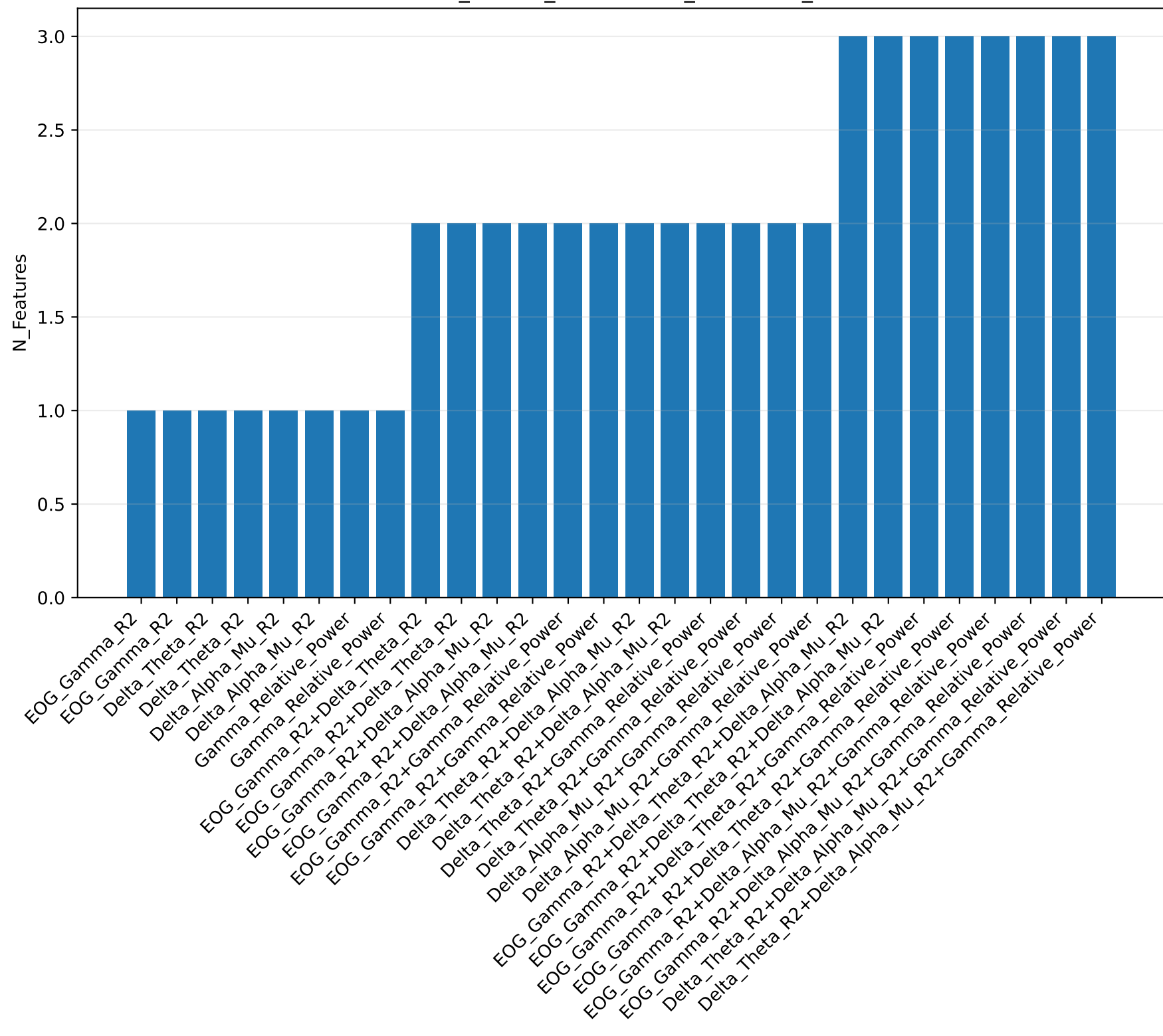
lambda075 benefit multivariate models: N Features
