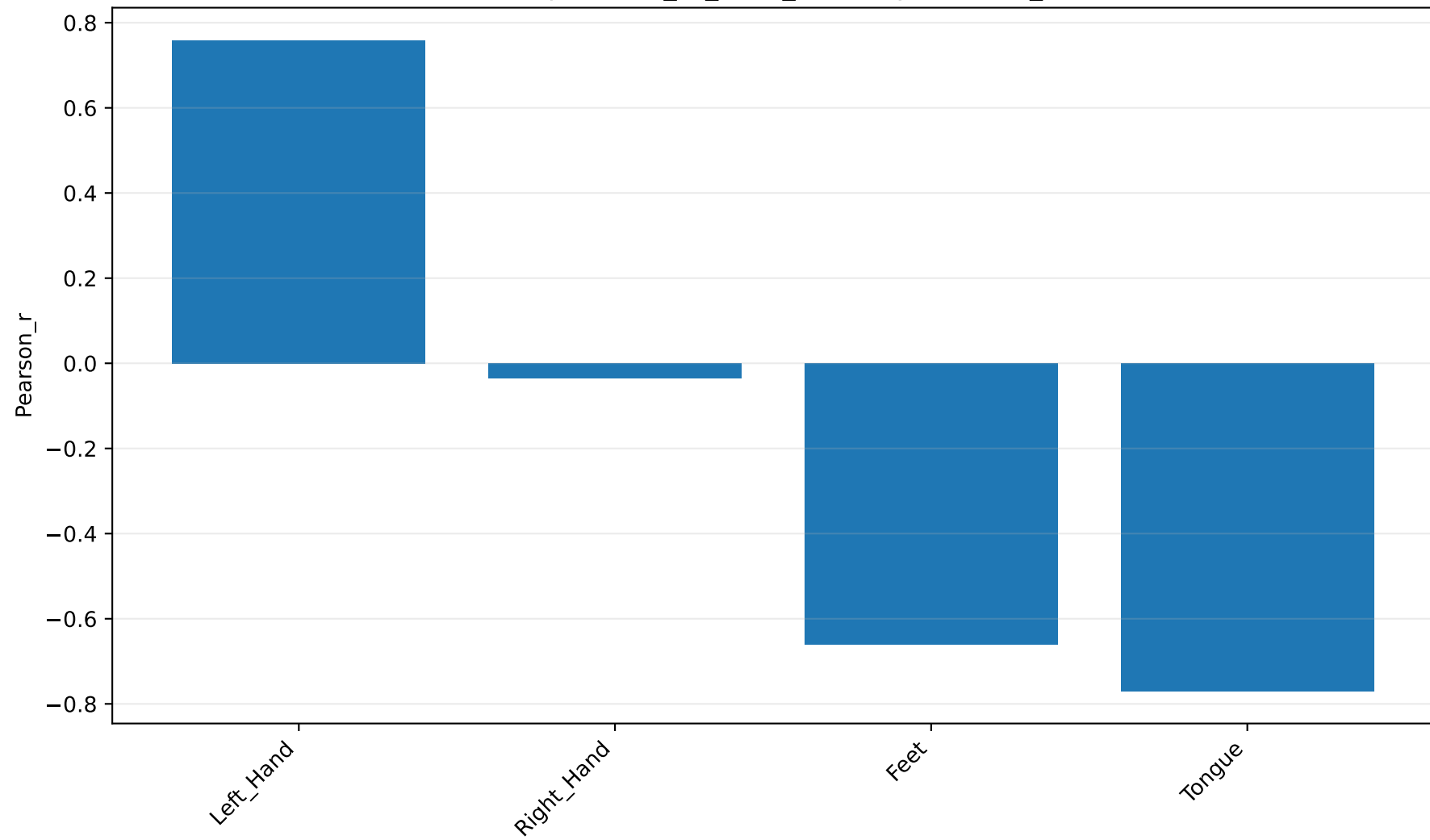
compactness_vs_class_accuracy: Pearson_r
