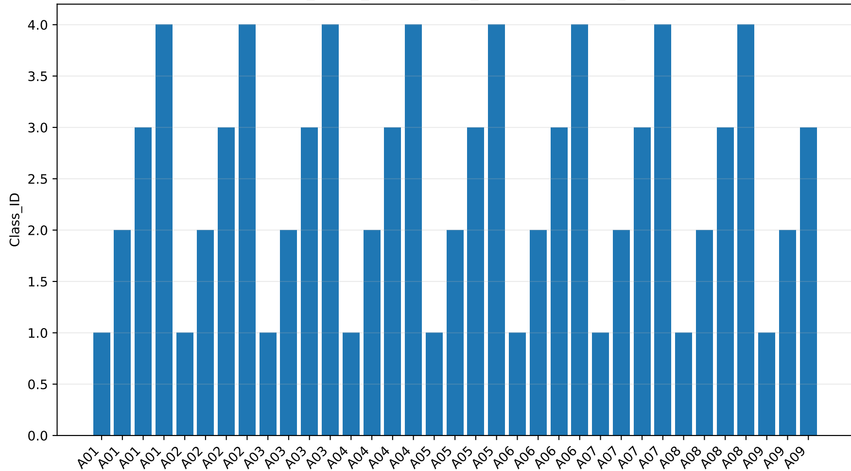
class_motor_lateralization_lambda075: Class_ID
