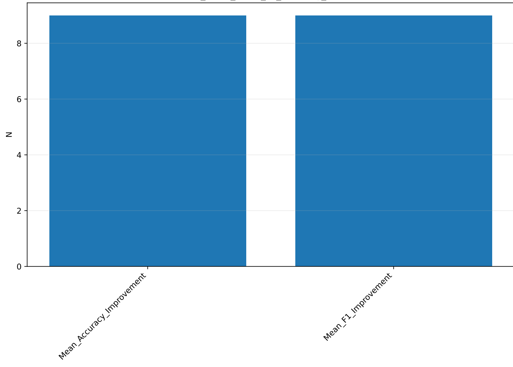
nested_loocv_score_vs_cleaning_benefit: N
