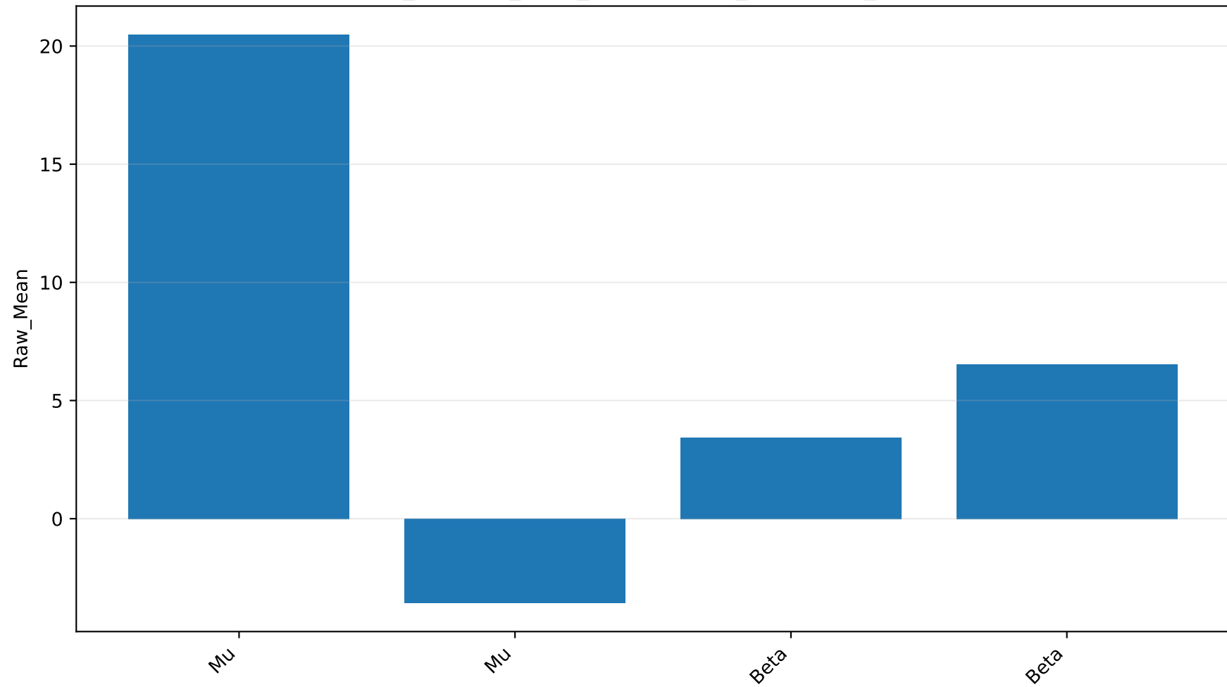
full_duration_hand_lateralization_tests: Raw_Mean
