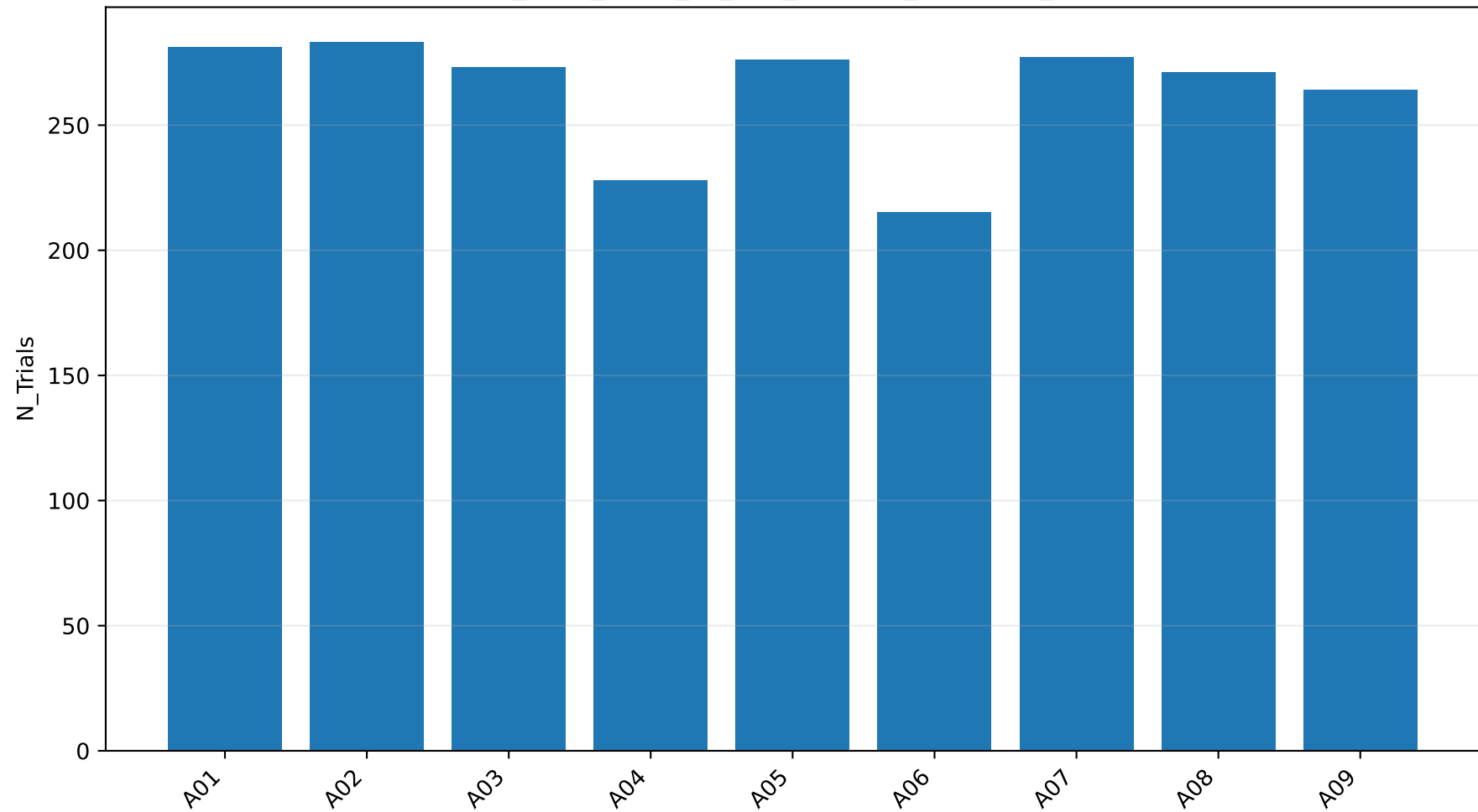
eog_error_slope_vs_eeg_spectral_profile: N_Trials
