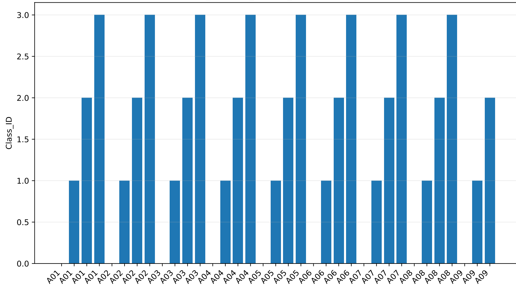
class_decision_margin_results: Class_ID
