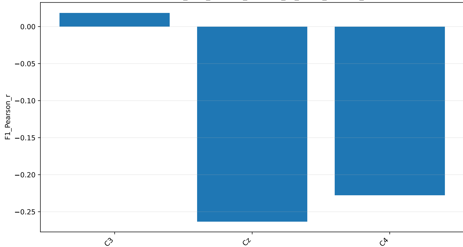
normalized_beta_channel_contrast_vs_f1: F1_Pearson_r
