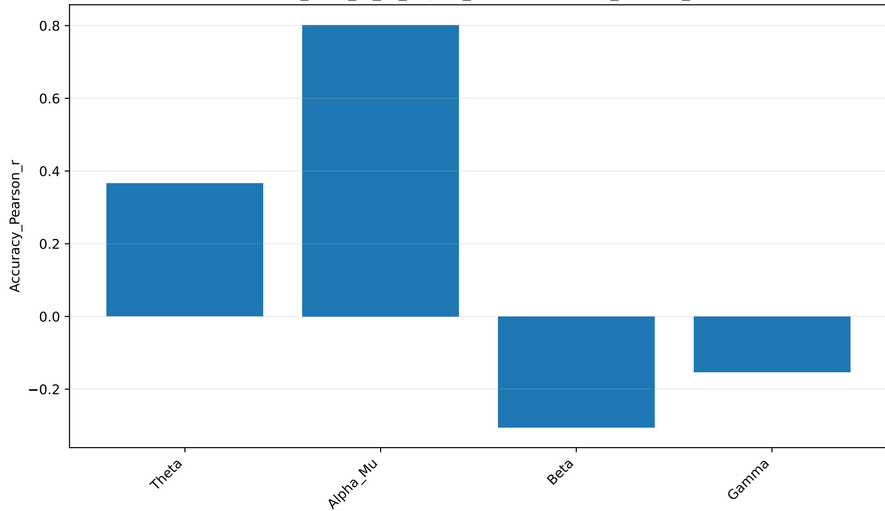
band_class_r2_vs_eegnet_benefit: Accuracy_Pearson_r
