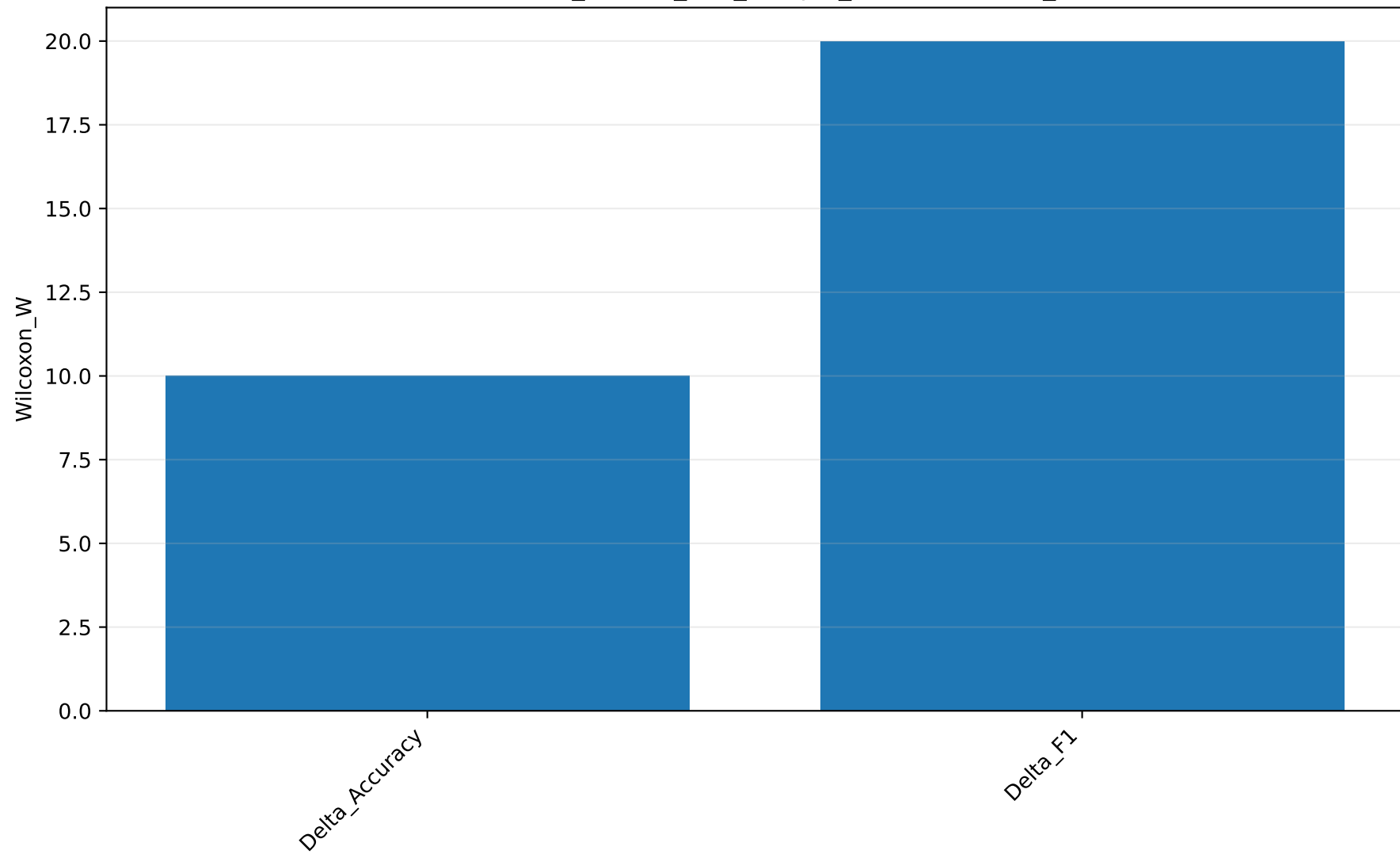
lambda075_benefit_one_sample_tests: Wilcoxon_W
