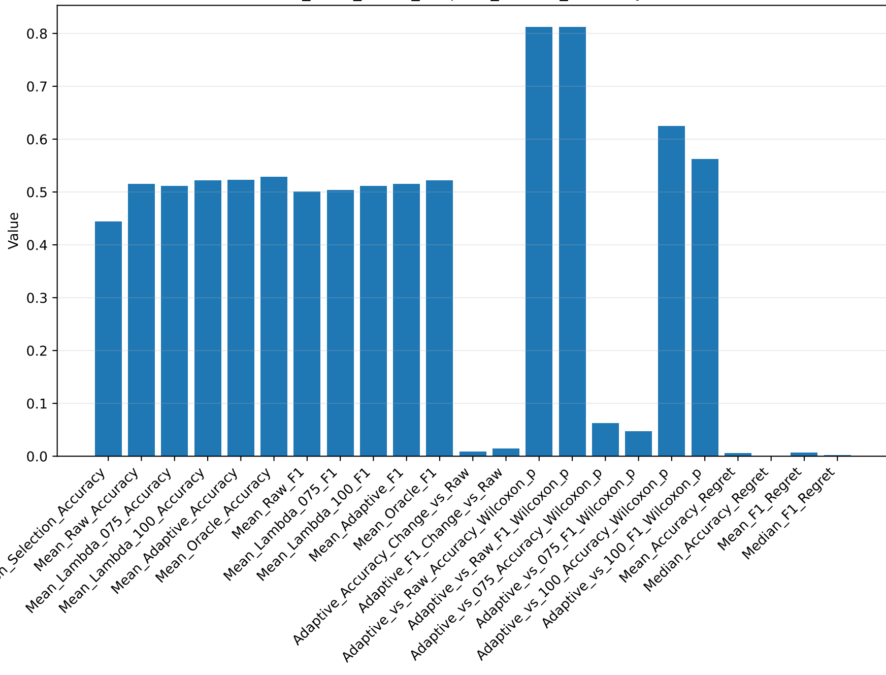
nested_three_action_adaptive_lambda_summary: Value
