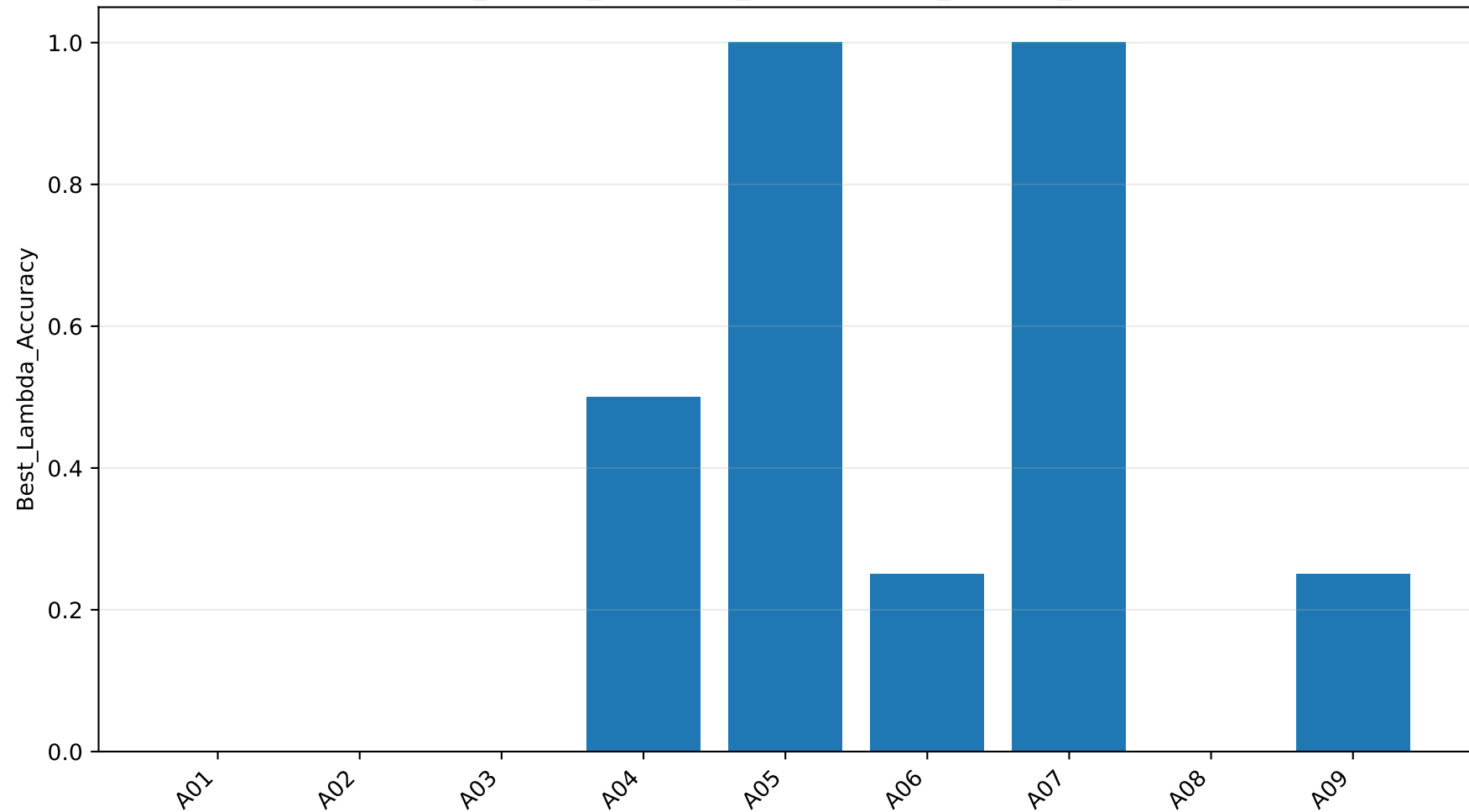
subject_lambda_prediction_features: Best_Lambda_Accuracy
