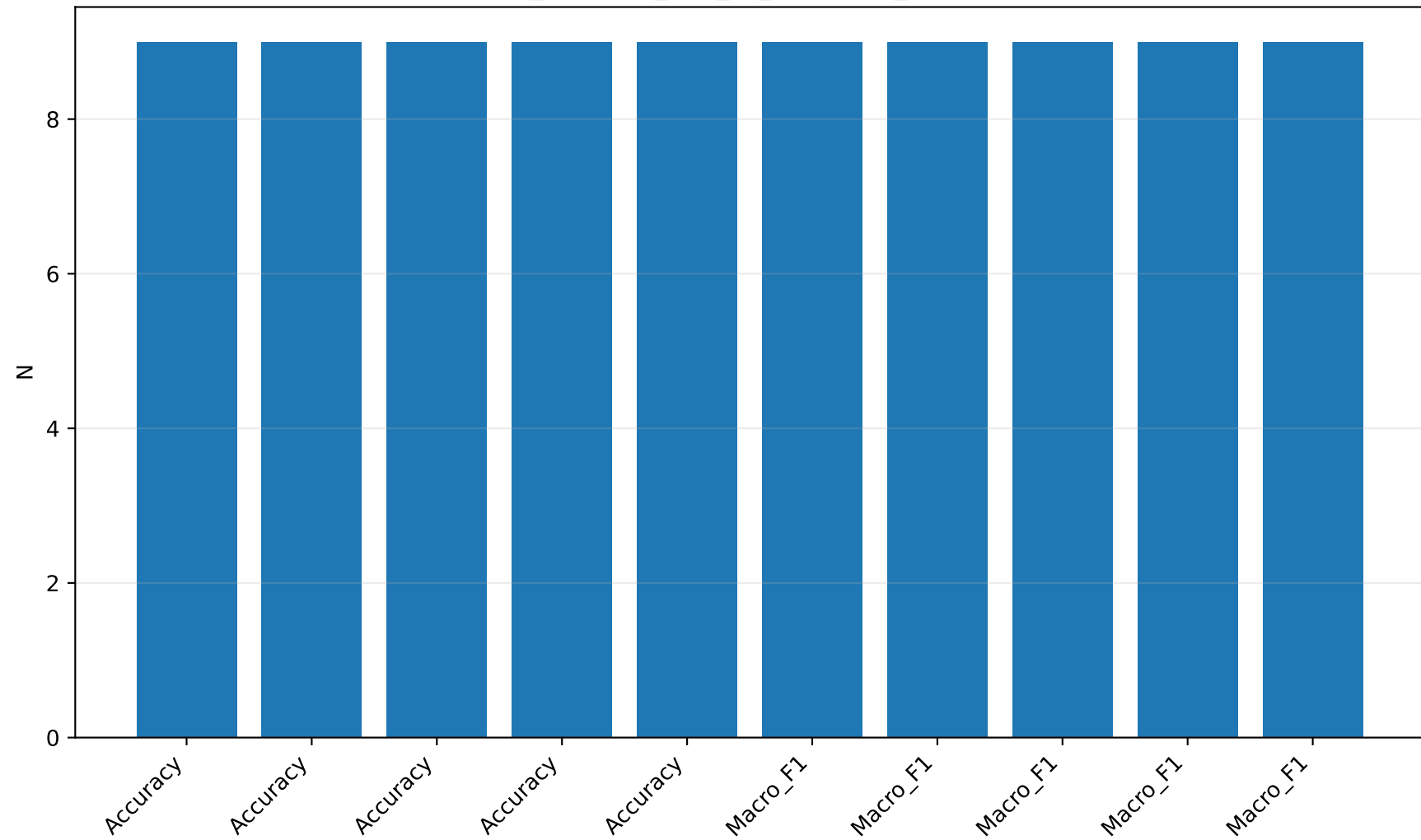
eegnet_cleaning_raw_vs_condition_statistics: N
