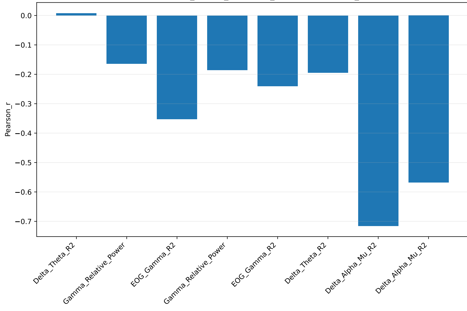
lambda075_benefit_candidate_scorecard: Pearson_r
