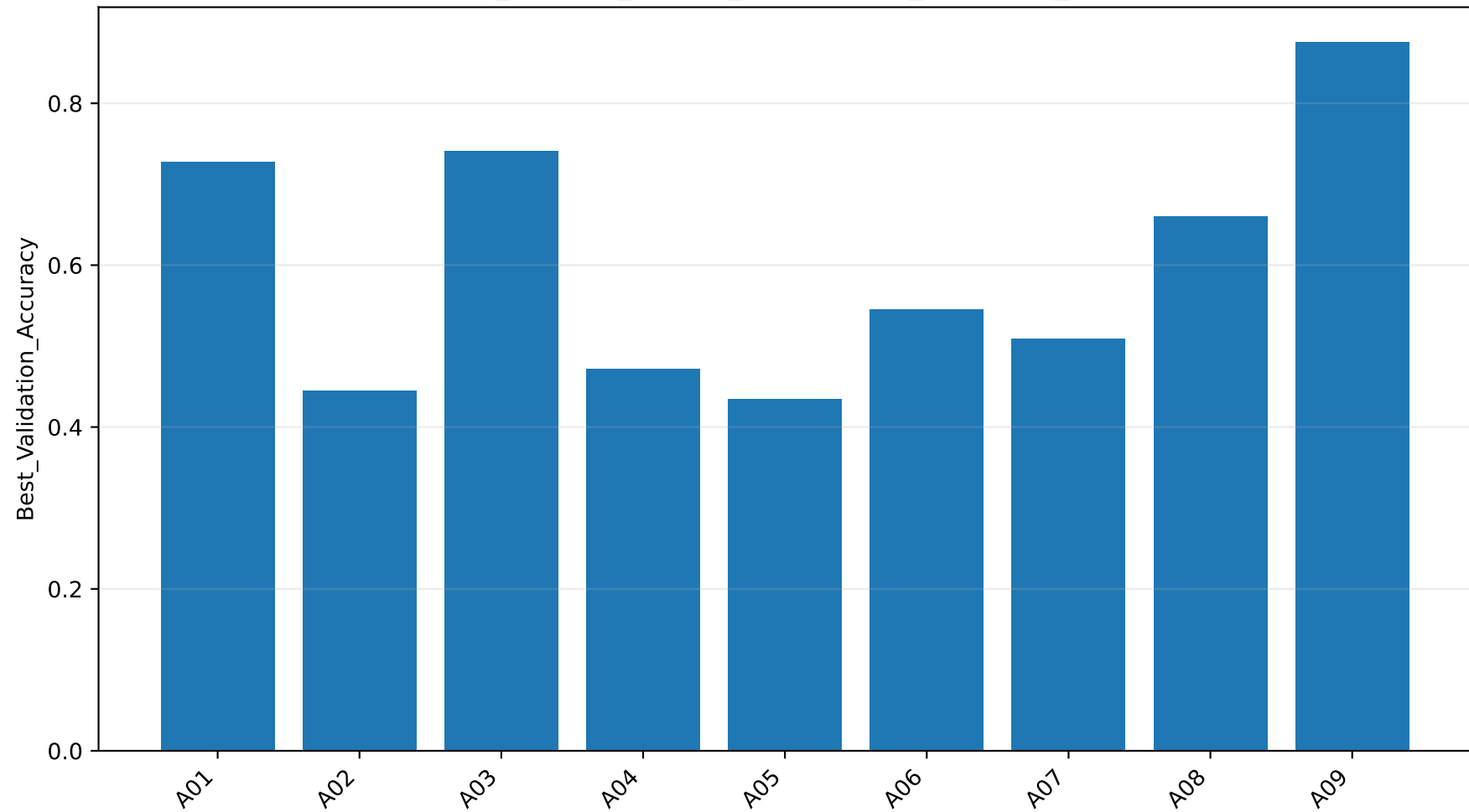
common_network_subject_results: Best_Validation_Accuracy
