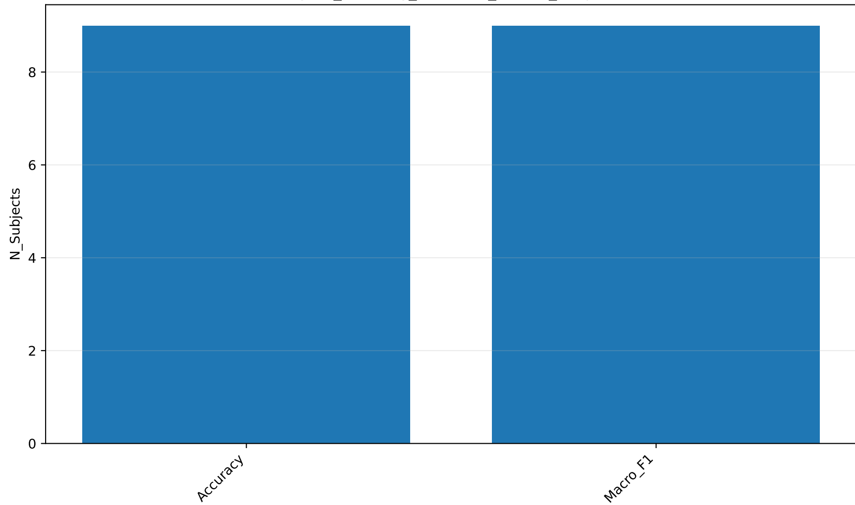
eegnet_cleaning_friedman_test: N_Subjects
