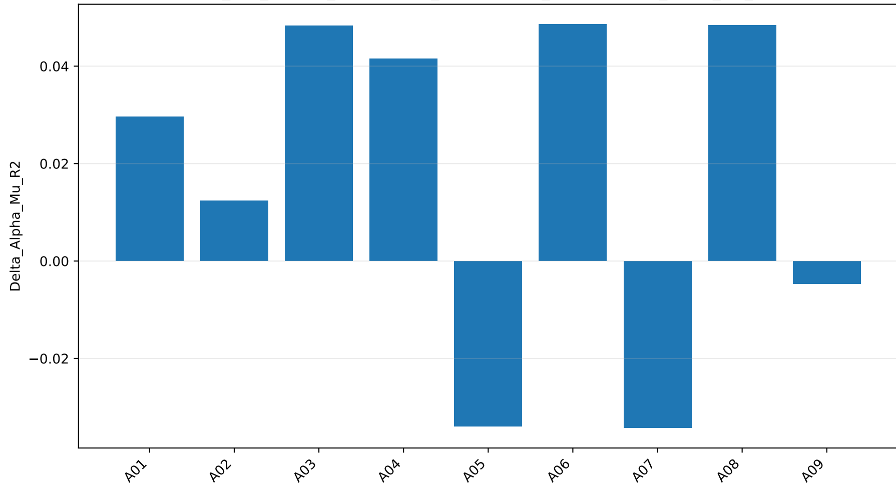
mi_eog_change_suppression_performance_master: Delta_Alpha_Mu_R2
