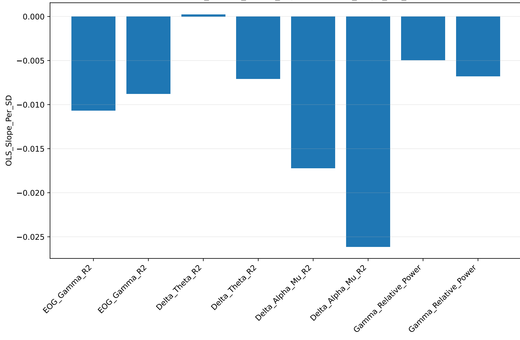
lambda075_benefit_robust_regression: OLS_Slope_Per_SD
