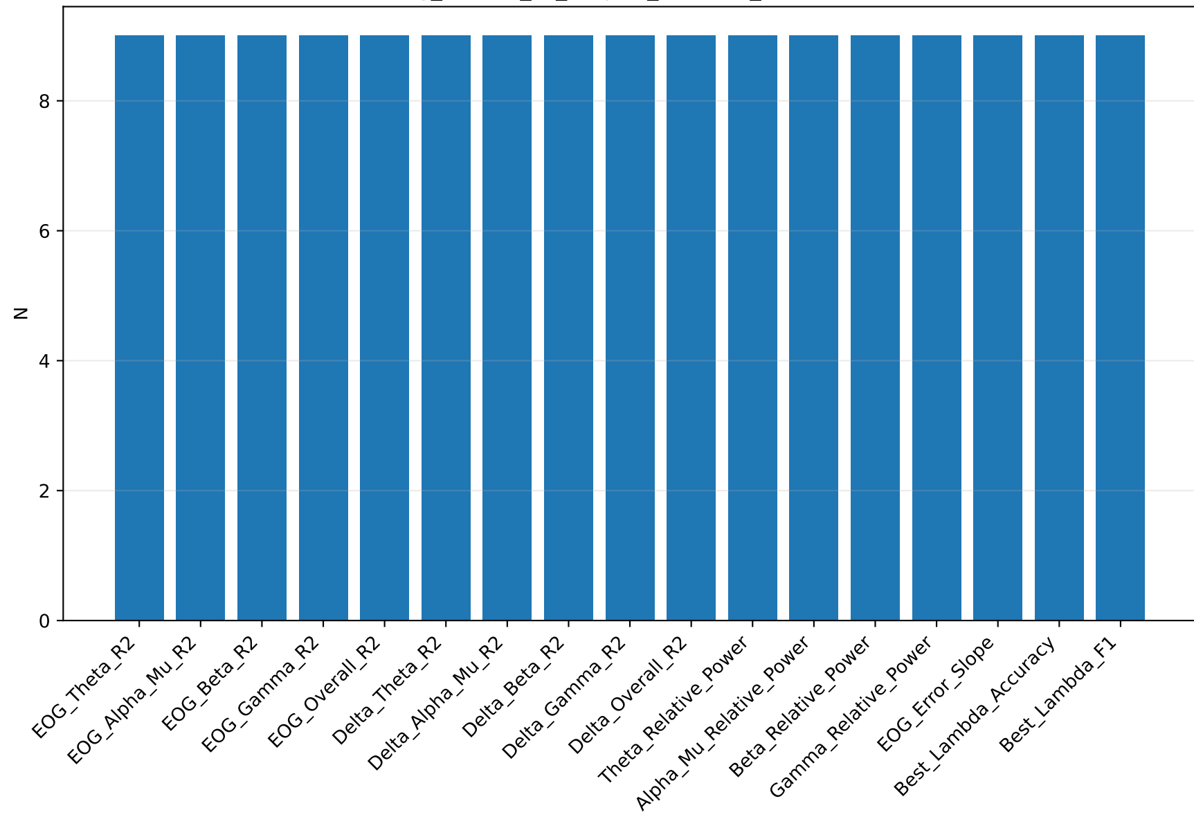
cleaning_benefit_vs_subject_features_correlations: N
