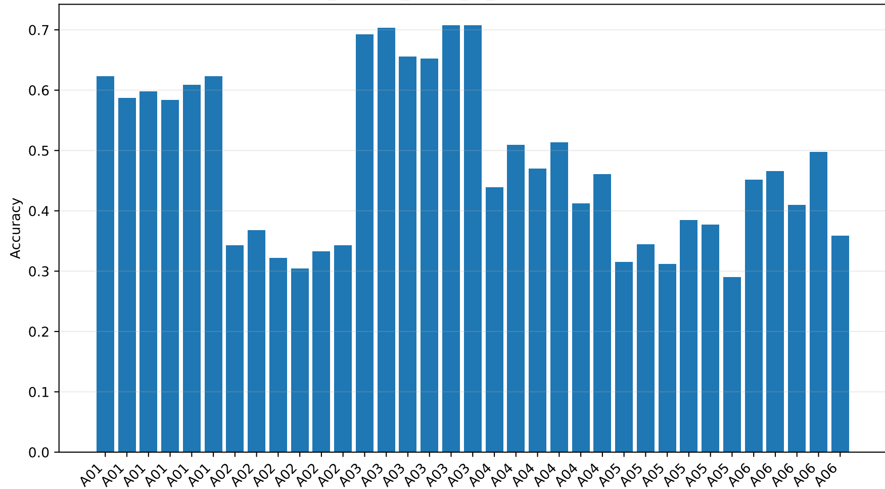
eeg_spectral_profile_vs_cleaning: Accuracy
