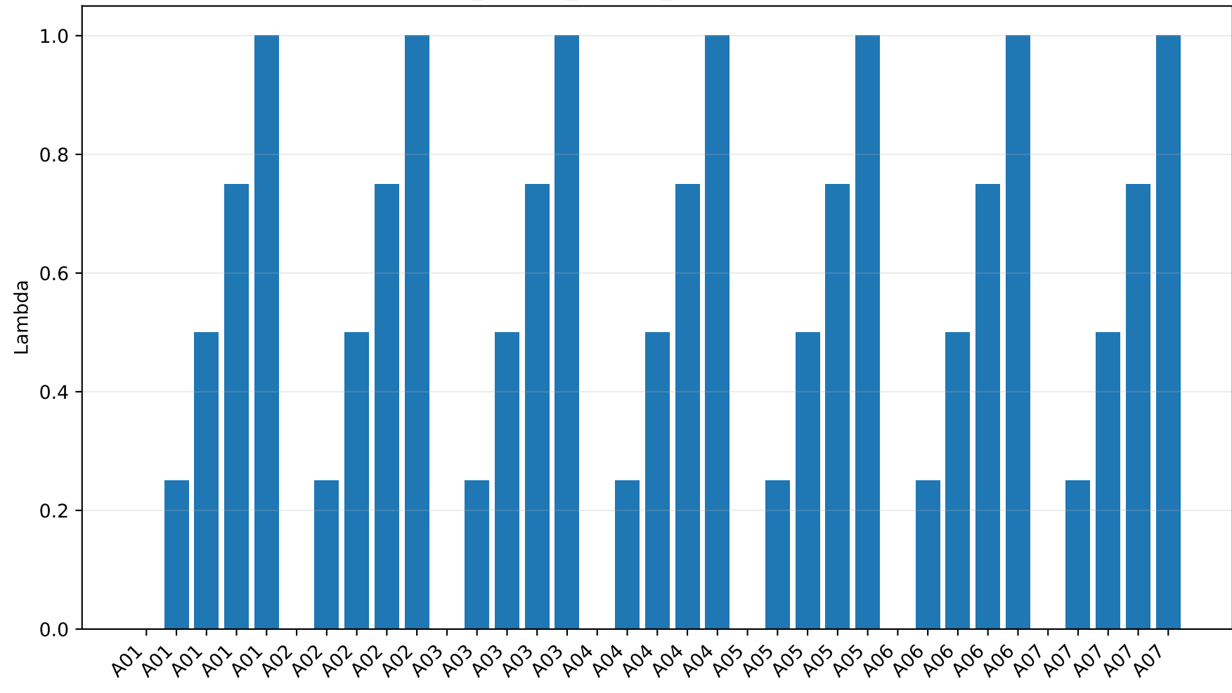
eegnet_allband_lambda_performance: Lambda
