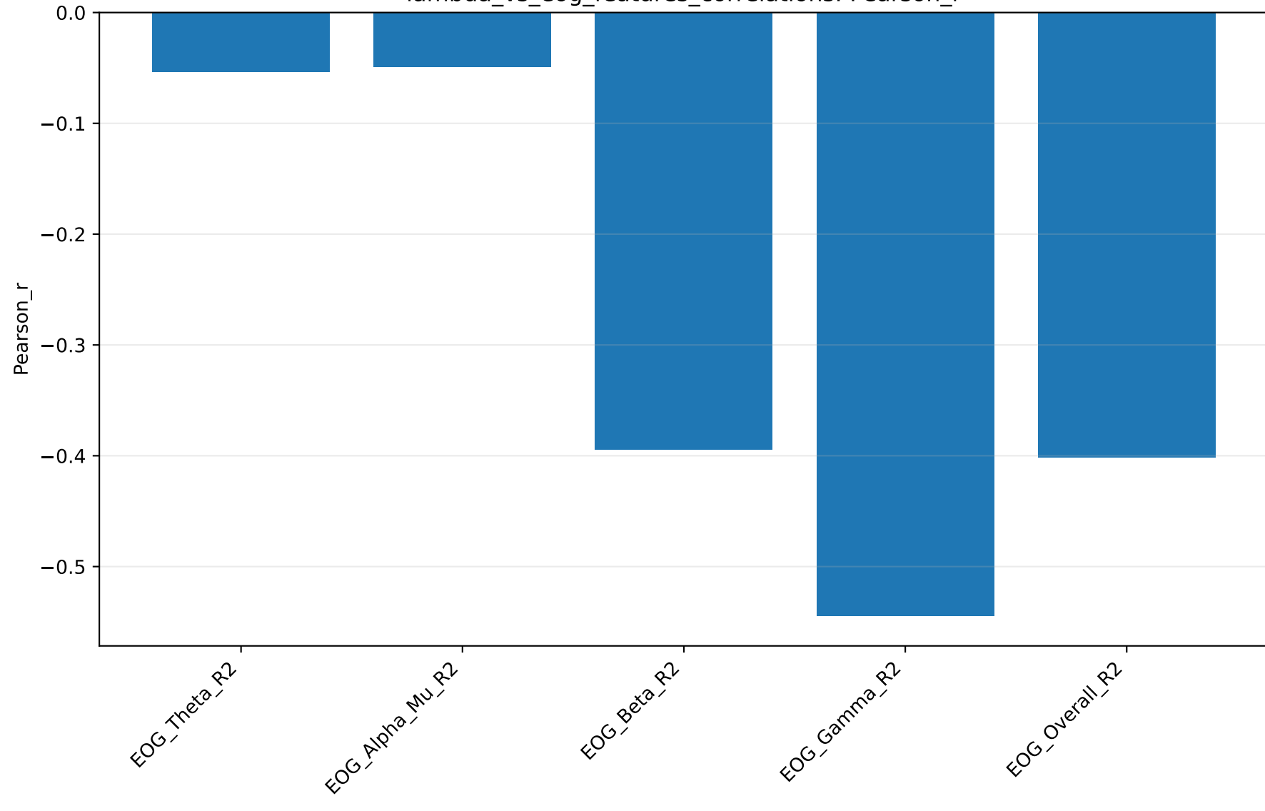
lambda_vs_eog_features_correlations: Pearson_r
