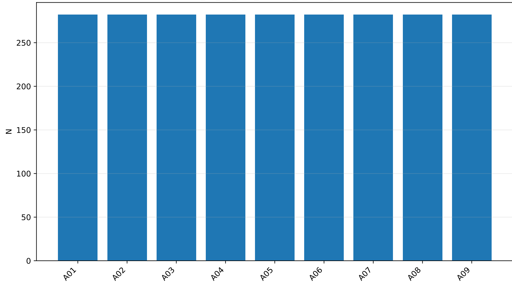
baseline_vs_mi_eog_subject_overall_statistics: N
