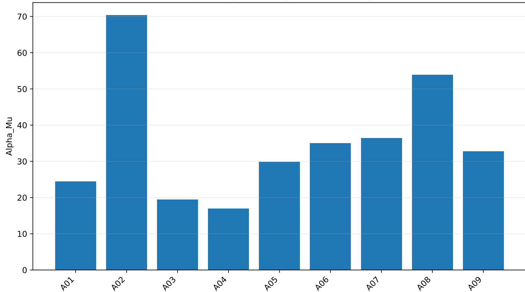
eog_subject_frequency_summary: Alpha_Mu
