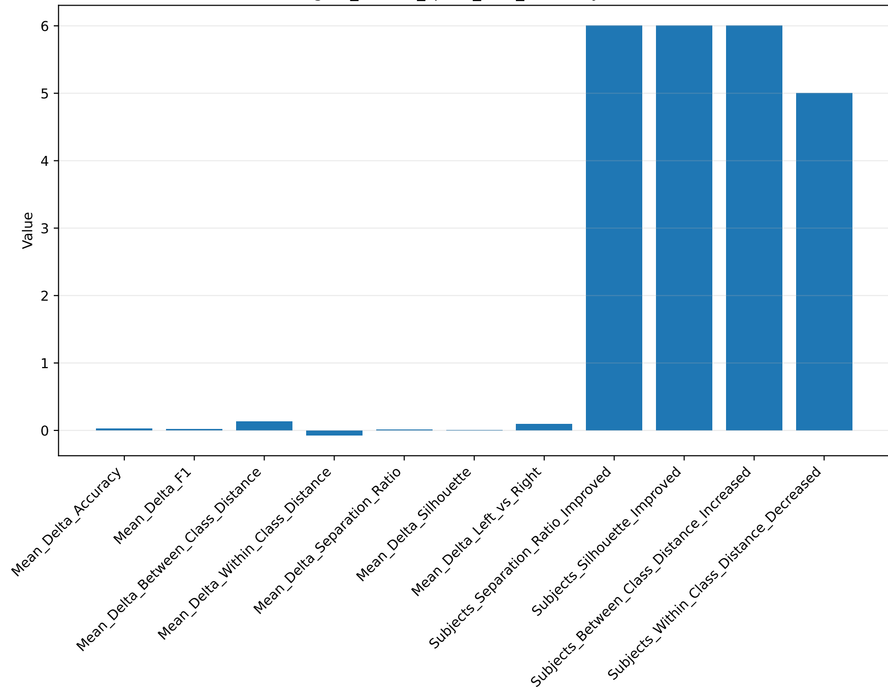
eegnet_feature_space_final_summary: Value
