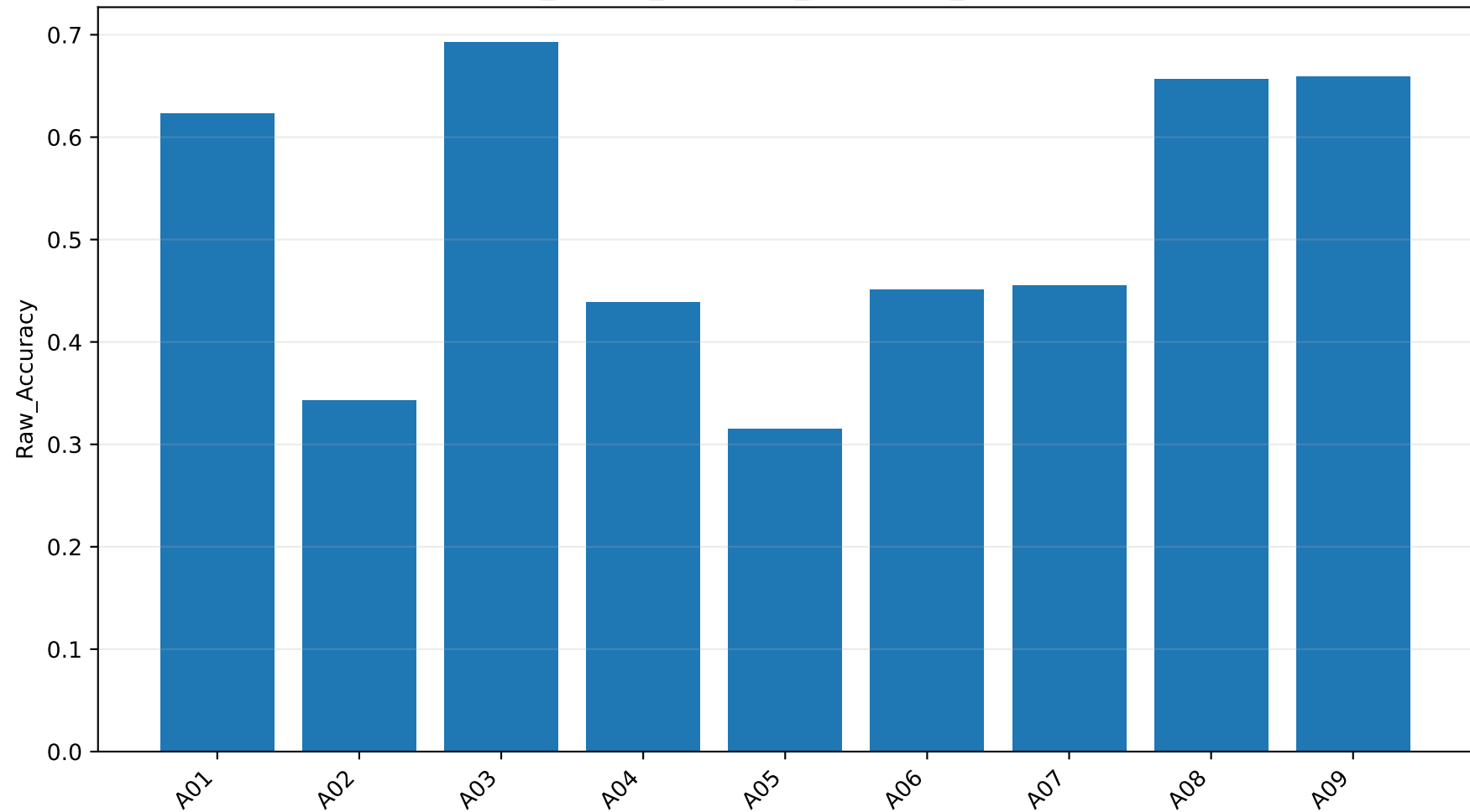
final_master_validation_table: Raw_Accuracy
