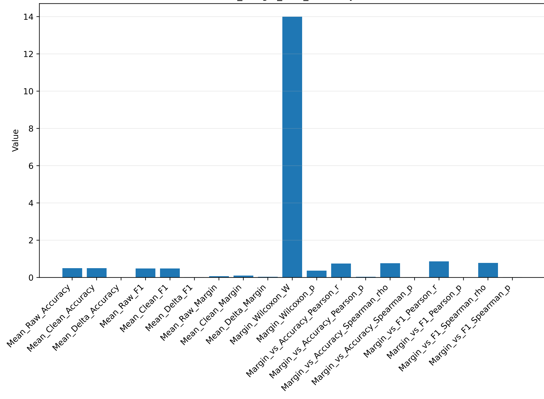
decision_margin_final_summary: Value
