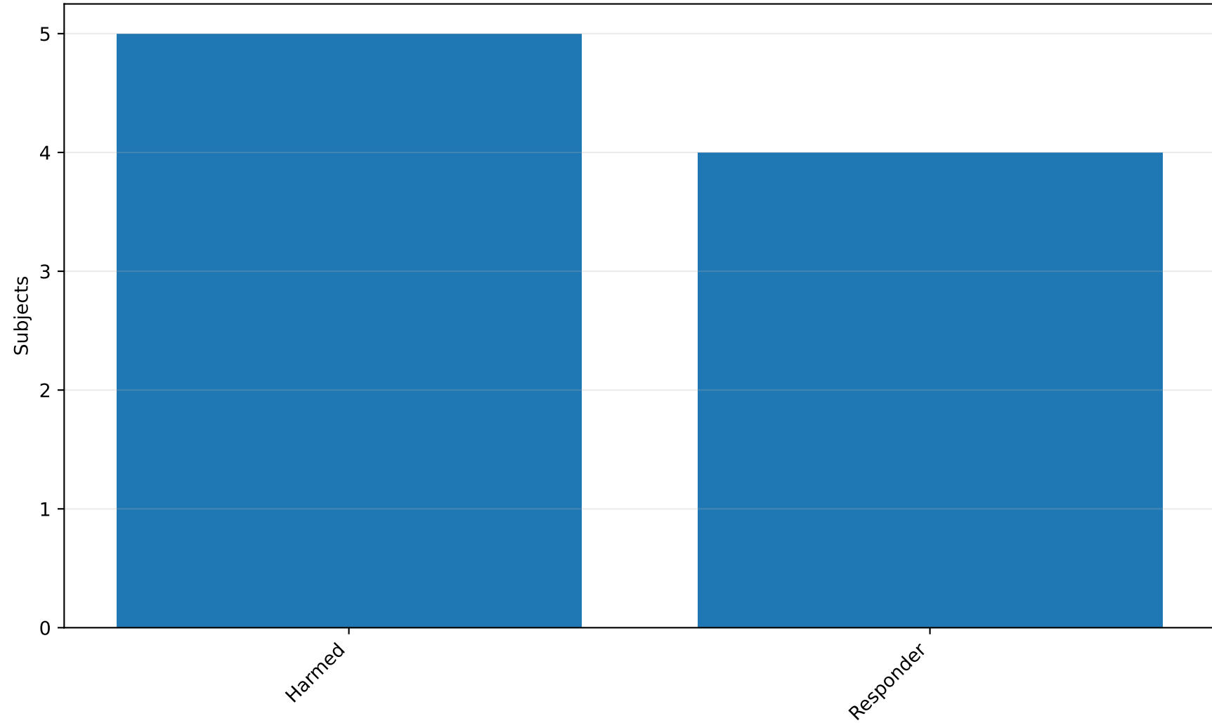
cleaning_response_group_summary: Subjects
