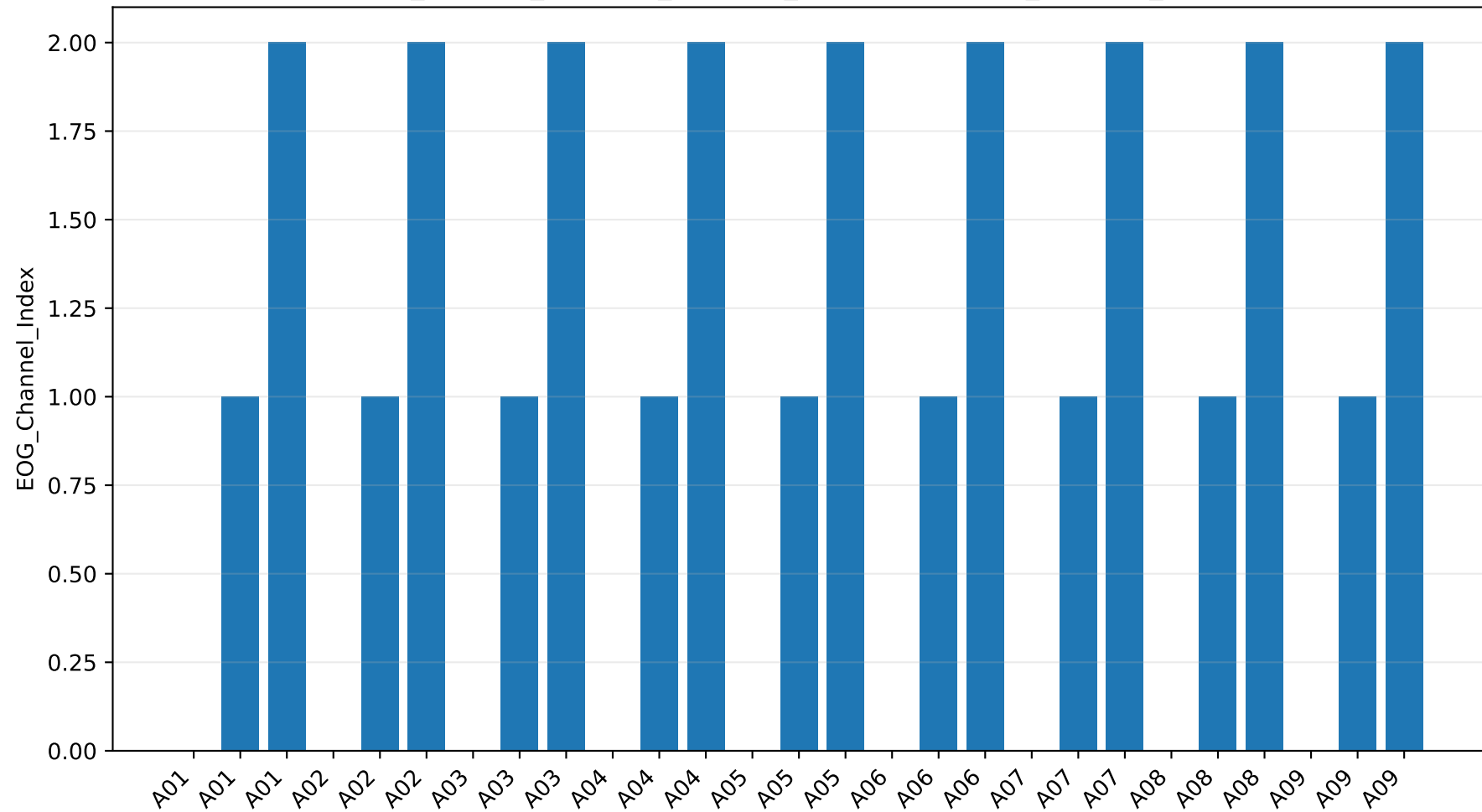
eog_channel_coupling_changes_lambda075: EOG_Channel_Index
