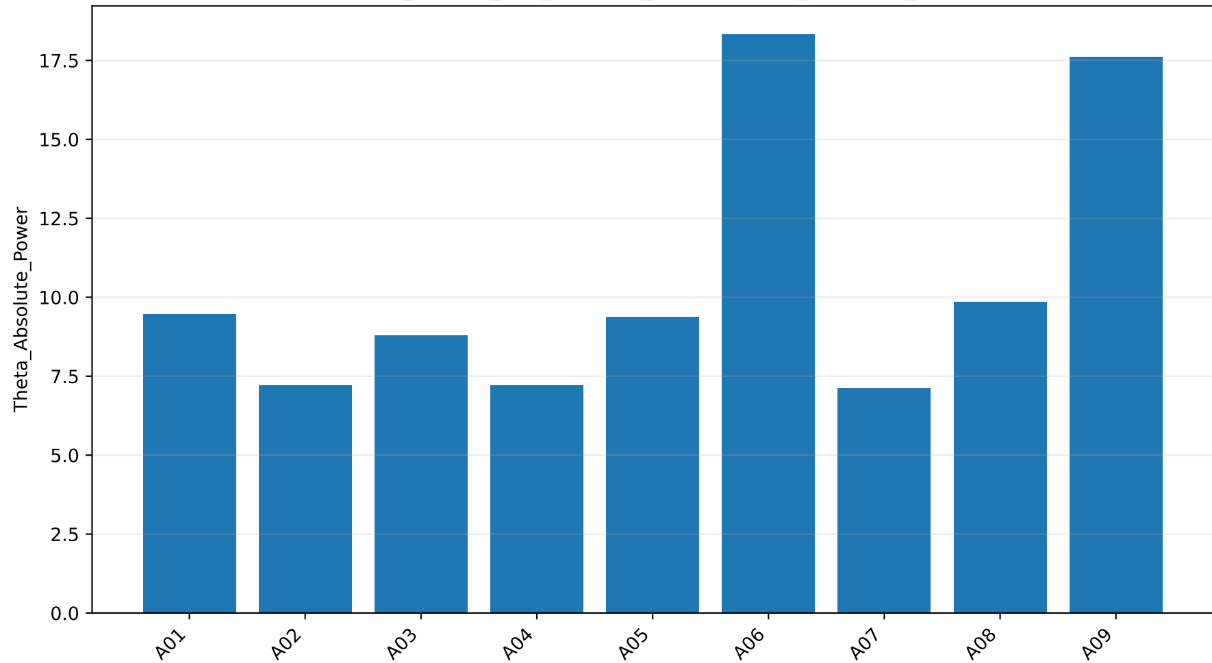
subject_central_eeg_spectral_profile: Theta_Absolute_Power
