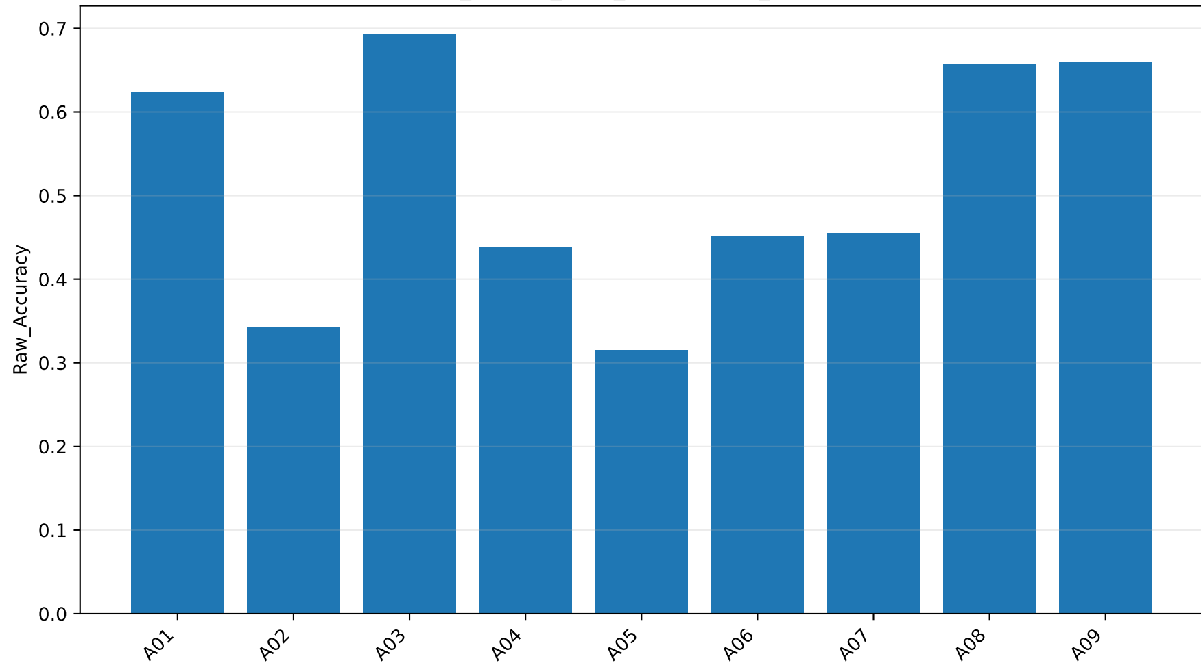
final_subject_level_results: Raw_Accuracy
