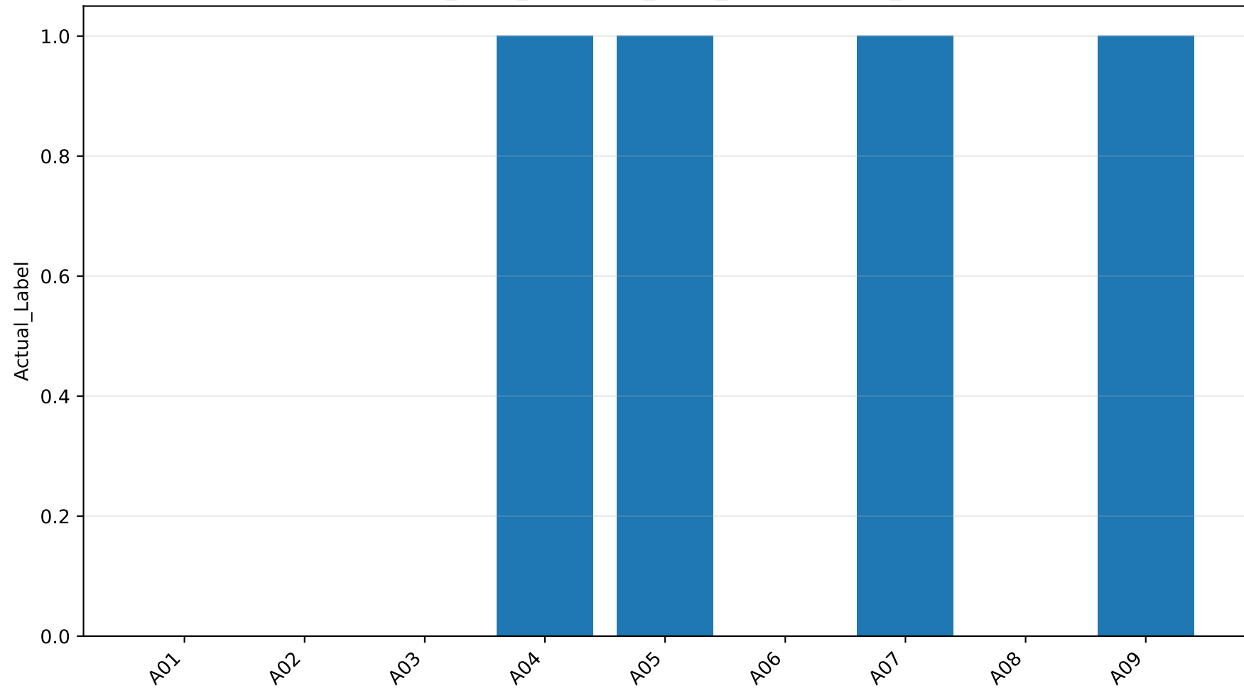
nested_loocv_responder_score_results: Actual_Label
