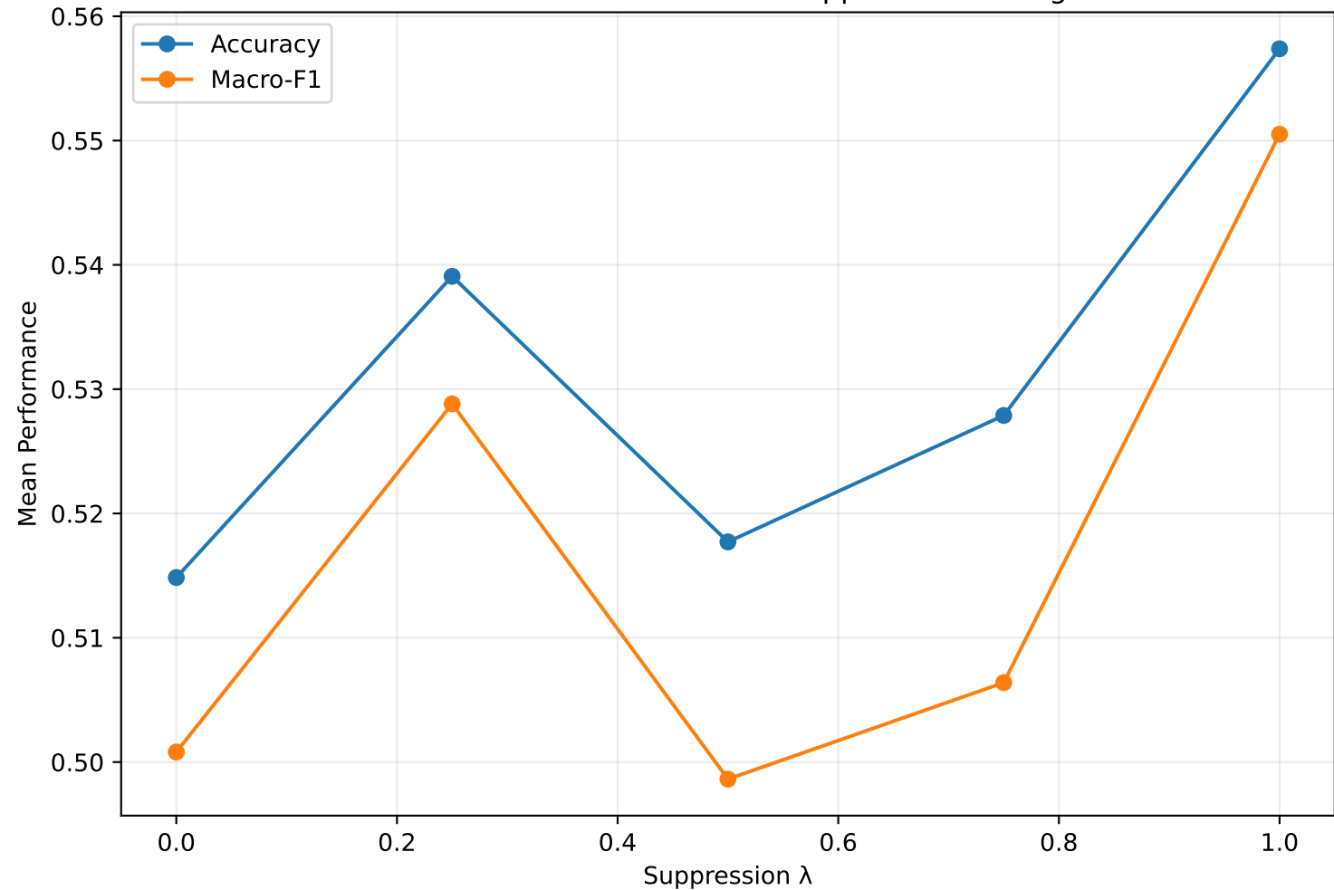
EEGNet Performance vs EOG Suppression Strength
