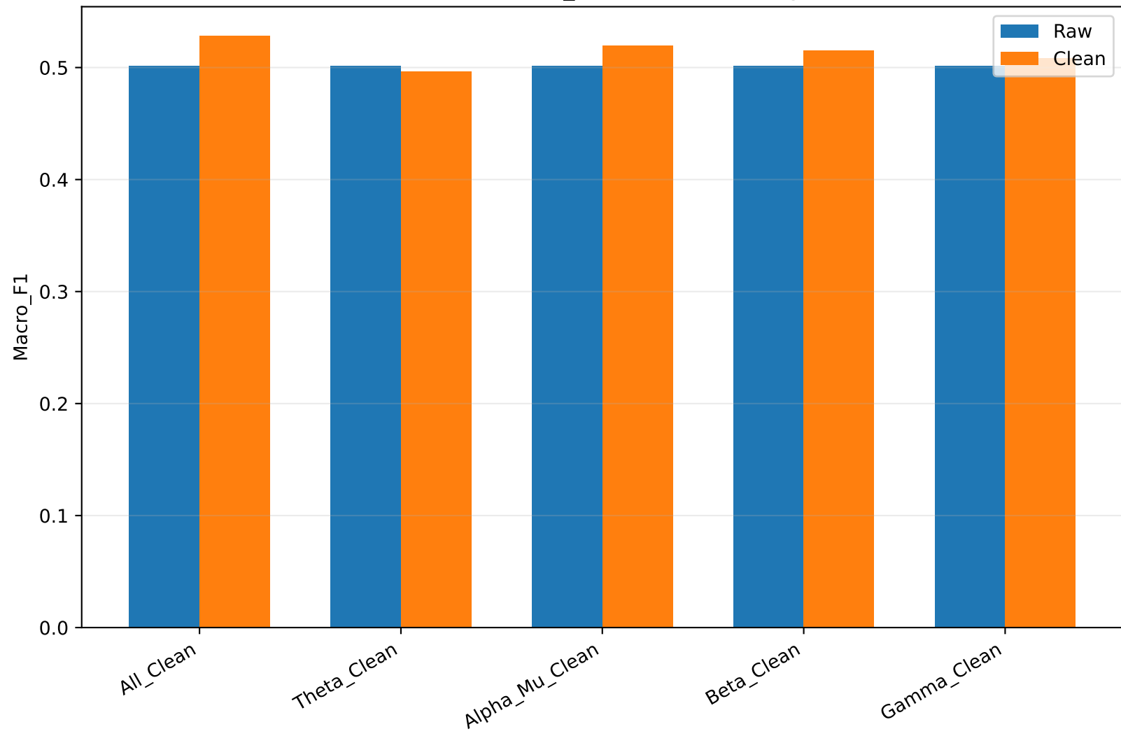
EEGNet Macro_F1: Raw vs Cleaning
