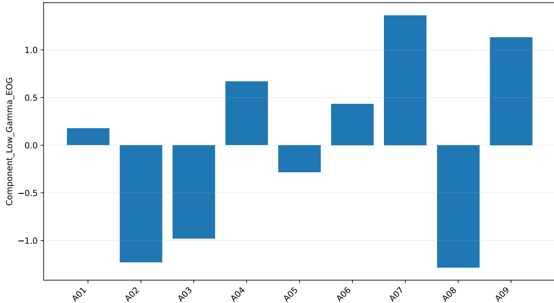
pre_cleaning_responder_score_components: Component_Low_Gamma_EOG
