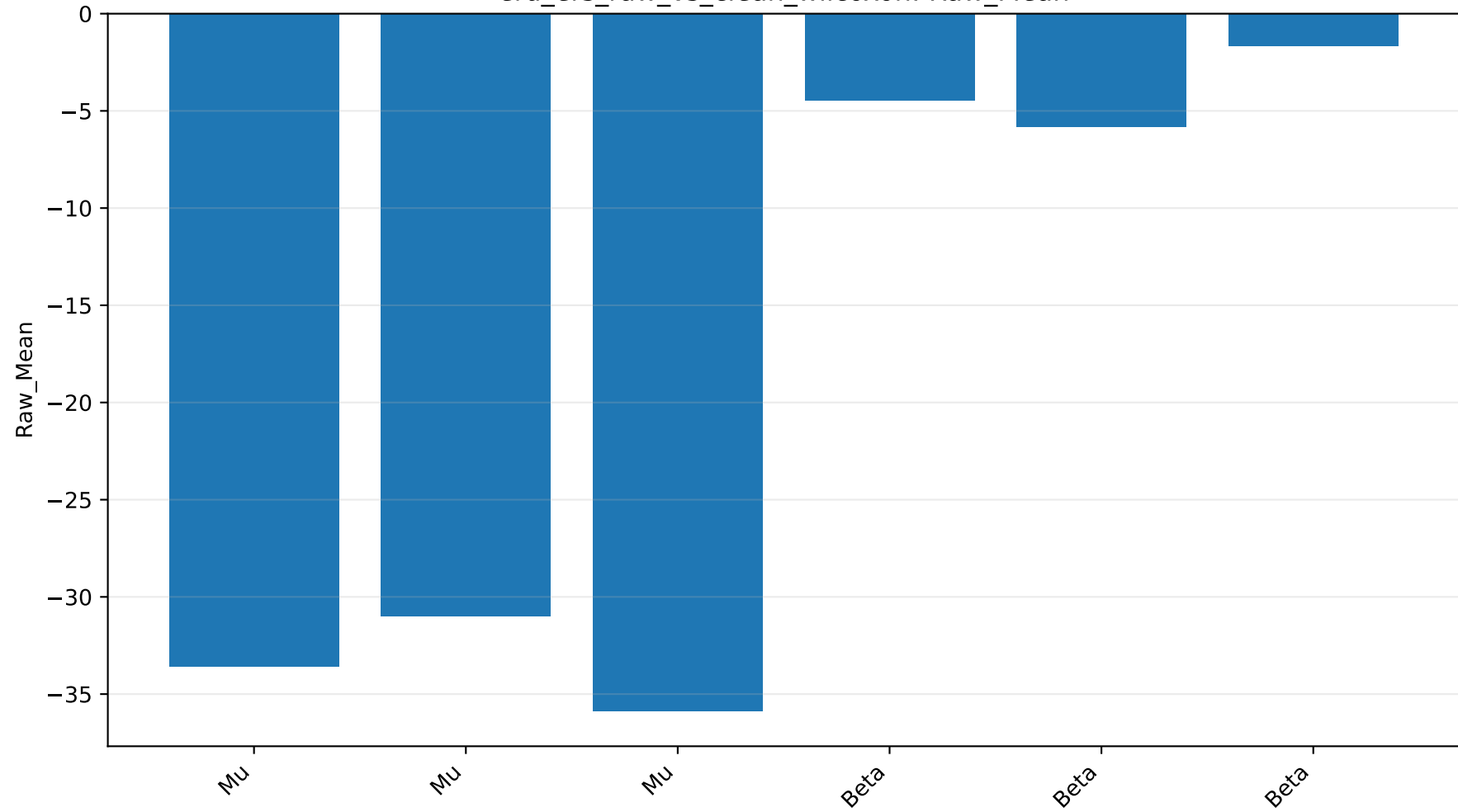
erd_ers_raw_vs_clean_wilcoxon: Raw_Mean
