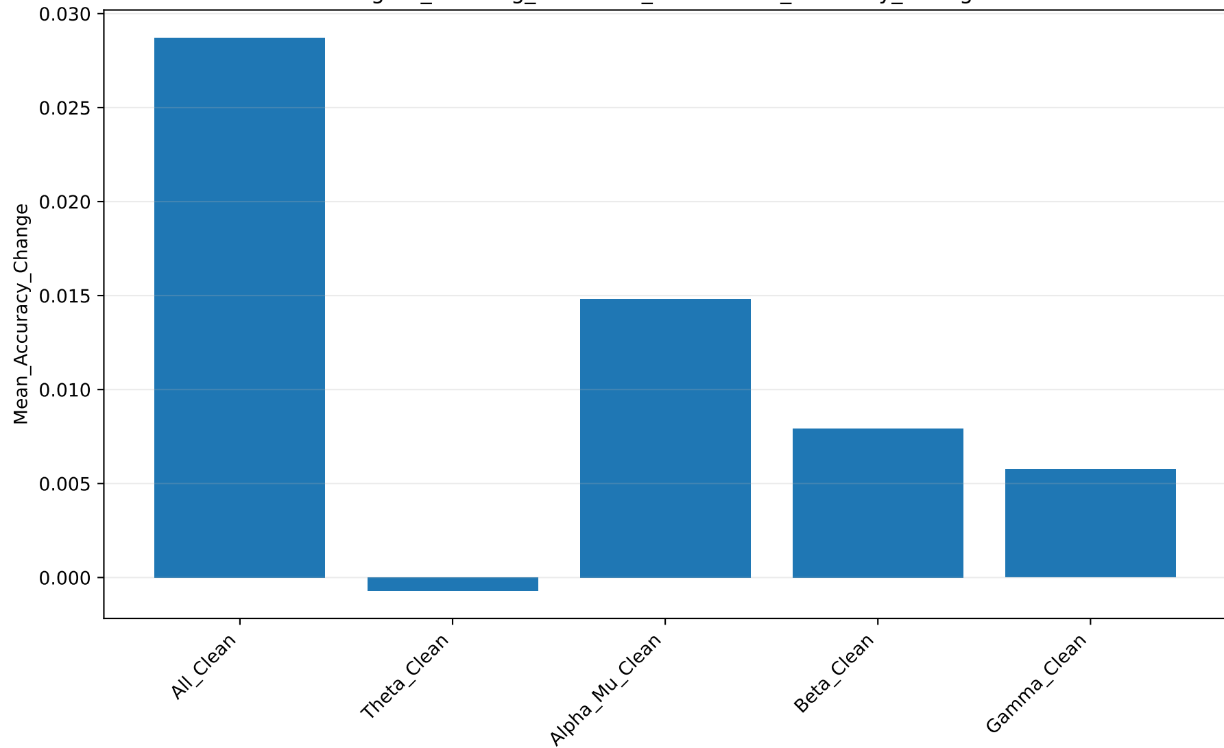
eegnet_cleaning_statistical_tests: Mean_Accuracy_Change
