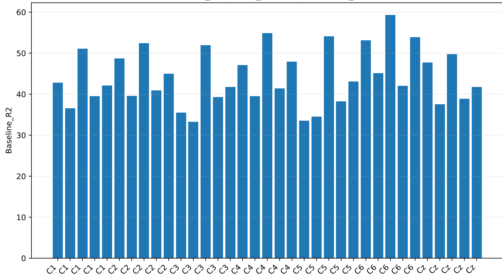
channel_frequency_summary: Baseline_R2
