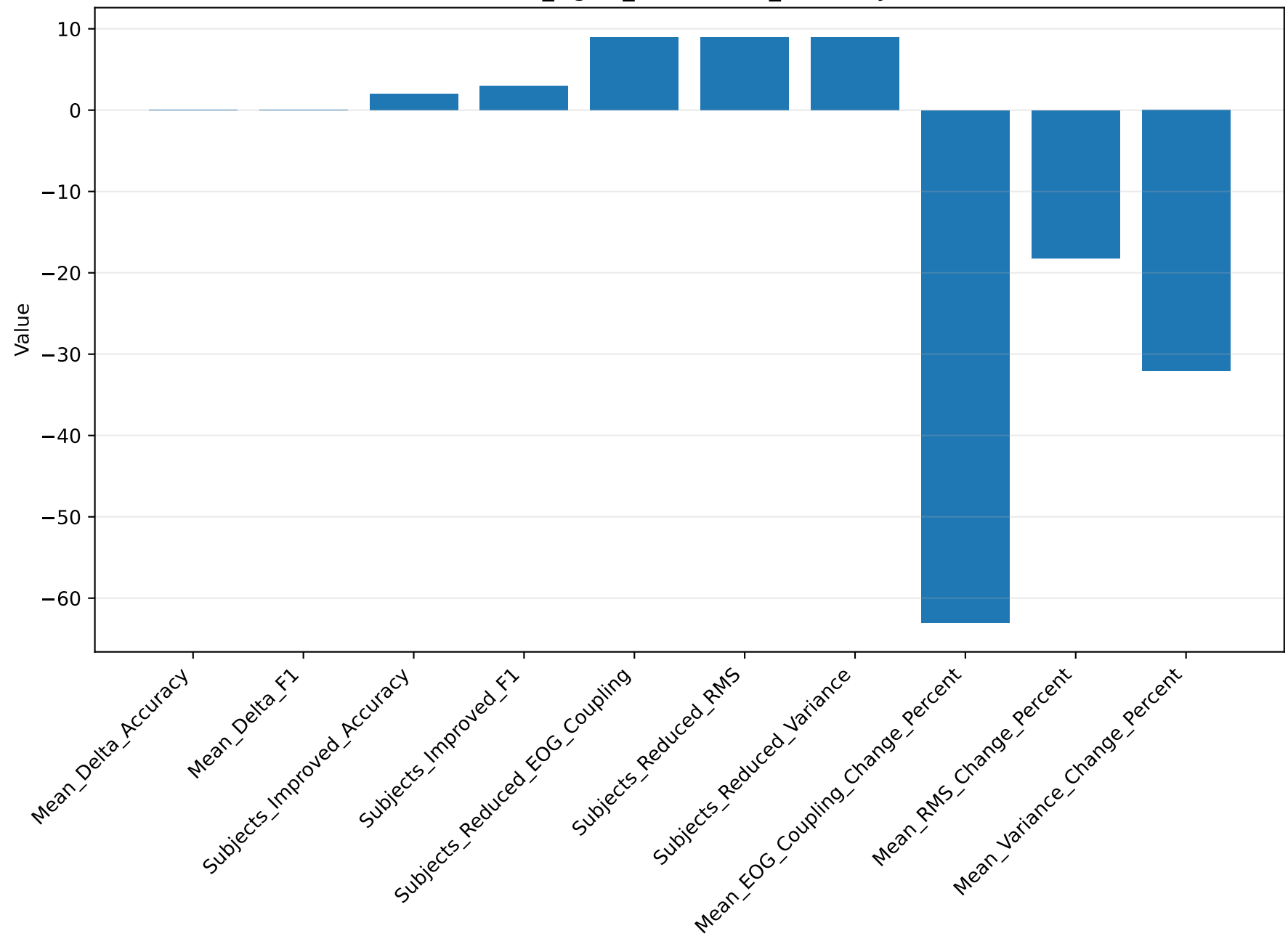
lambda075_signal_mechanism_summary: Value
