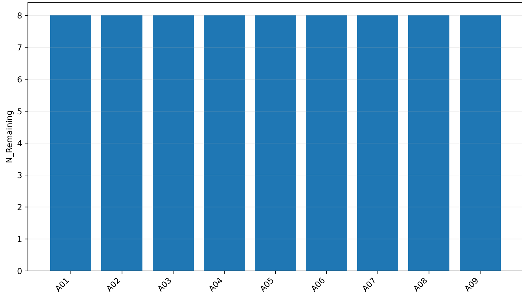
final_leave_one_subject_out: N_Remaining
