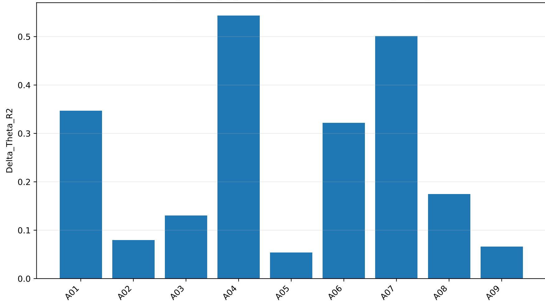
mi_eog_change_vs_optimal_lambda_master: Delta_Theta_R2
