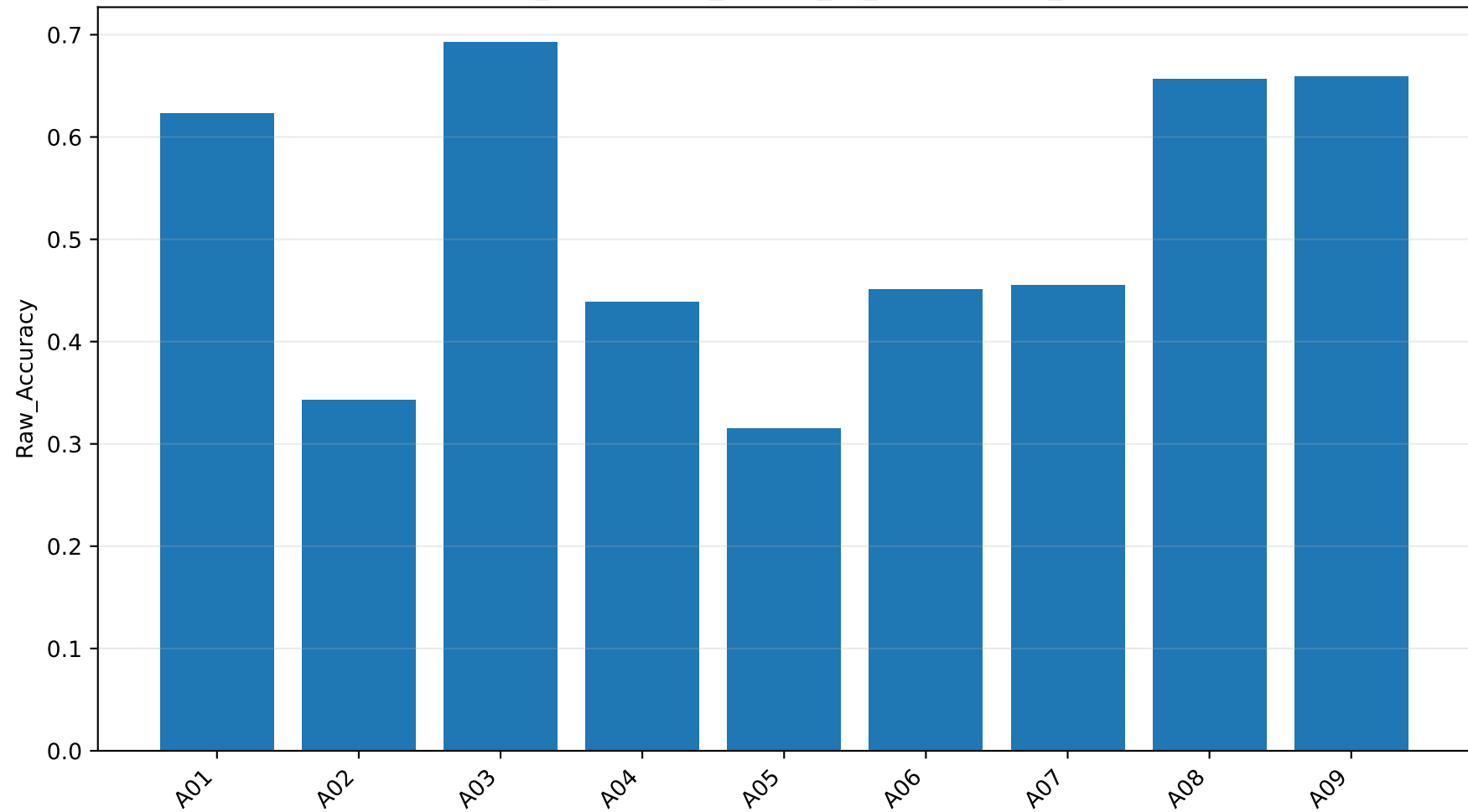
lambda075_suppression_benefit_by_subject: Raw_Accuracy
