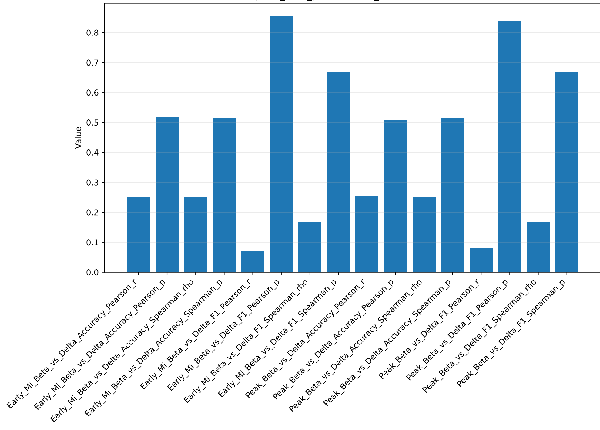
temporal_beta_performance_correlations: Value
