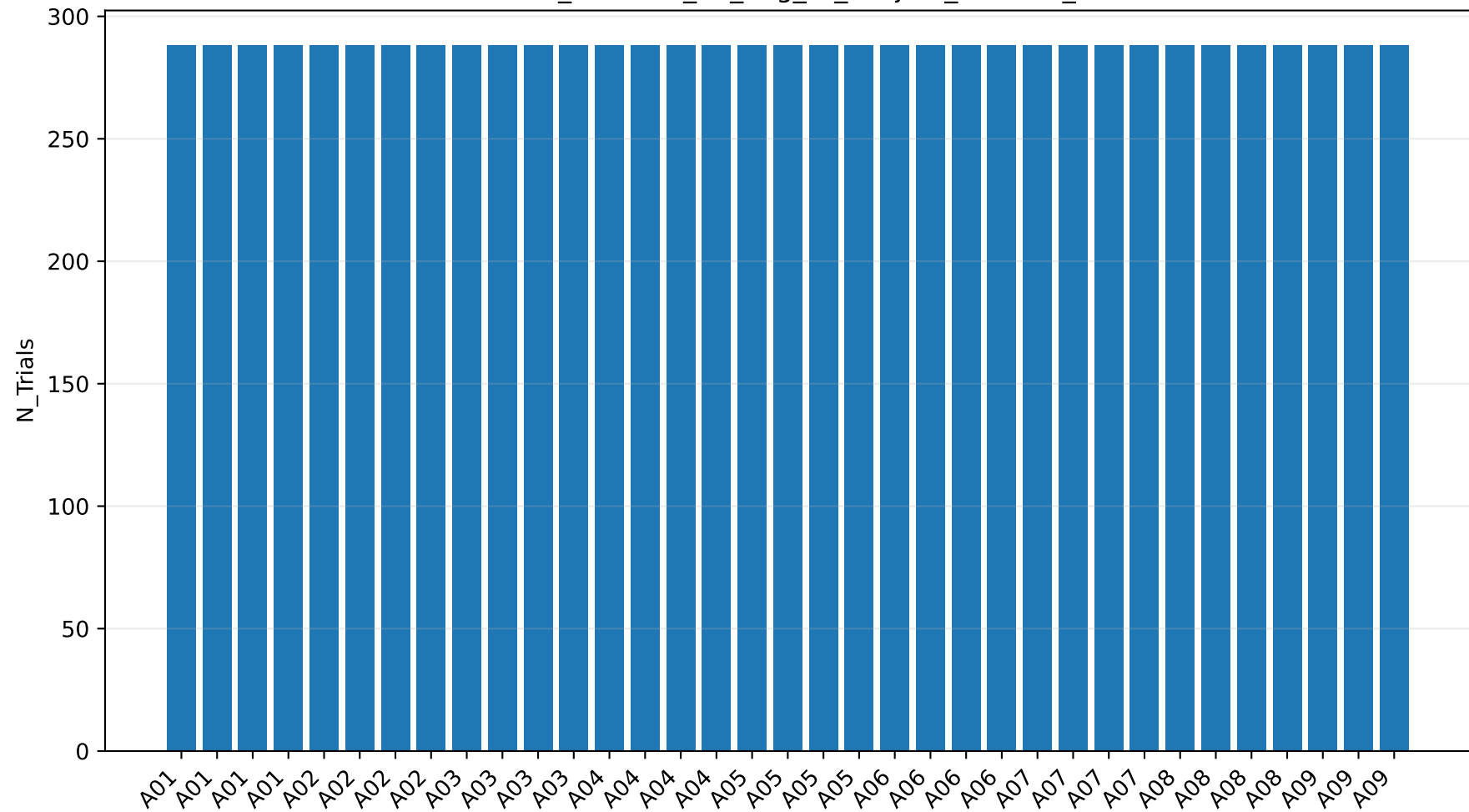
corrected_baseline_mi_eog_r2_subject_band: N_Trials
