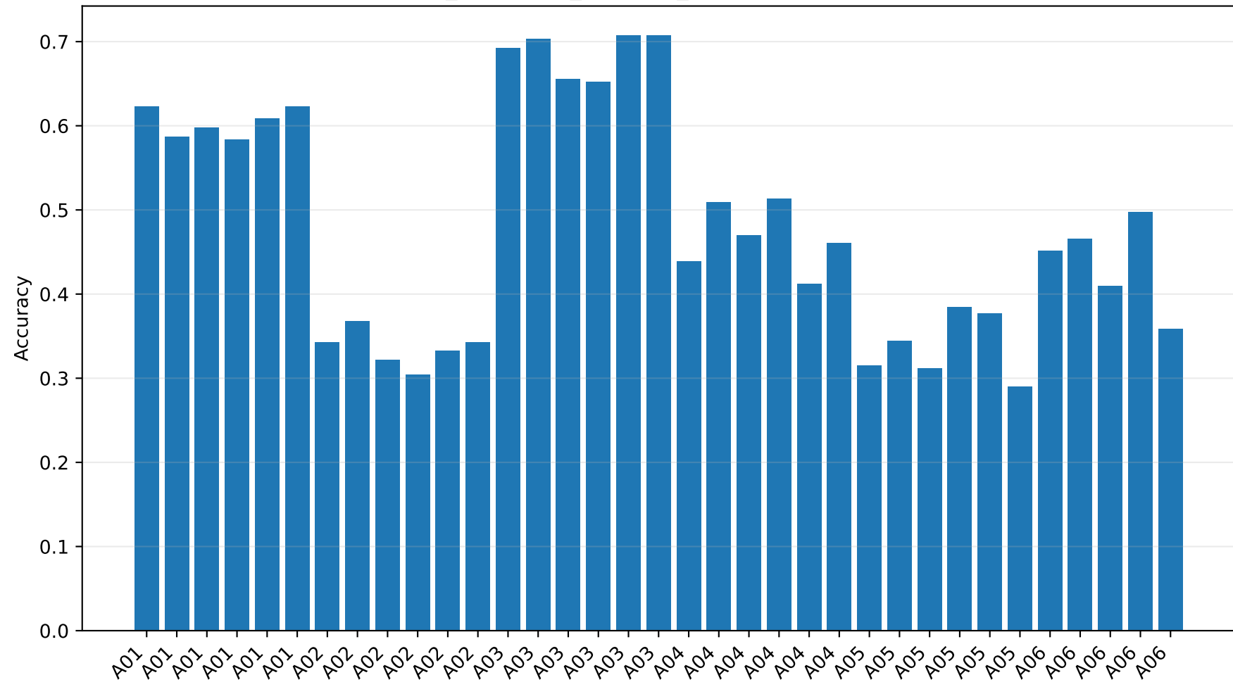
eegnet_frequency_cleaning_performance: Accuracy
