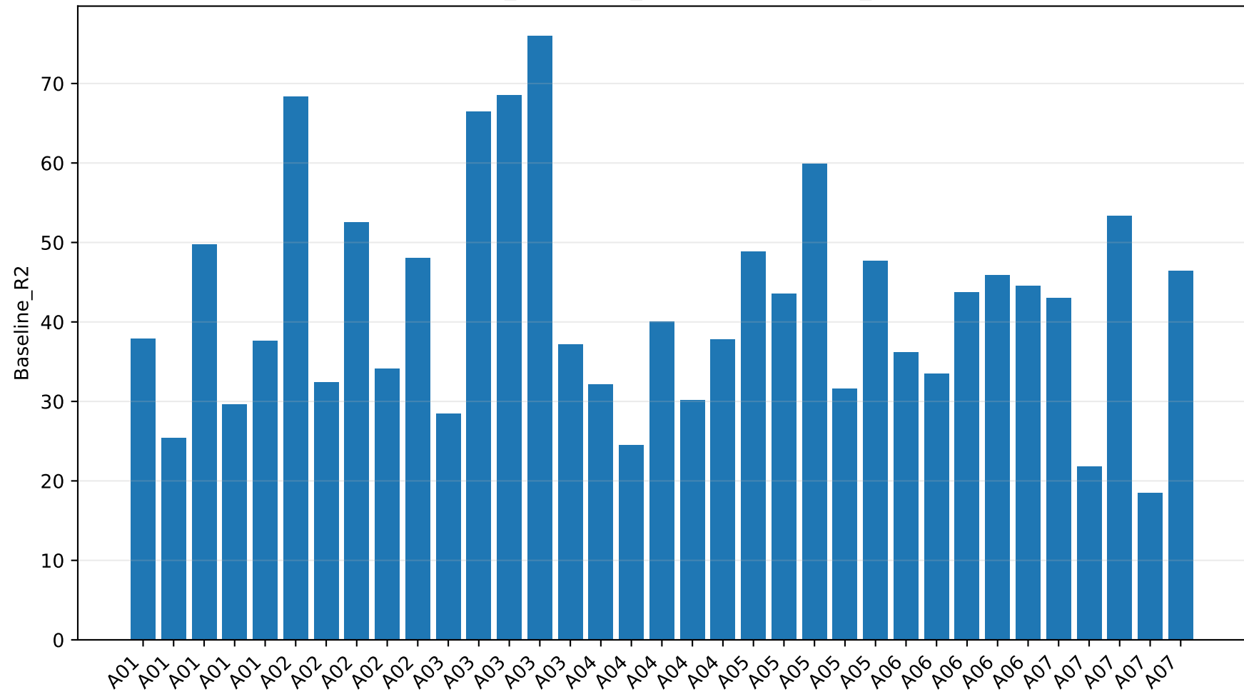
subject_frequency_summary: Baseline_R2
