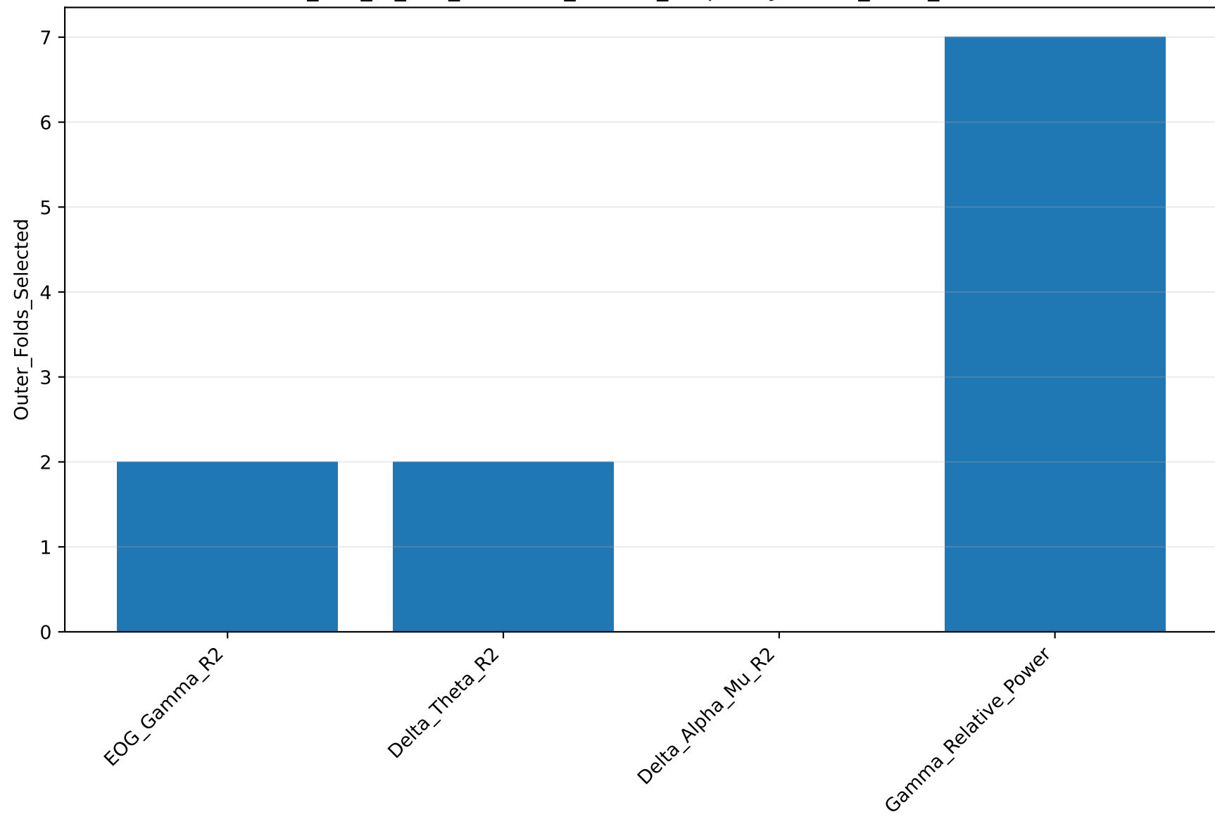
exact_end_to_end_observed_feature_frequency: Outer_Folds_Selected
