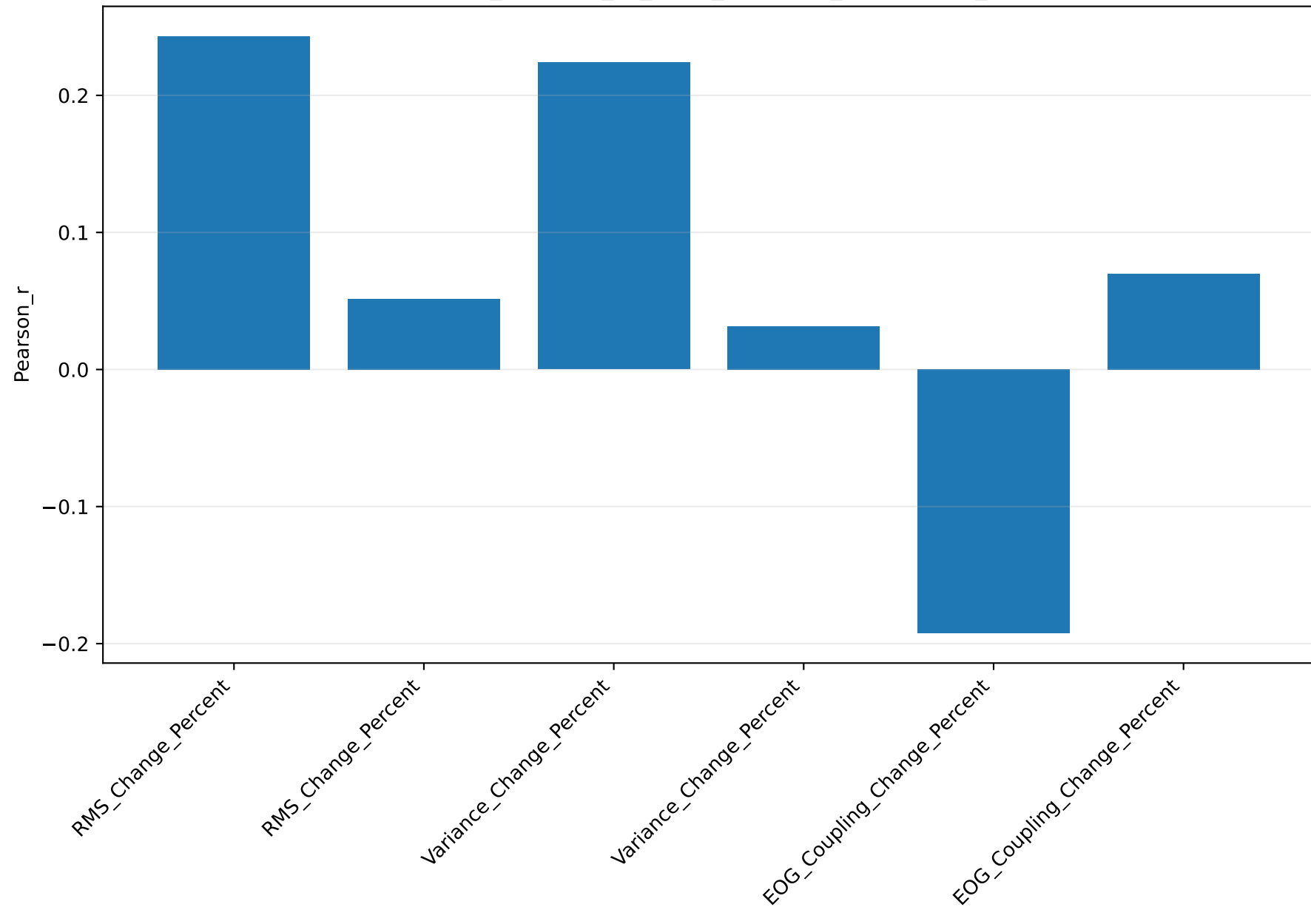
signal_changes_vs_delta_accuracy_f1: Pearson_r
