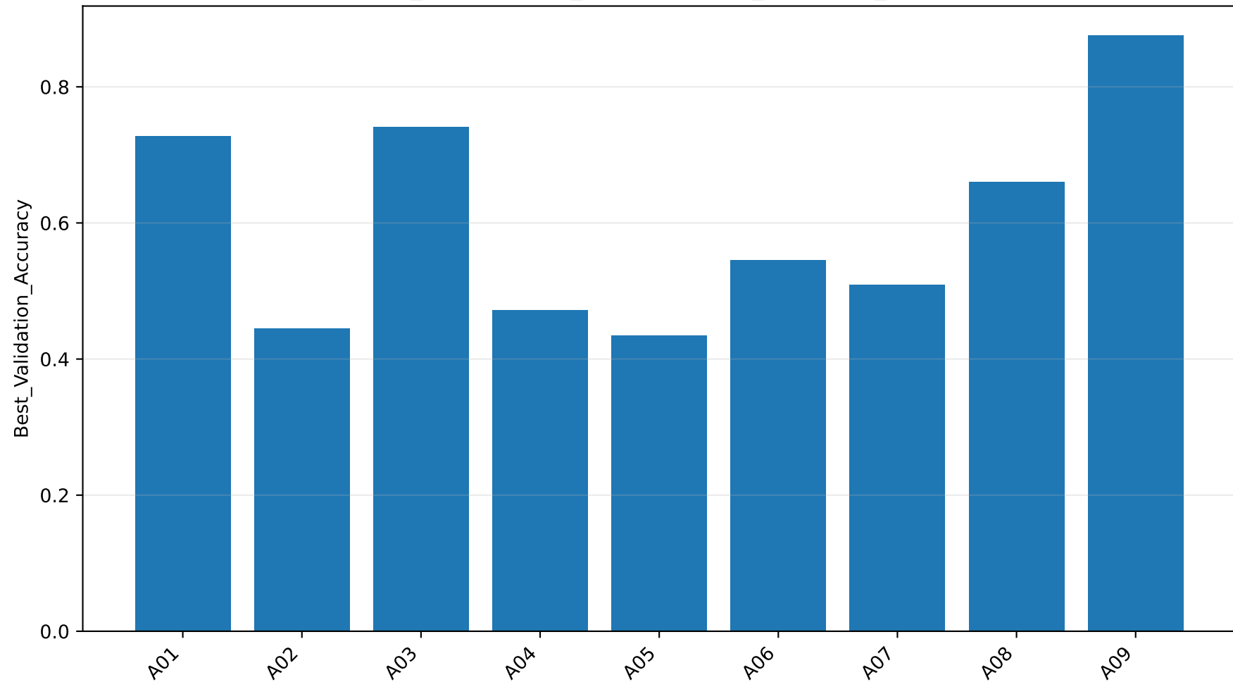
subject_compactness_summary: Best_Validation_Accuracy
