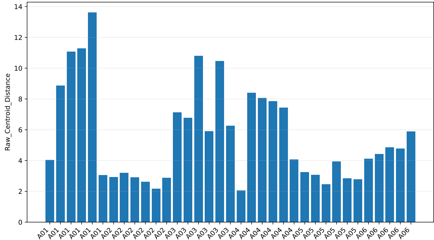
pairwise_feature_space_distances: Raw_Centroid_Distance
