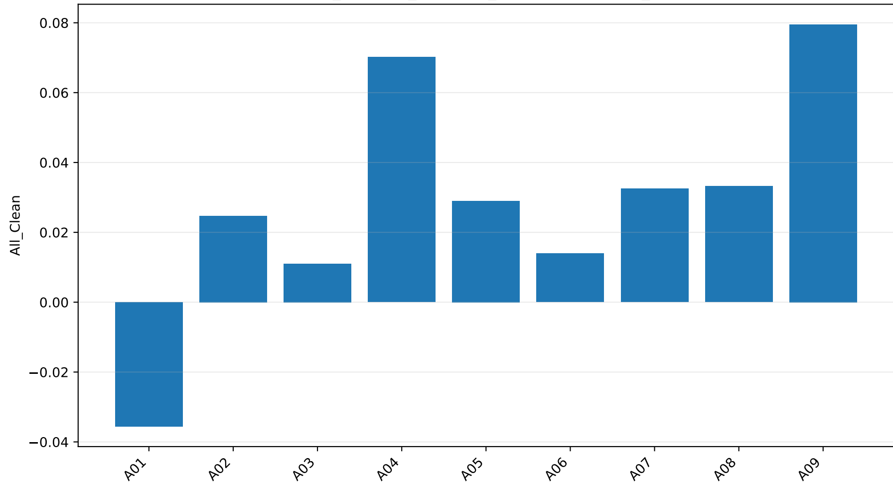
eegnet_cleaning_accuracy_improvements: All_Clean
