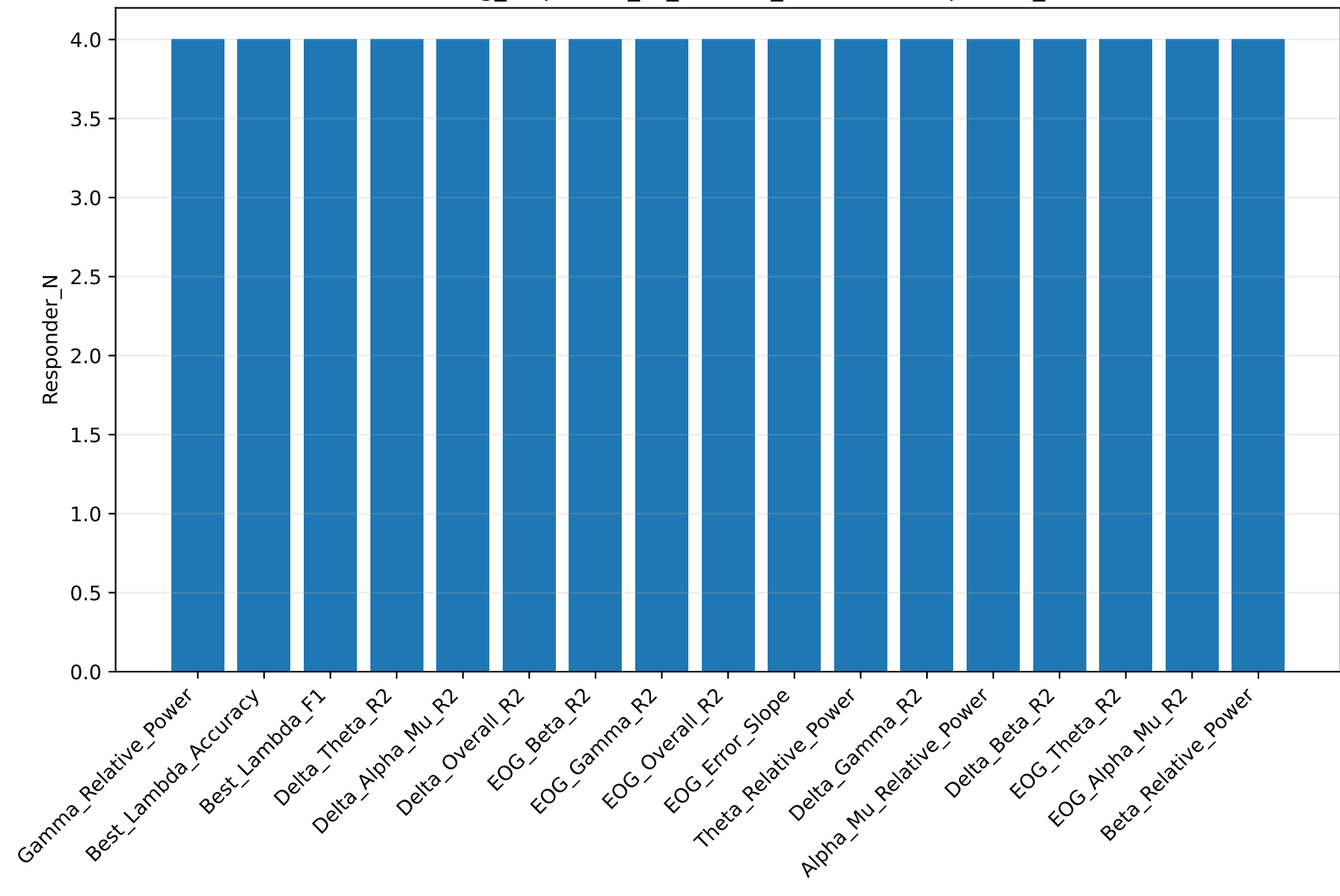
cleaning_responder_vs_harmed_statistics: Responder_N
