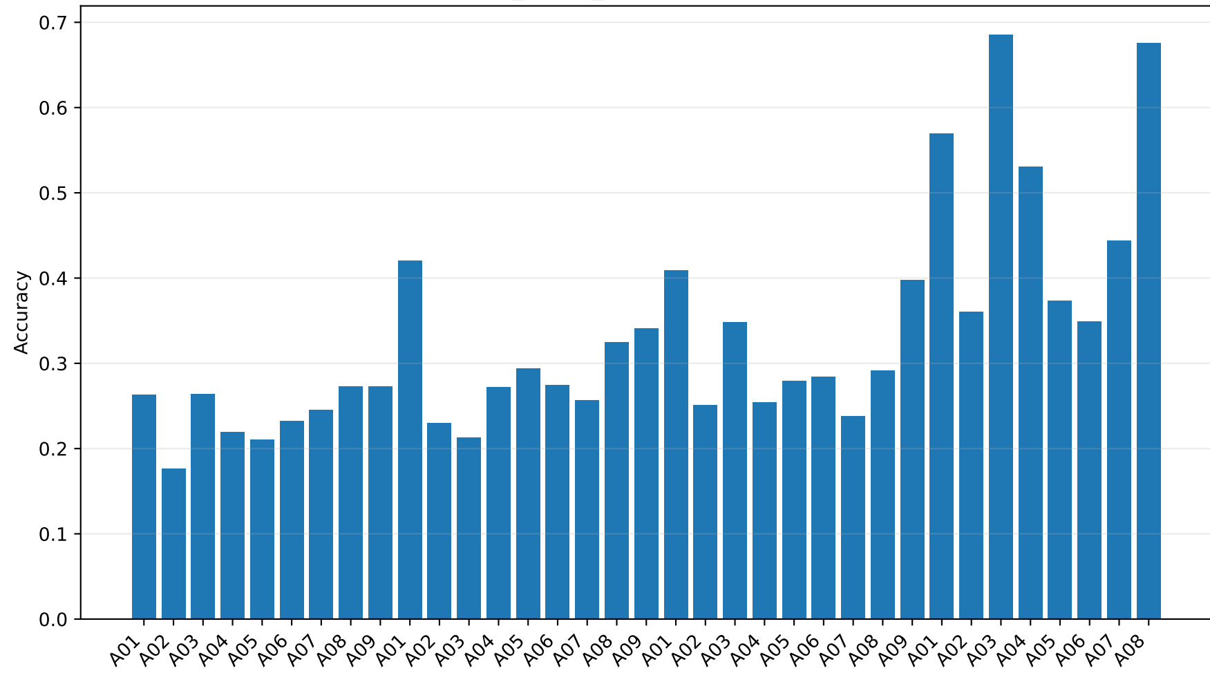
subject_model_performance: Accuracy
