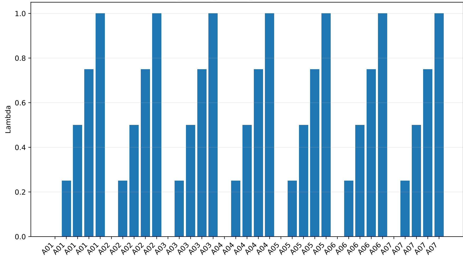
eegnet_allband_lambda_performance: Lambda
