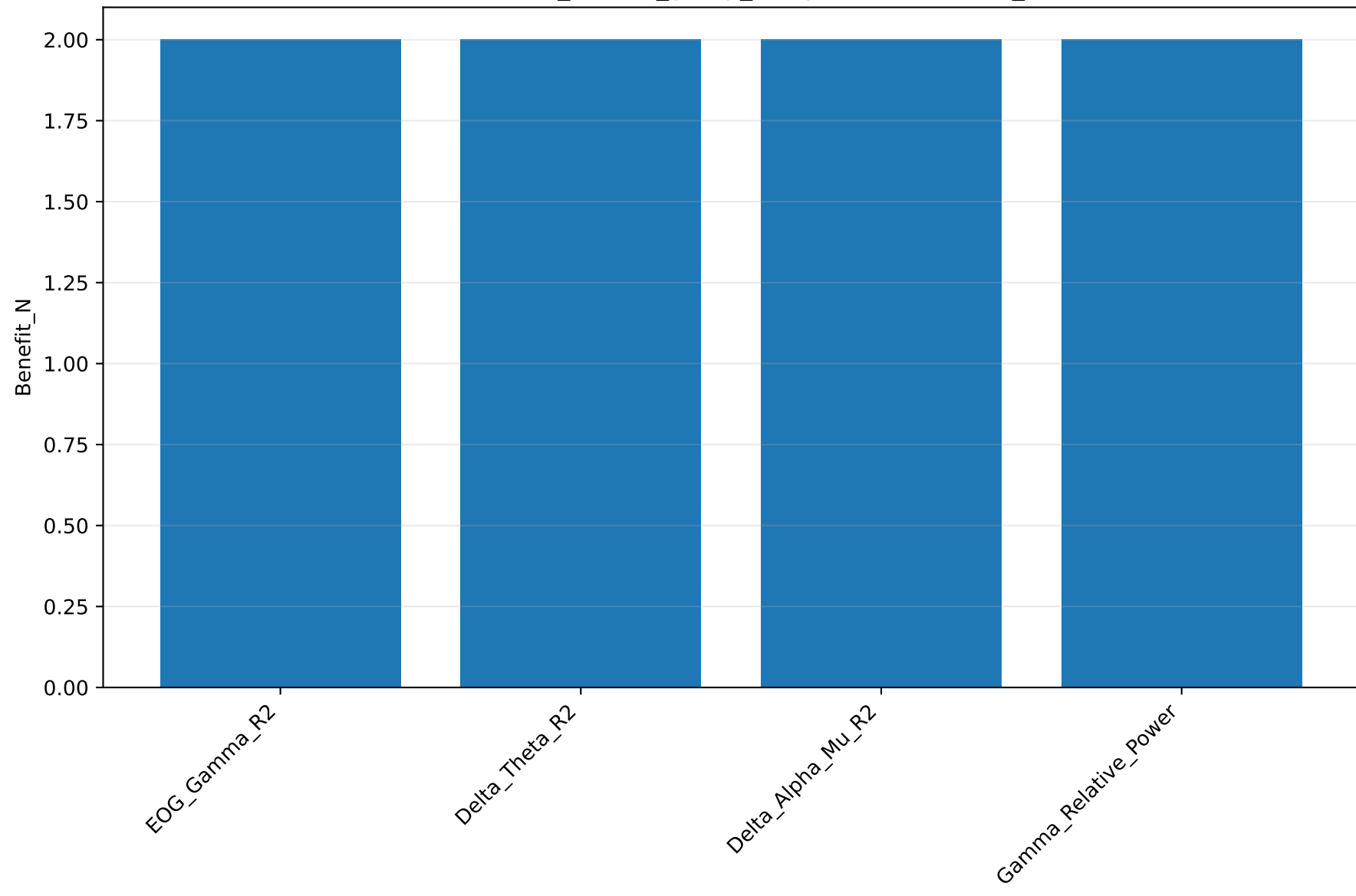
lambda075_benefit_group_comparisons: Benefit_N
