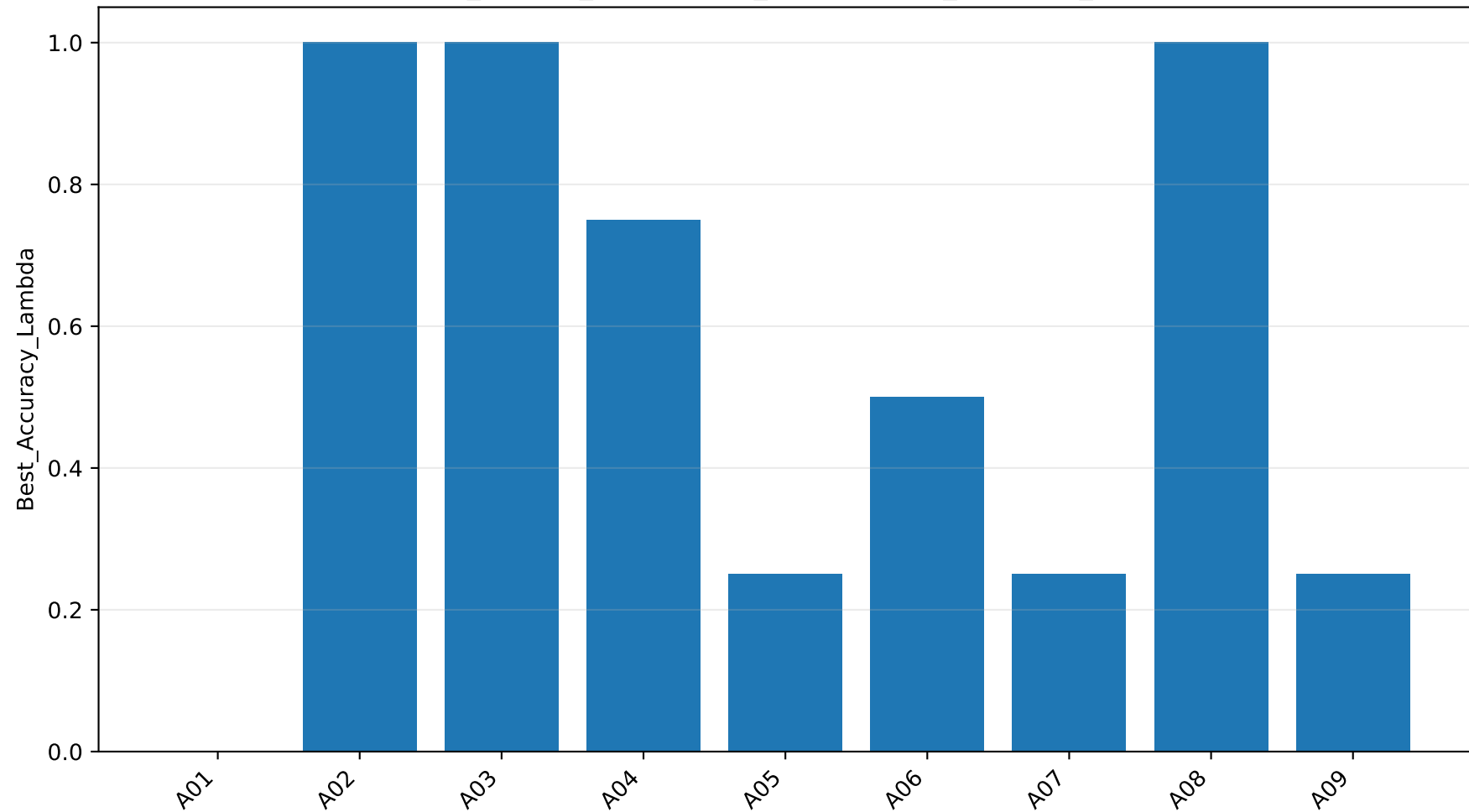
subject_allband_suppression_profiles: Best_Accuracy_Lambda
