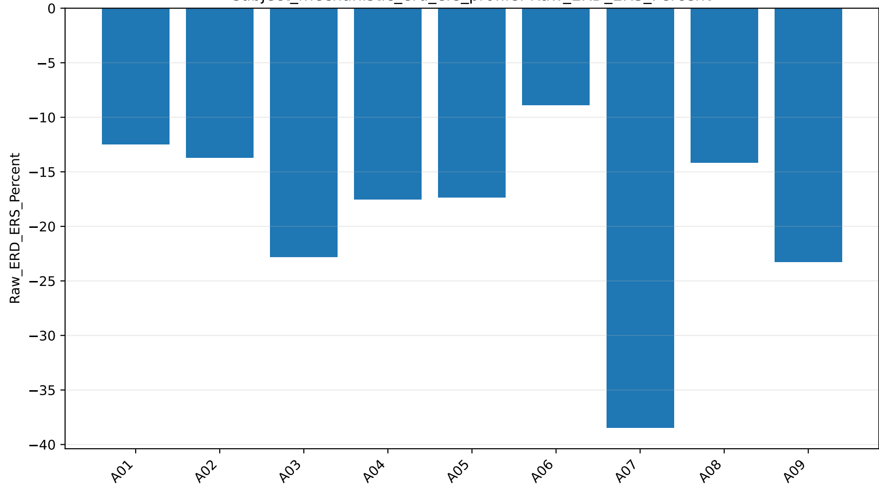
subject_mechanistic_erd_ers_profile: Raw_ERD_ERS_Percent
