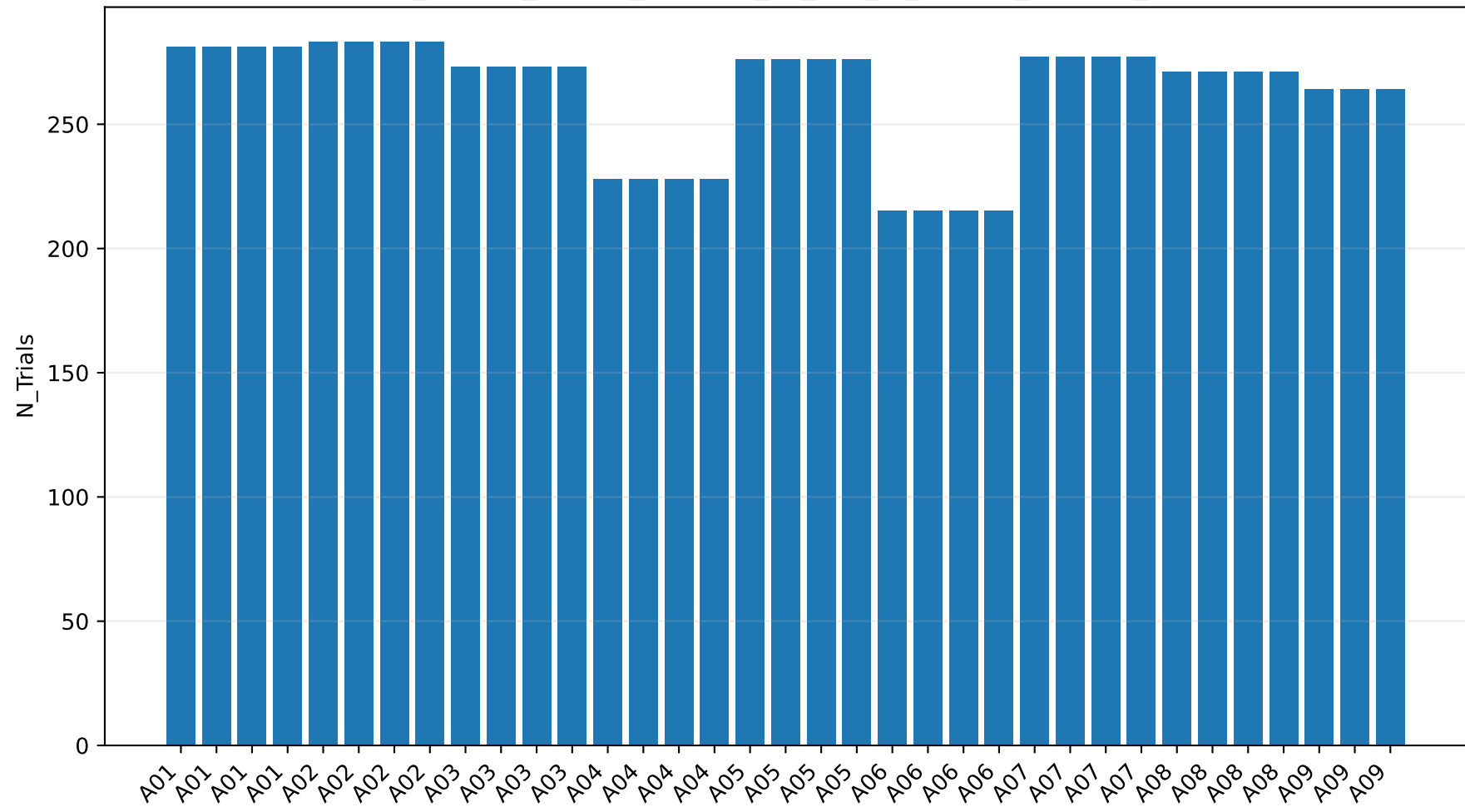
final_artifact_filtered_baseline_mi_eog_r2_subject_band: N_Trials
