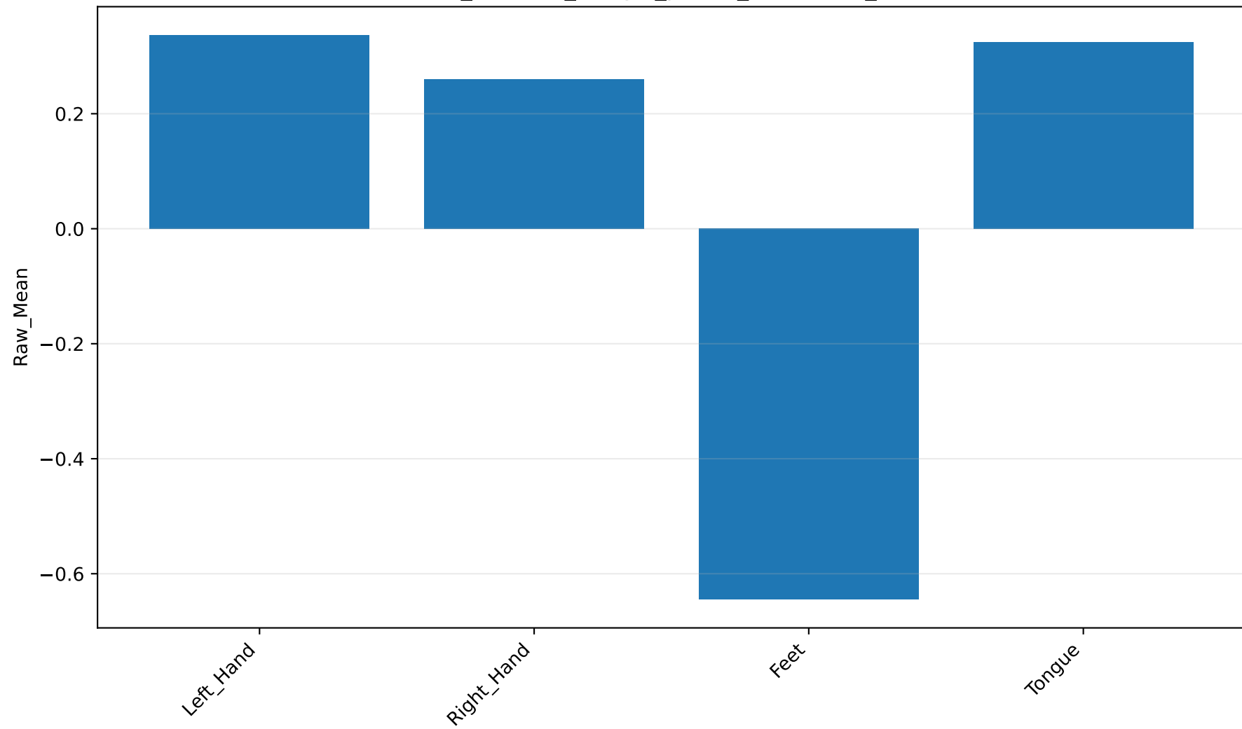
class_decision_margin_paired_tests: Raw_Mean
