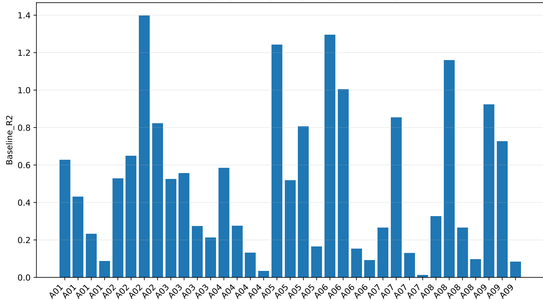
baseline_mi_subject_band_delta_r2: Baseline_R2
