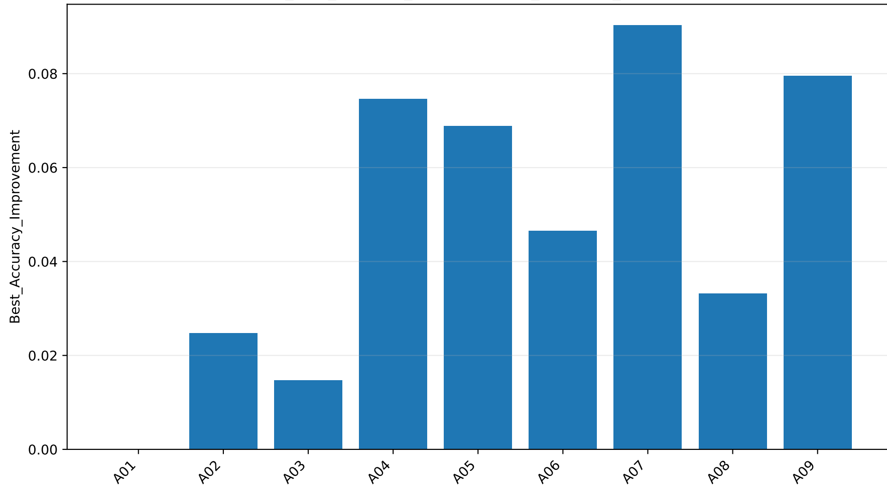
subject_best_cleaning_response: Best_Accuracy_Improvement
