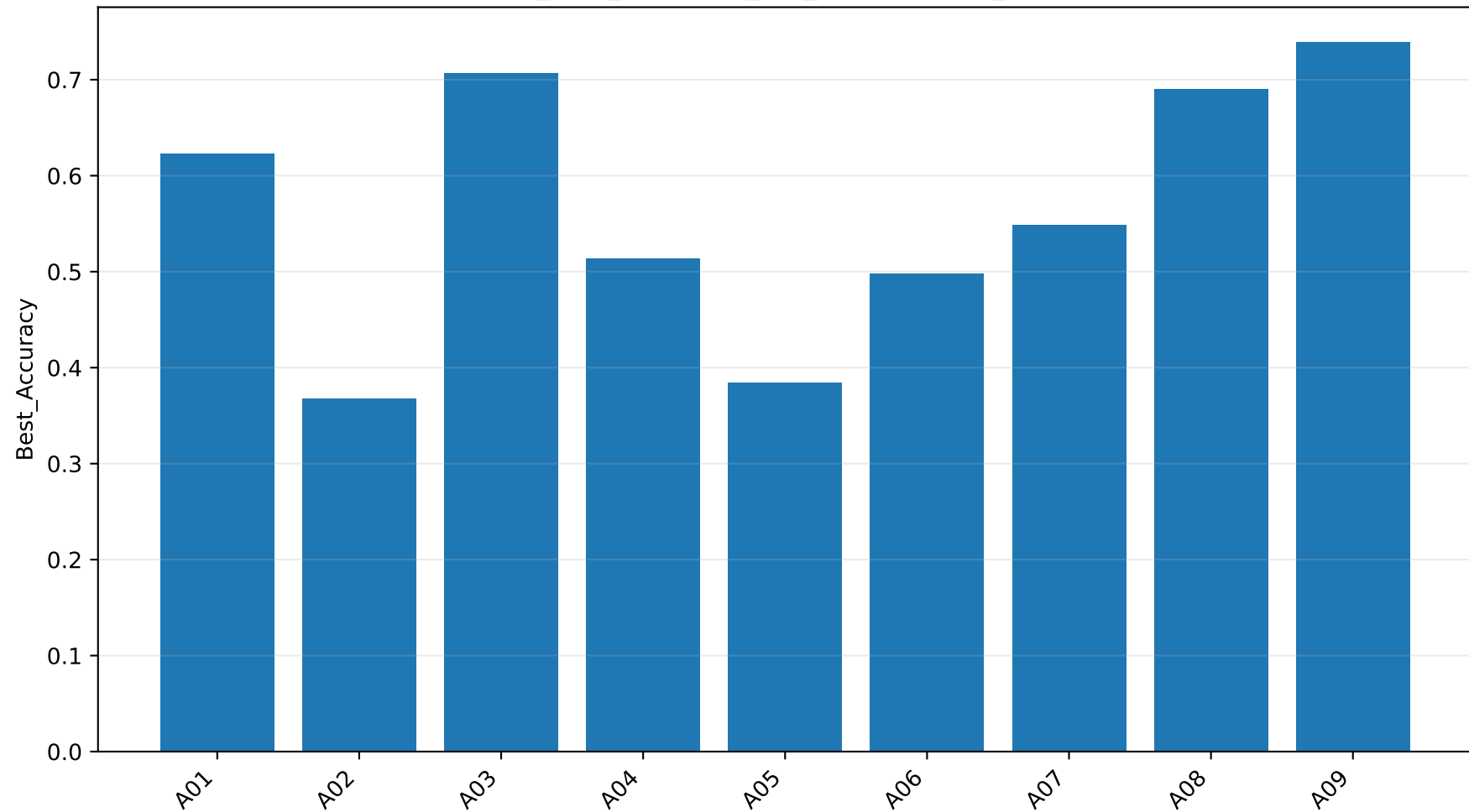
eegnet_best_condition_per_subject: Best_Accuracy
