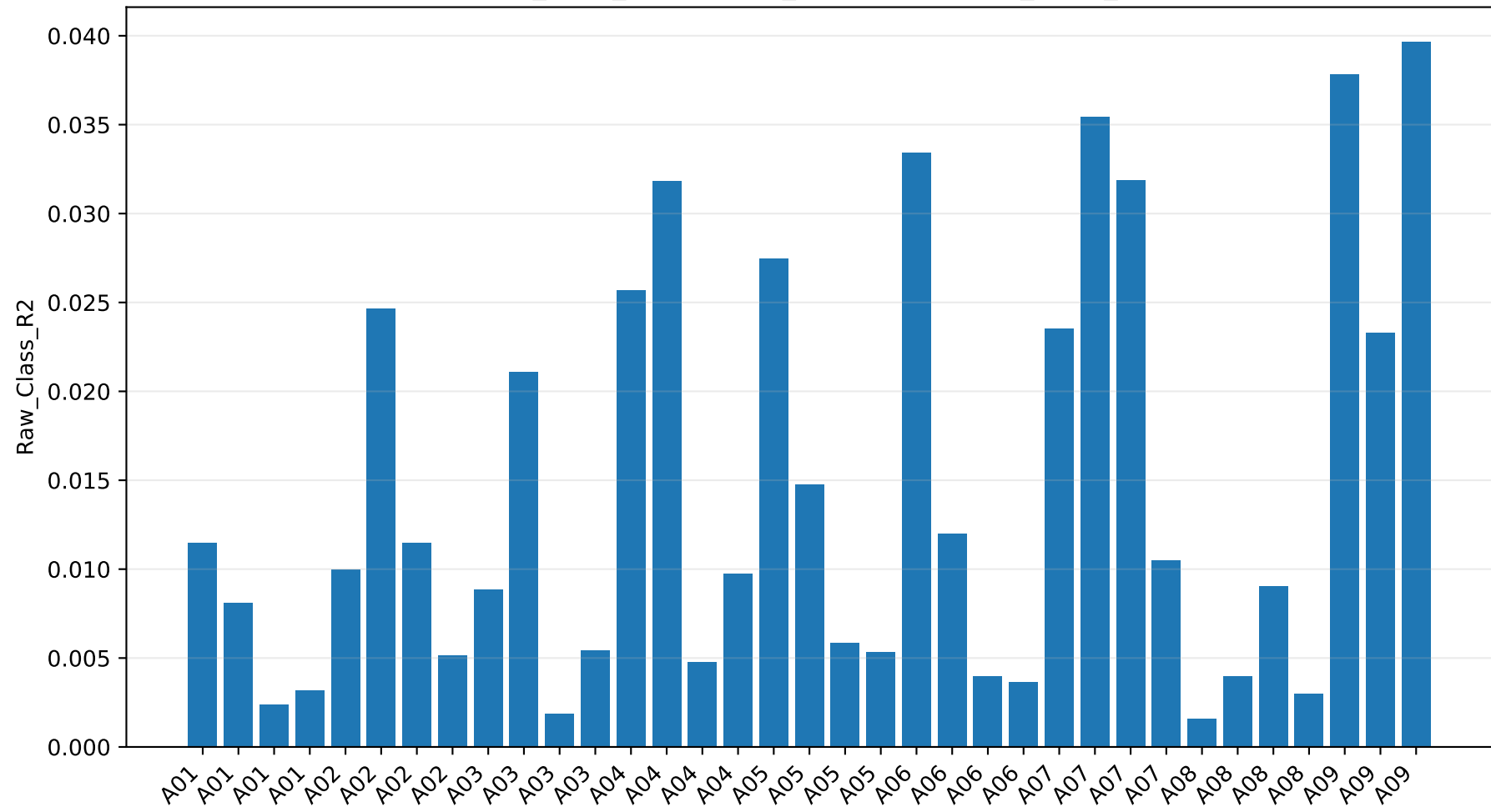
band_class_separability_lambda075: Raw_Class_R2
