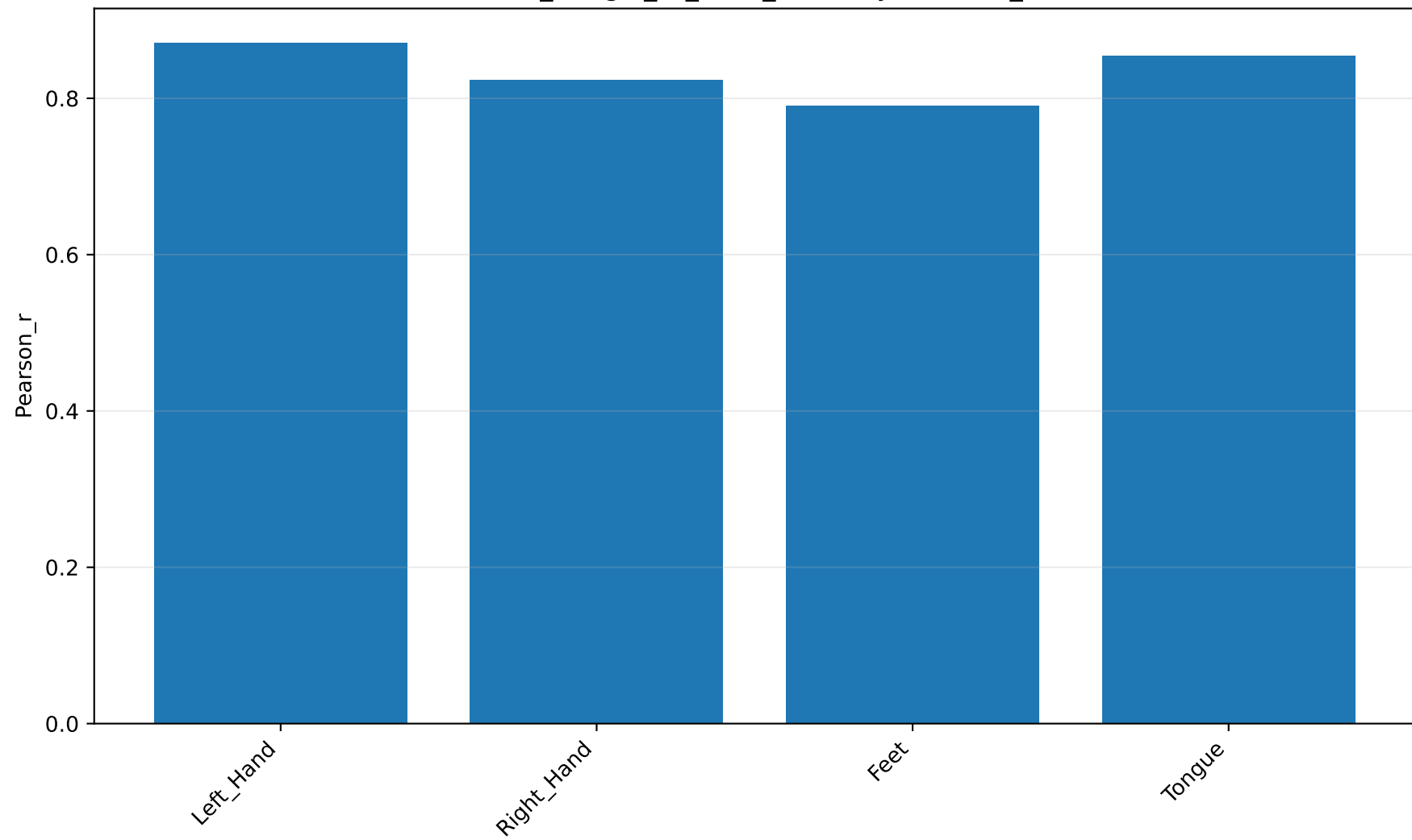
class_margin_vs_class_accuracy: Pearson_r
