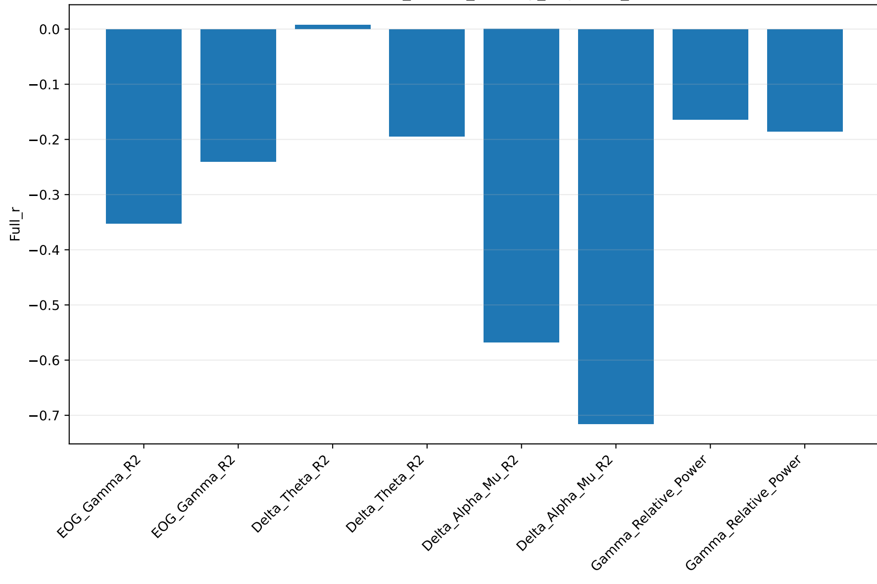
lambda075_benefit_stability_flags: Full_r
