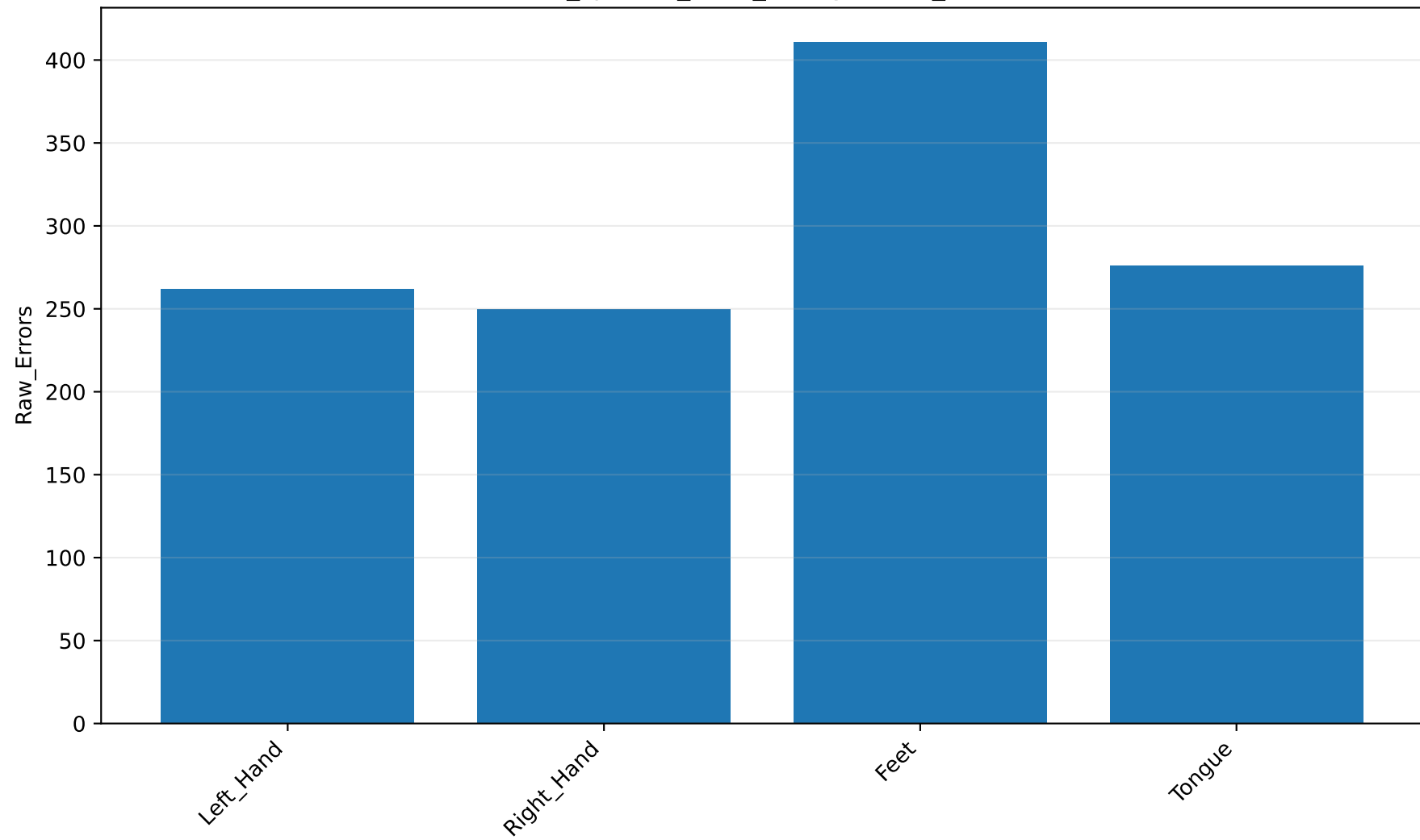
class_specific_error_change: Raw_Errors
