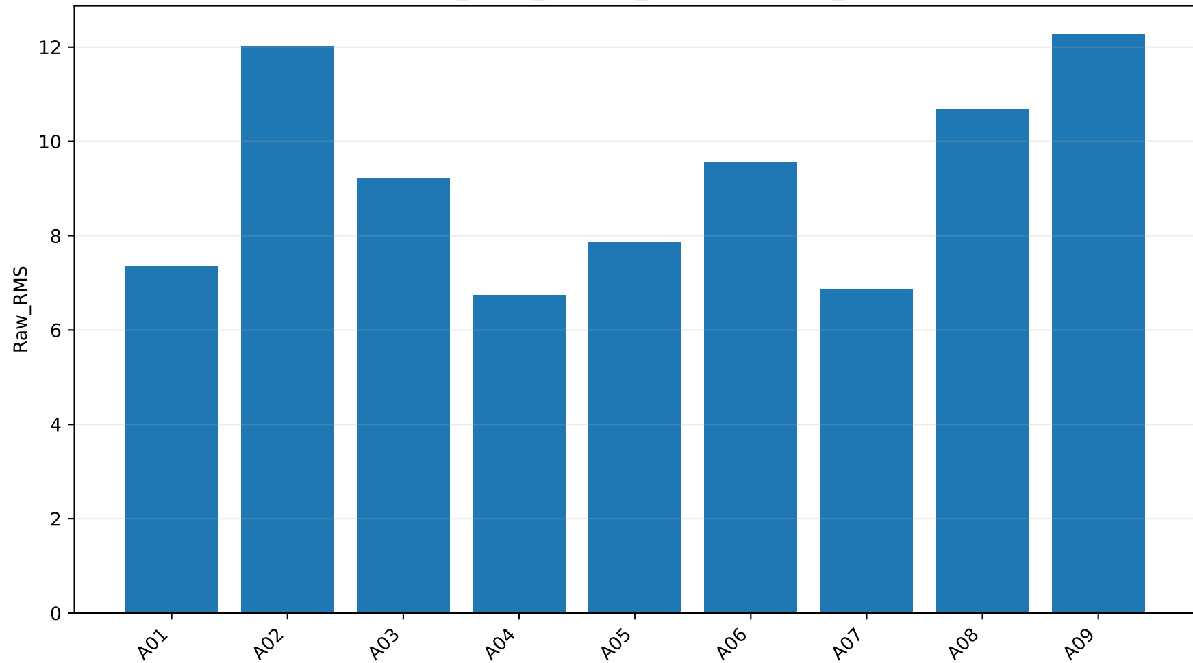
subject_signal_changes_lambda075: Raw_RMS
