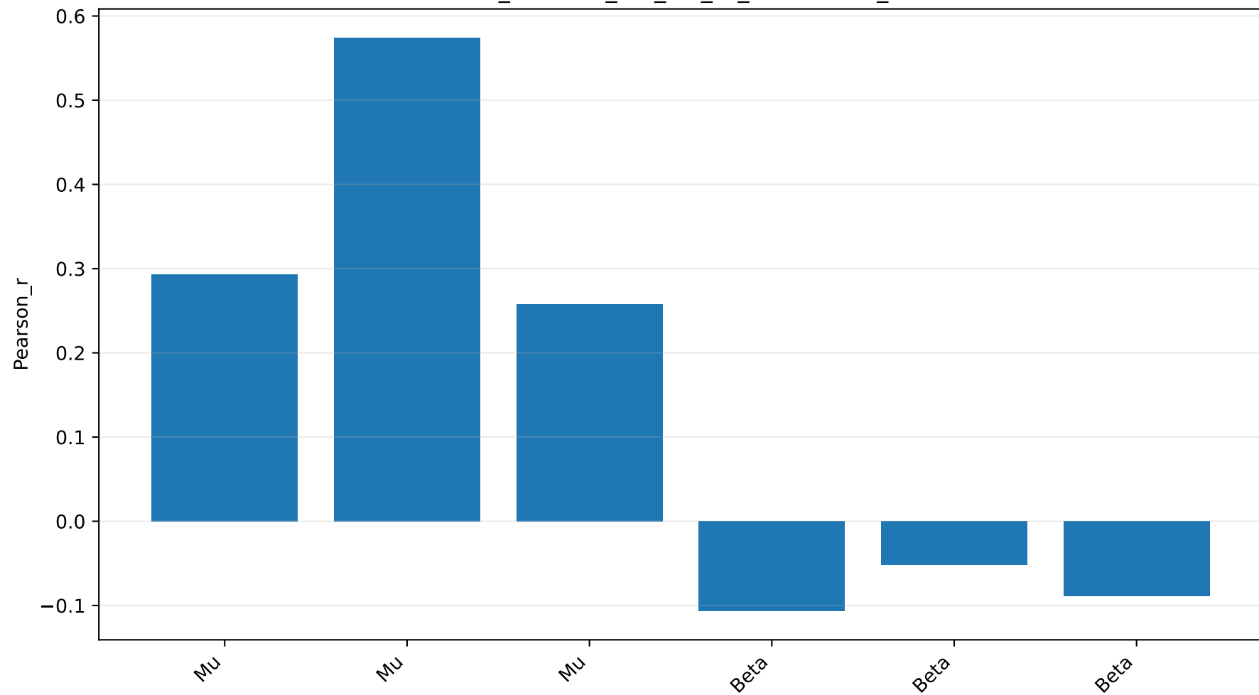
full_duration_erd_ers_vs_f1: Pearson_r
