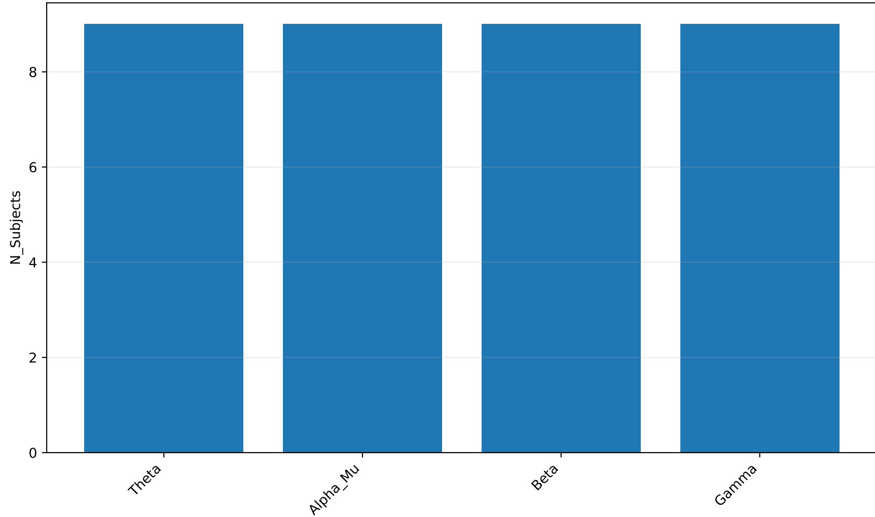
eog_error_slope_spectral_correlations: N_Subjects
