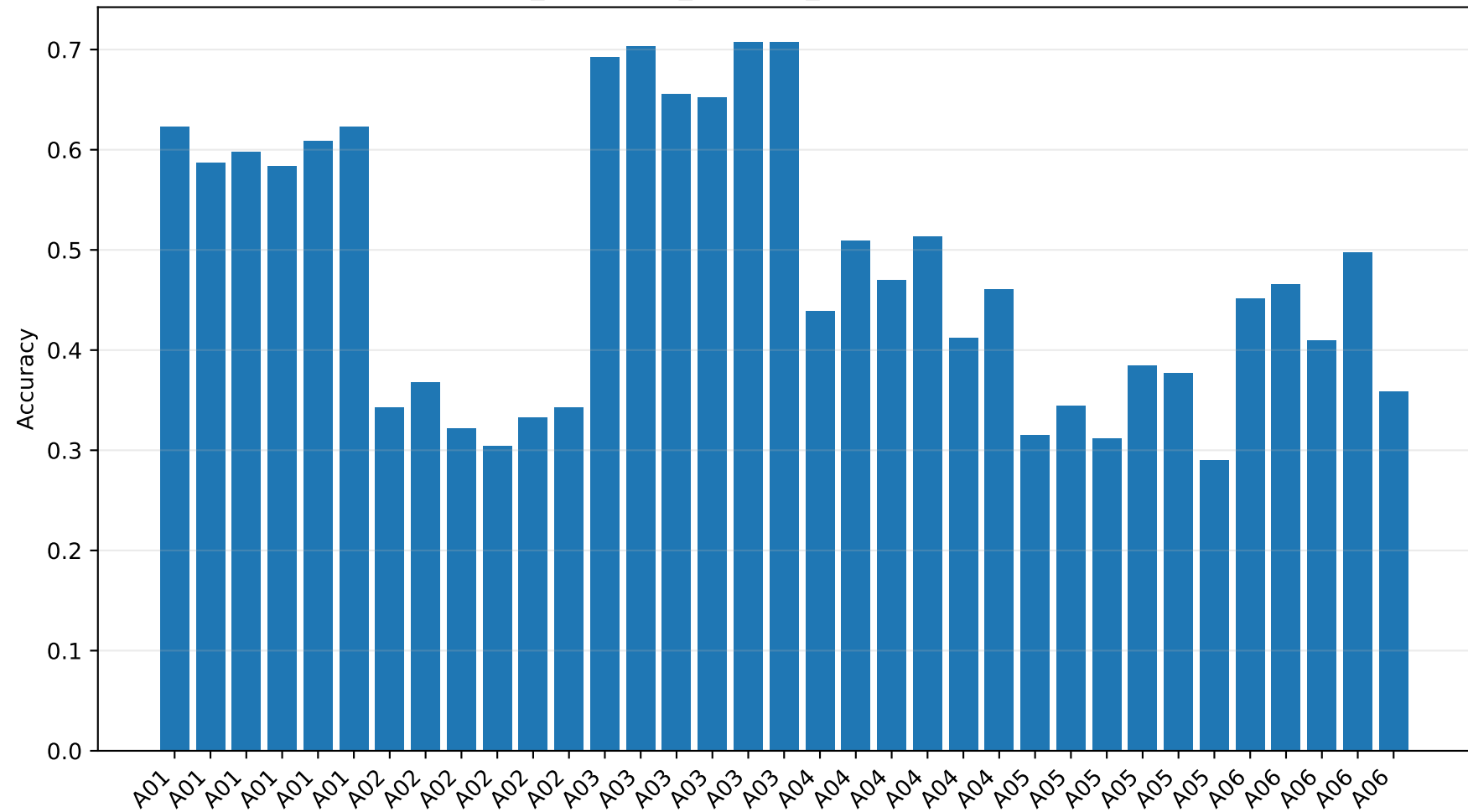
eegnet_frequency_cleaning_performance: Accuracy
