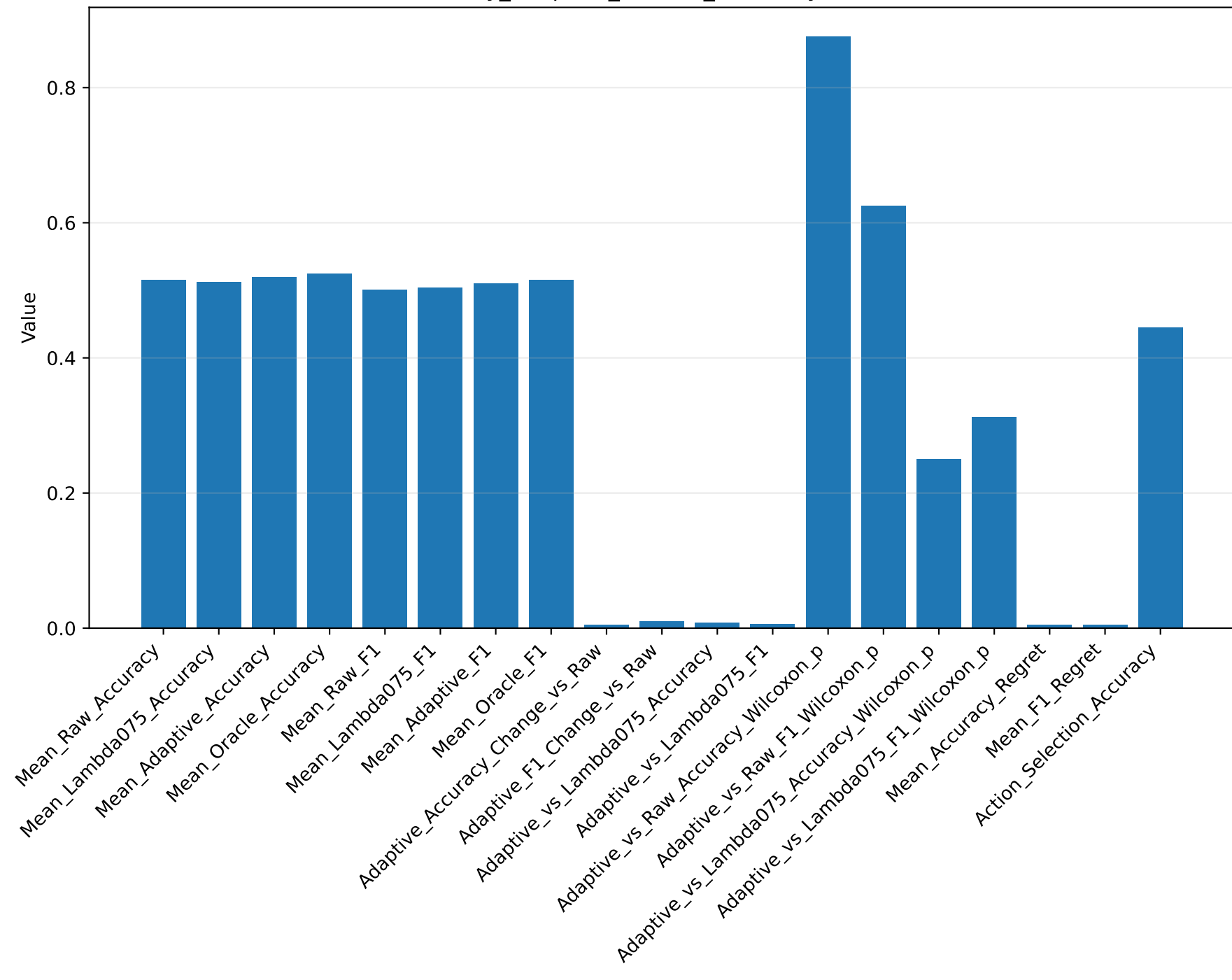
binary_adaptive_lambda_summary: Value
