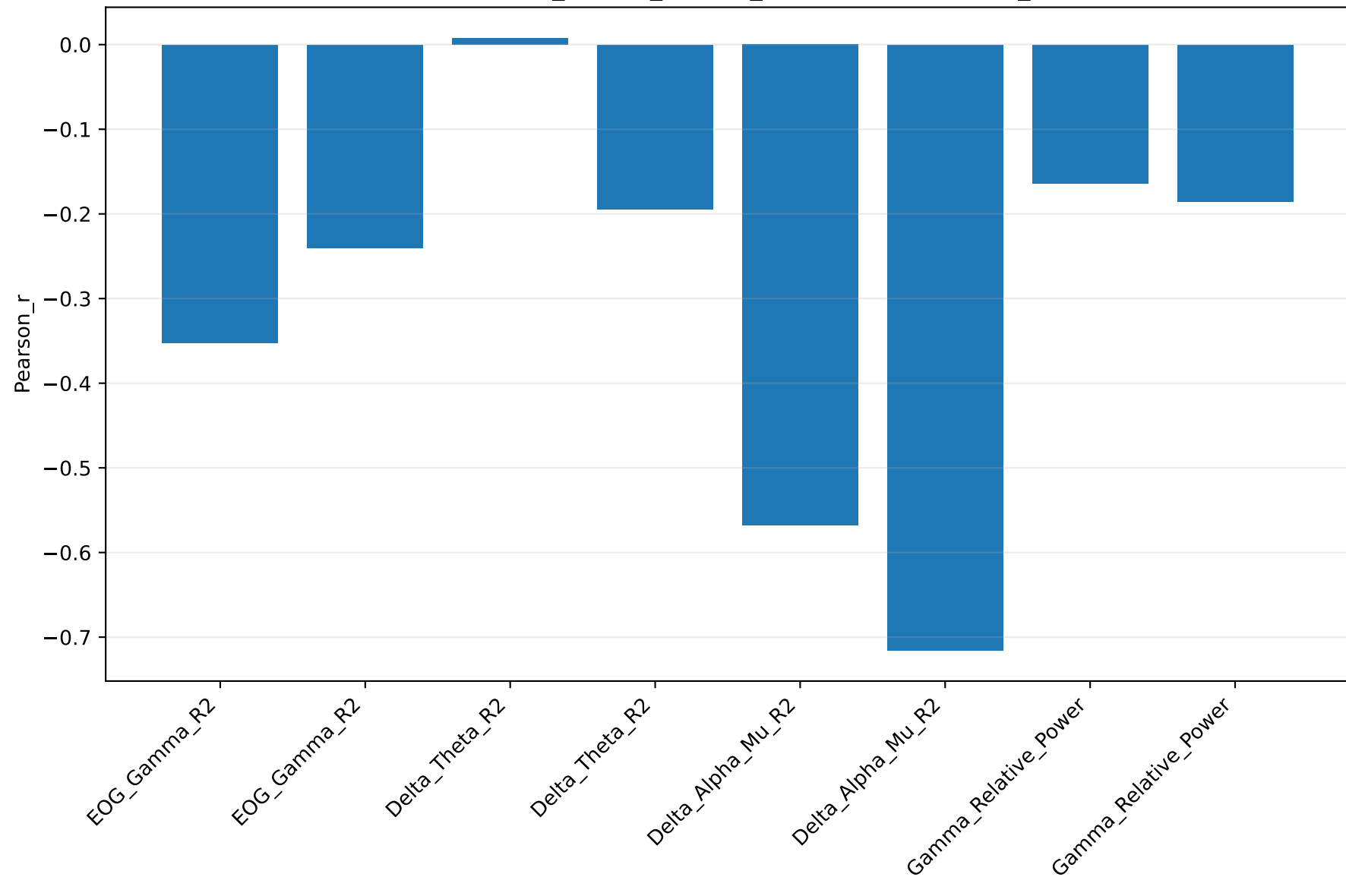
lambda075_benefit_feature_correlations: Pearson_r
