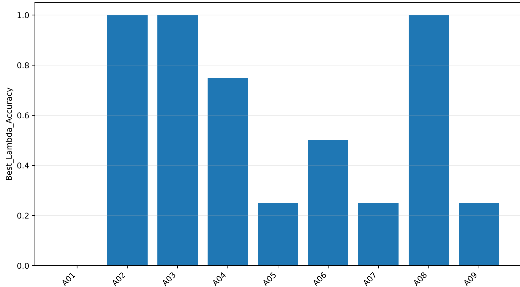
subject_best_allband_lambda: Best_Lambda_Accuracy
