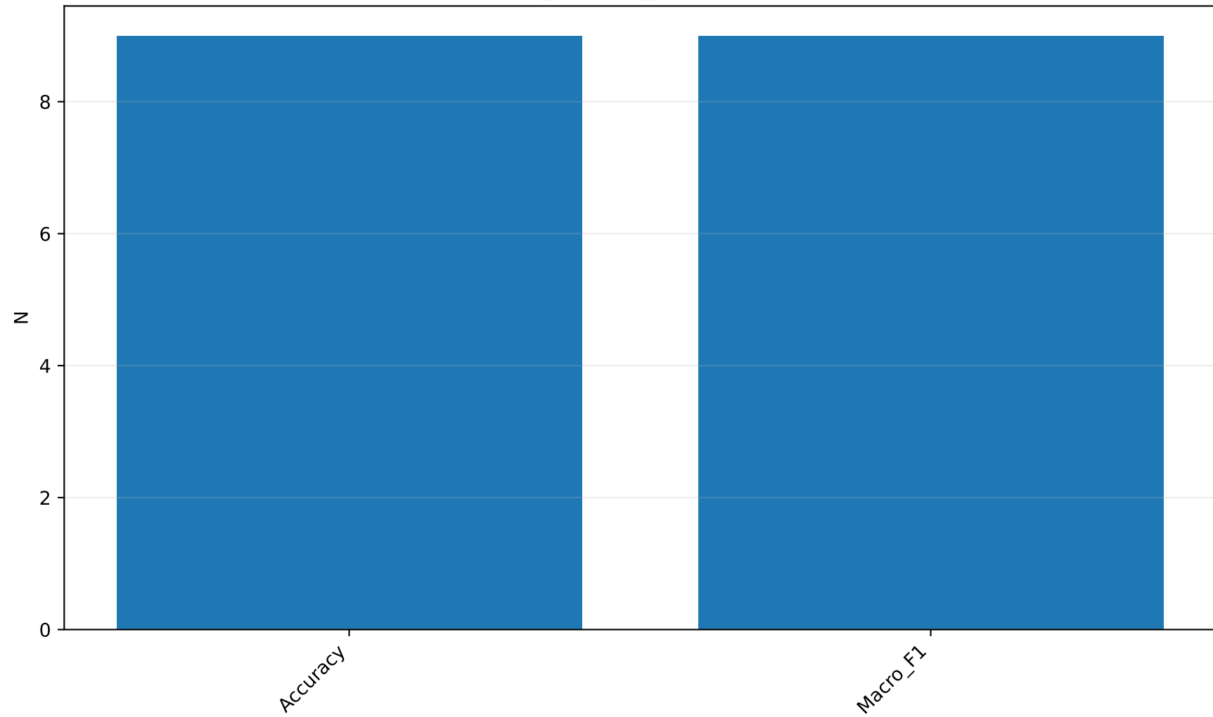
final_primary_statistics: N
