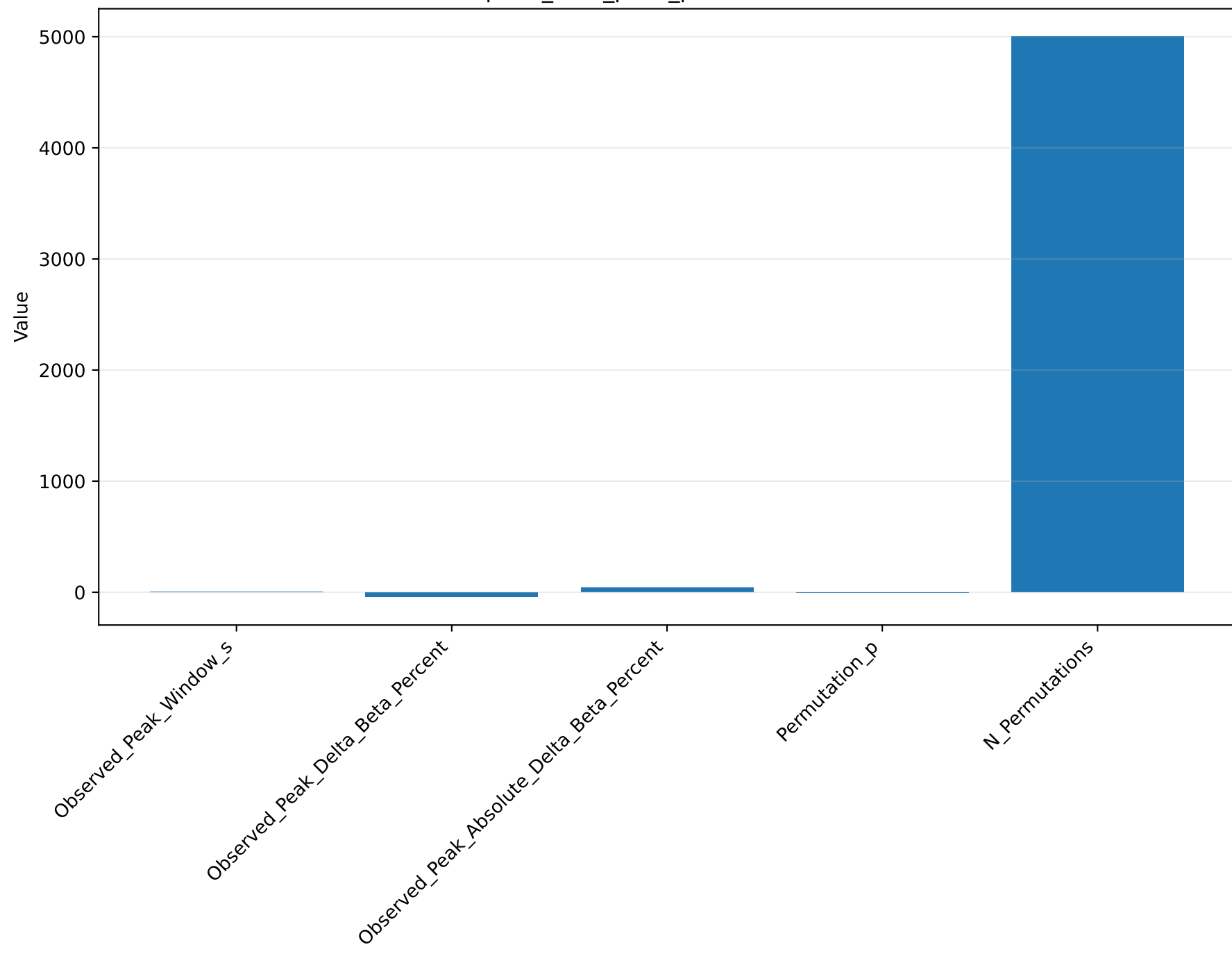
temporal_beta_peak_permutation: Value
