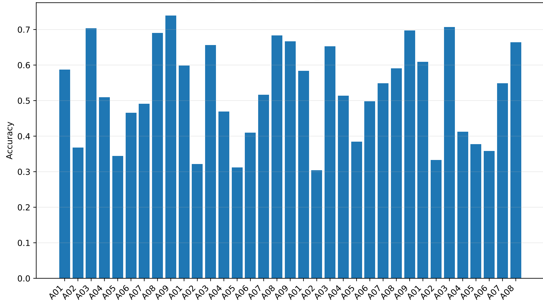
mi_eog_change_vs_cleaning_benefit: Accuracy
