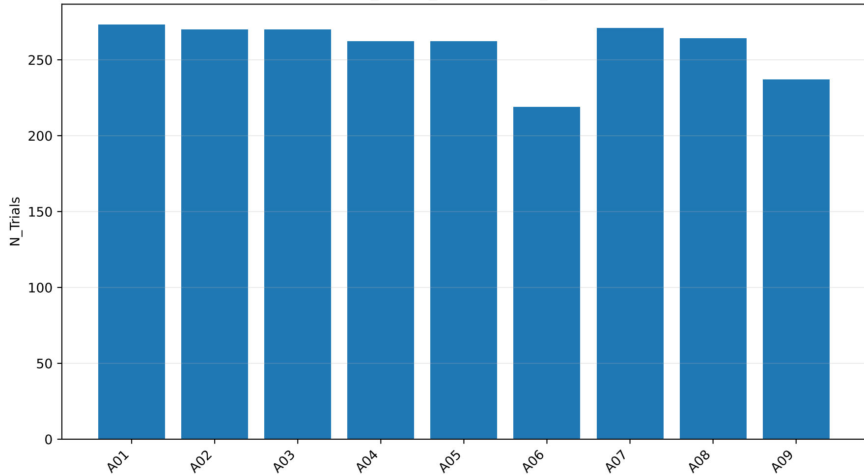
trial_timing_diagnostic: N_Trials
