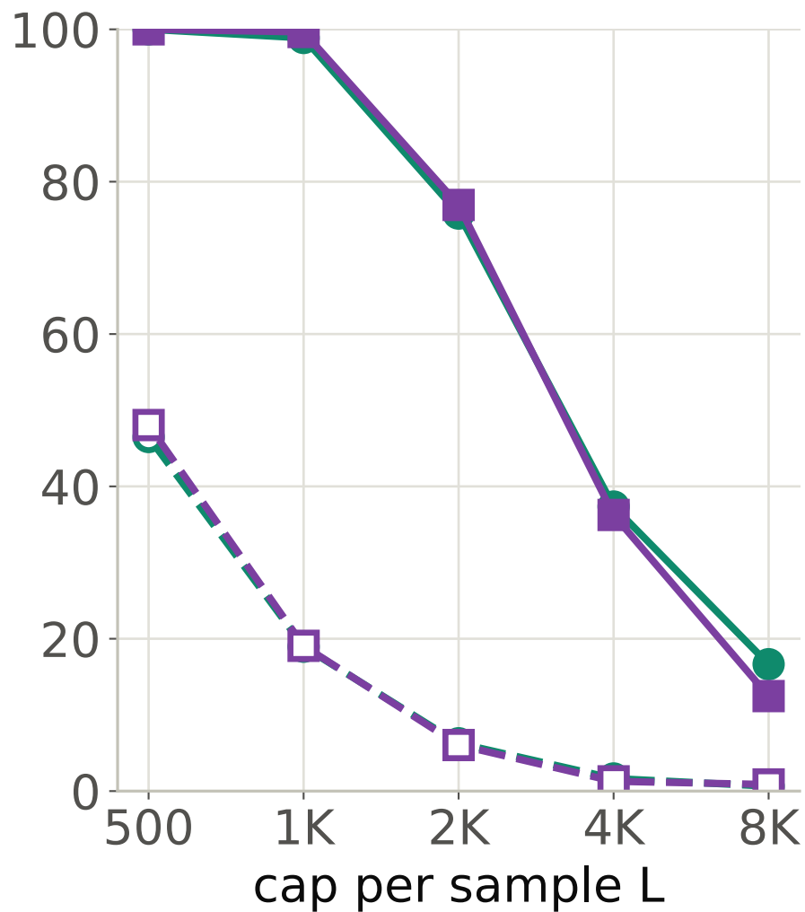
% of samples truncated
