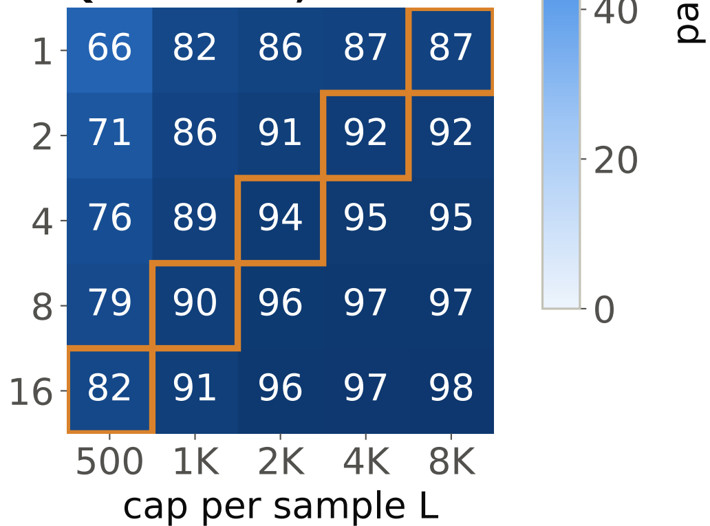
Qwen3-4B, nothink
