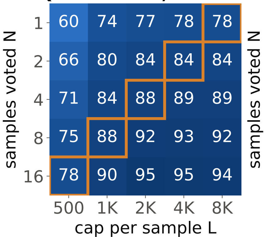
Qwen3-1.7B, nothink
