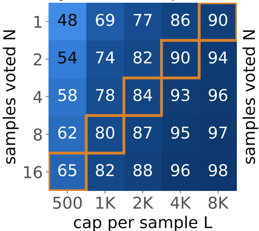
Qwen3-1.7B, nothink
