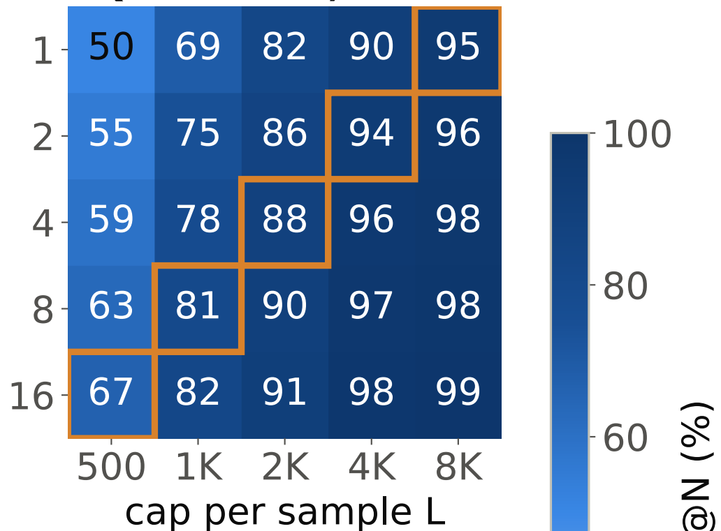
Qwen3-4B, nothink
