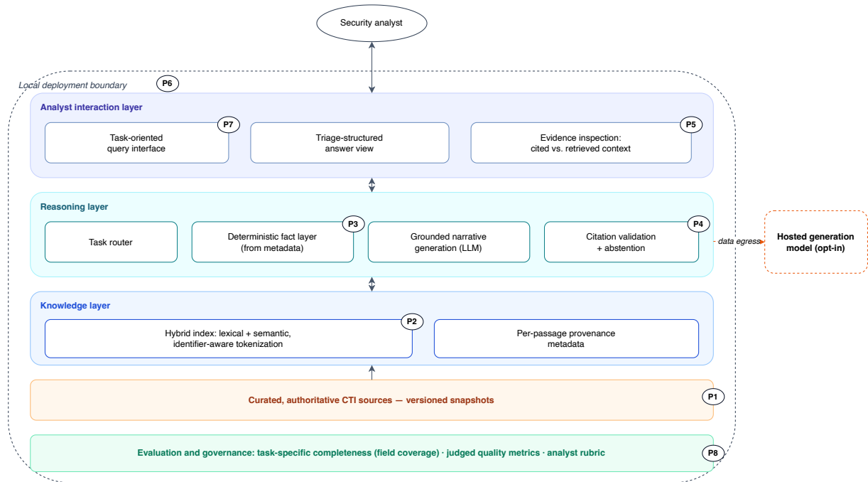
Figure 8: Reference model for integrating RAG into CTI workflows. Badges P1–P8 locate the design principles of Table 15.
