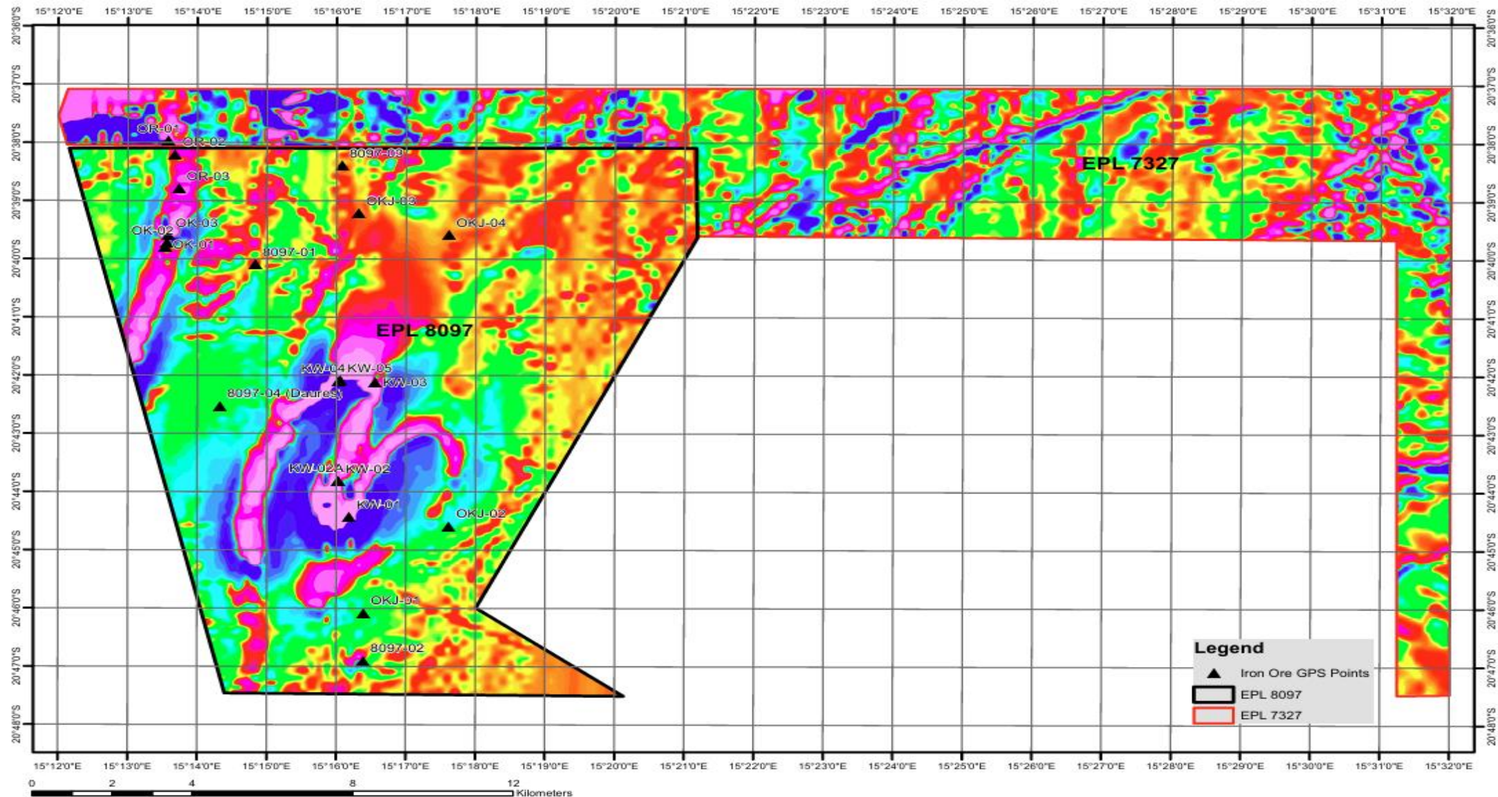
EPL 8097 & 7327 Magnetic Map
