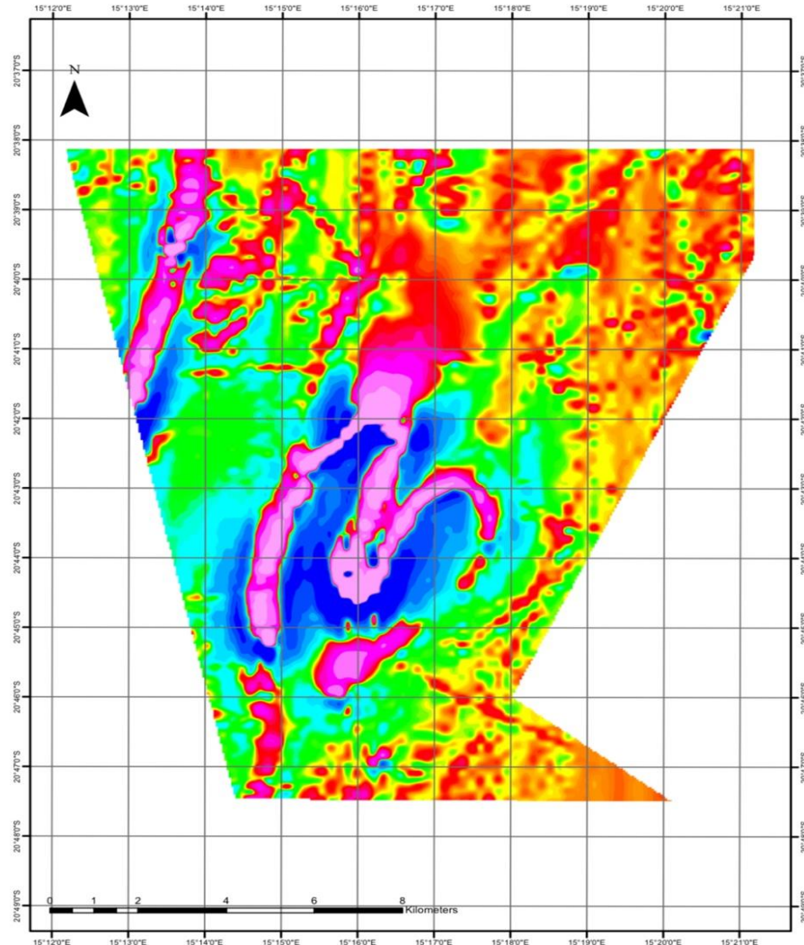
EPL 8097 Mag 1vd Geophysics Map
