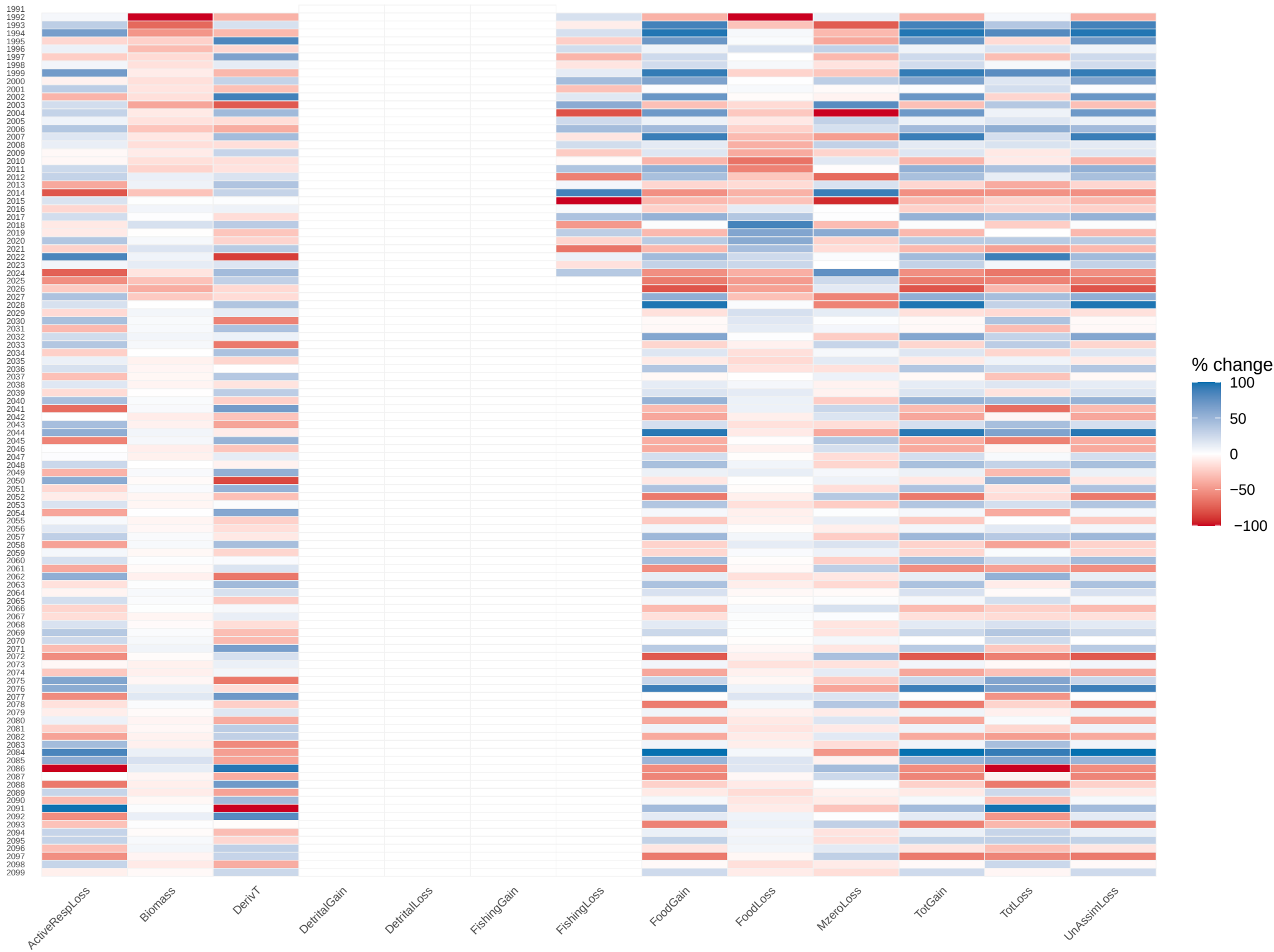
Year to year change: gfdl_126 arrowtooth_flounder_adult
