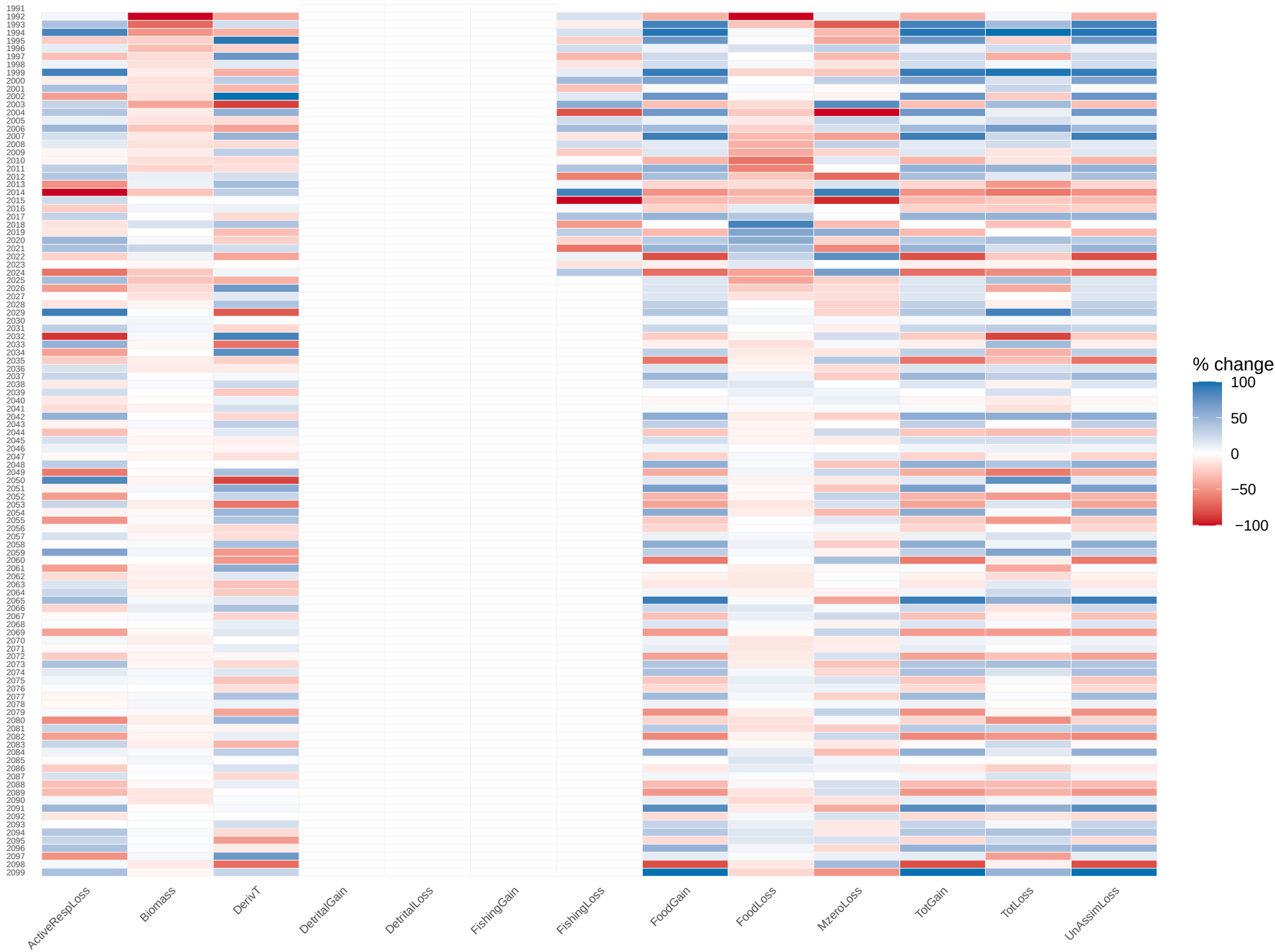
Year to year change: gfdl_245 arrowtooth_flounder_adult
