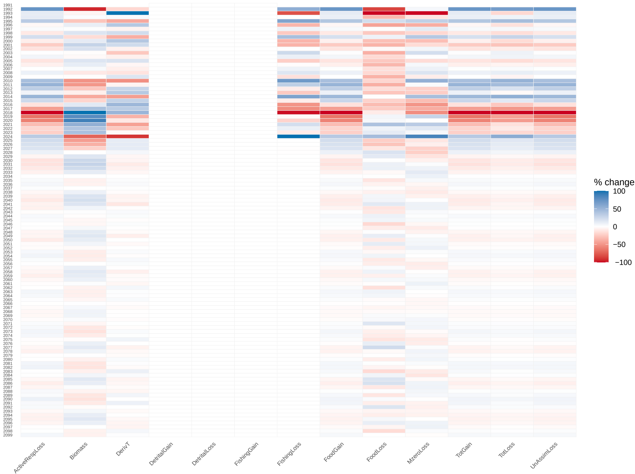
Year to year change: gfdl_126 pacific_cod_adult
