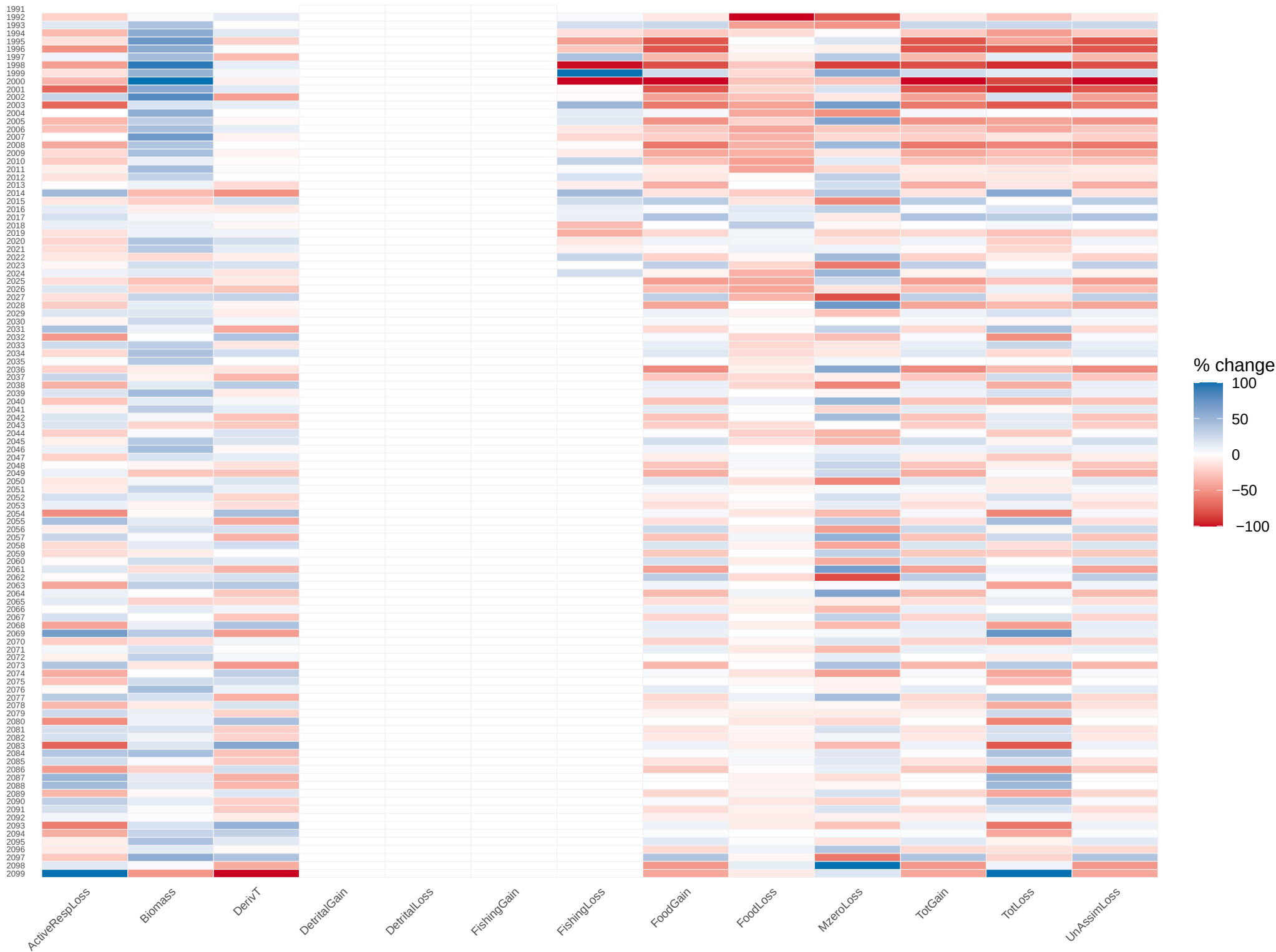
Year to year change: gfdl_585 walleye_pollock_adult
