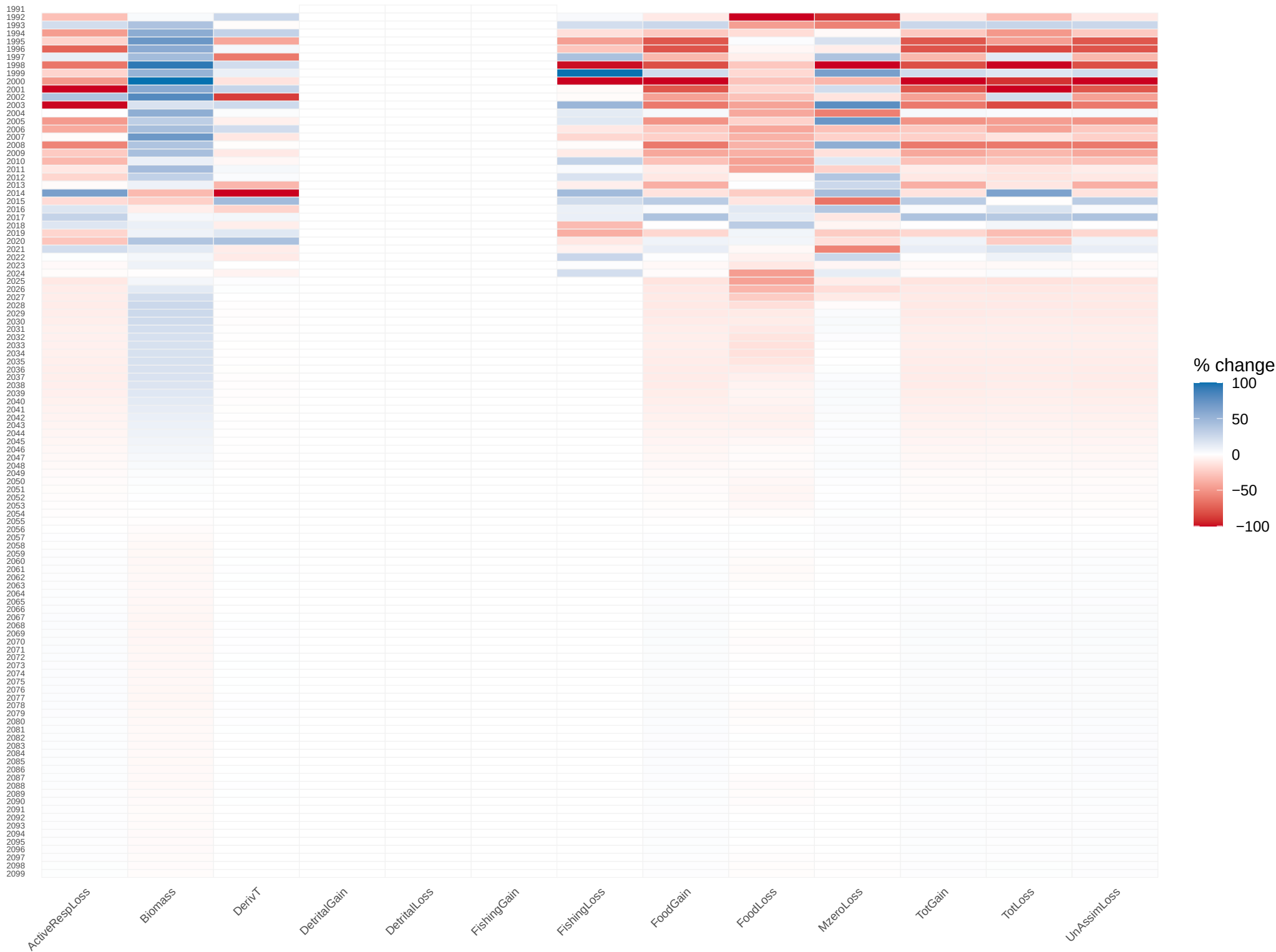
Year to year change: gfdl_persist walleye_pollock_adult
