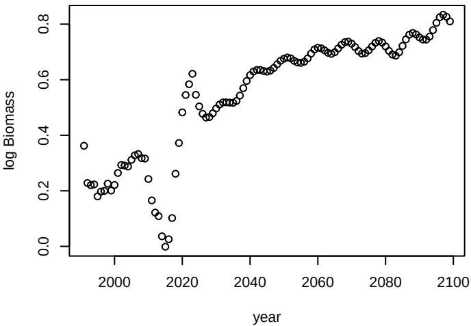
arrowtooth_flounder_adult gfdl_245
