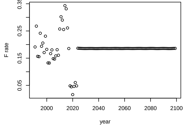
arrowtooth_flounder_adult gfdl_245
