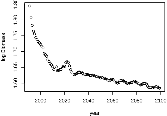
arrowtooth_flounder_adult gfdl_245
