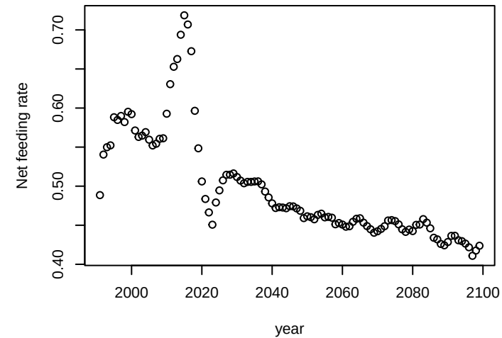
arrowtooth_flounder_adult gfdl_245
