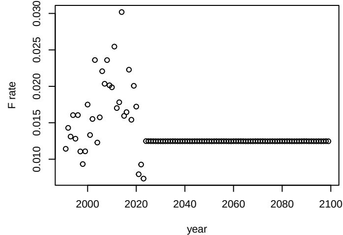
arrowtooth_flounder_adult gfdl_245
