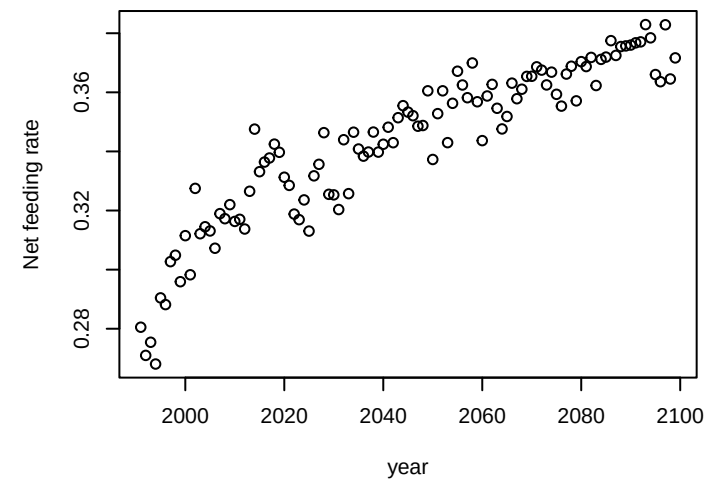
arrowtooth_flounder_adult gfdl_245
