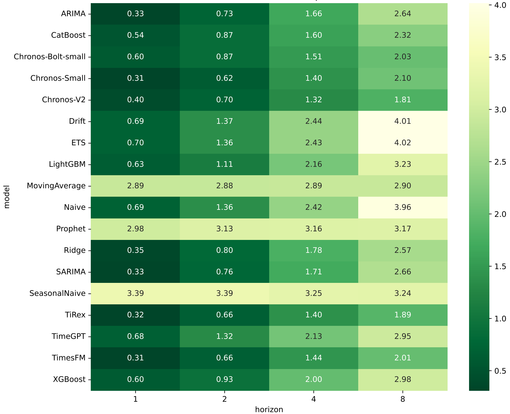
Model Performance Heatmap (MAE)
