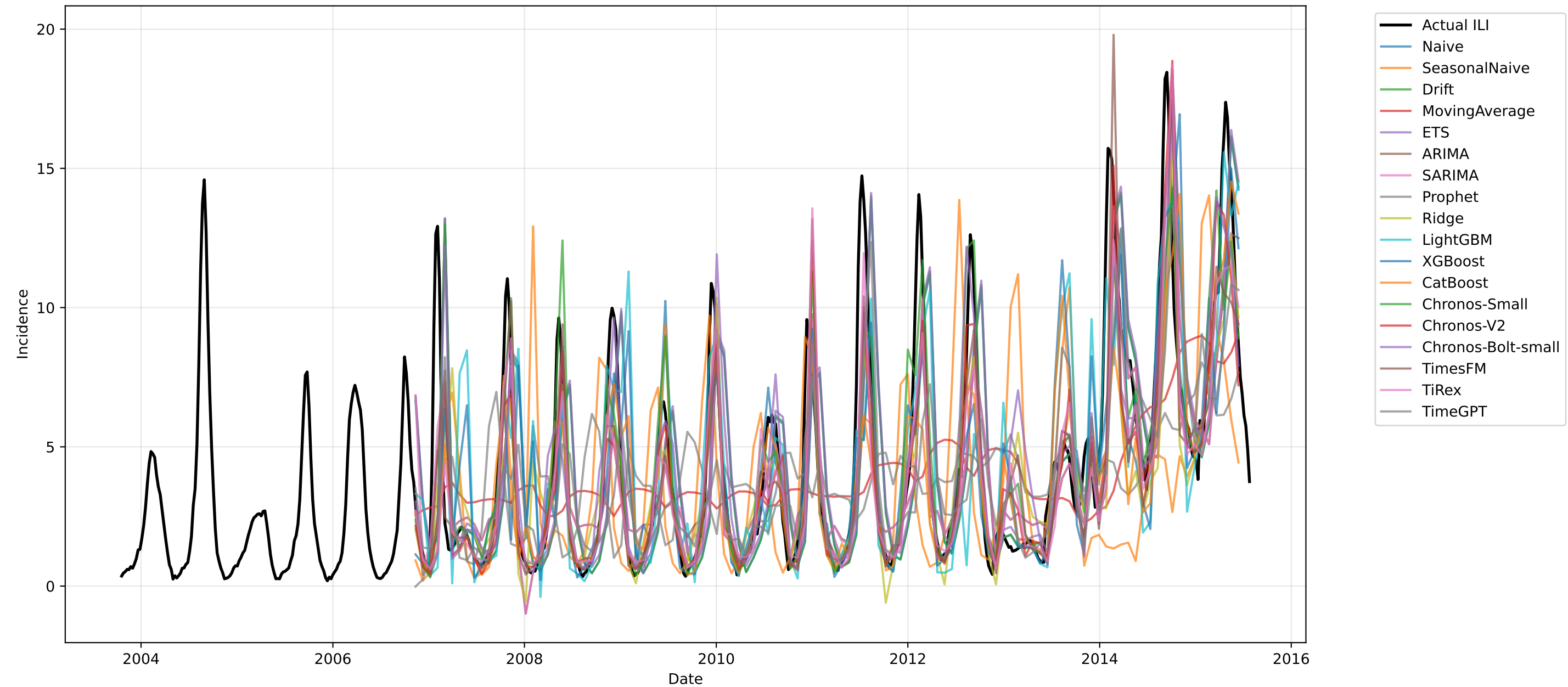
National ILI Forecasts (Horizon: 4 weeks)
