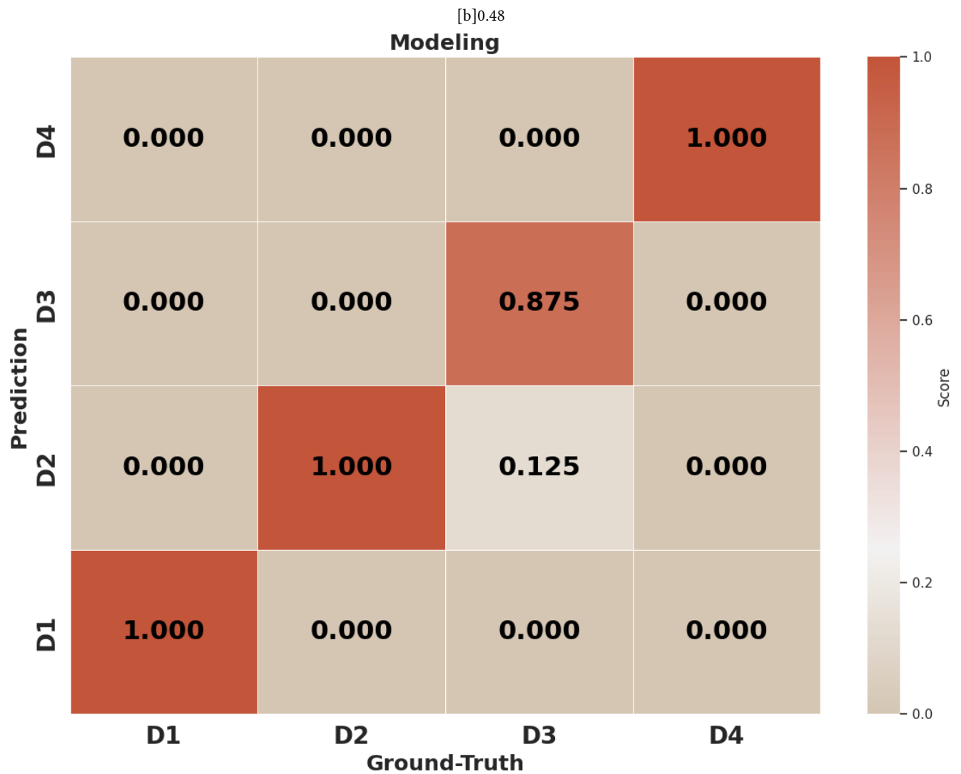
Figure 4: Modeling Heatmap
