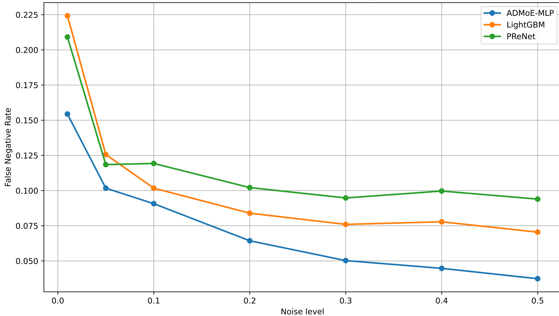
False Negative Rate vs Noise Level - 12_SpamBase
