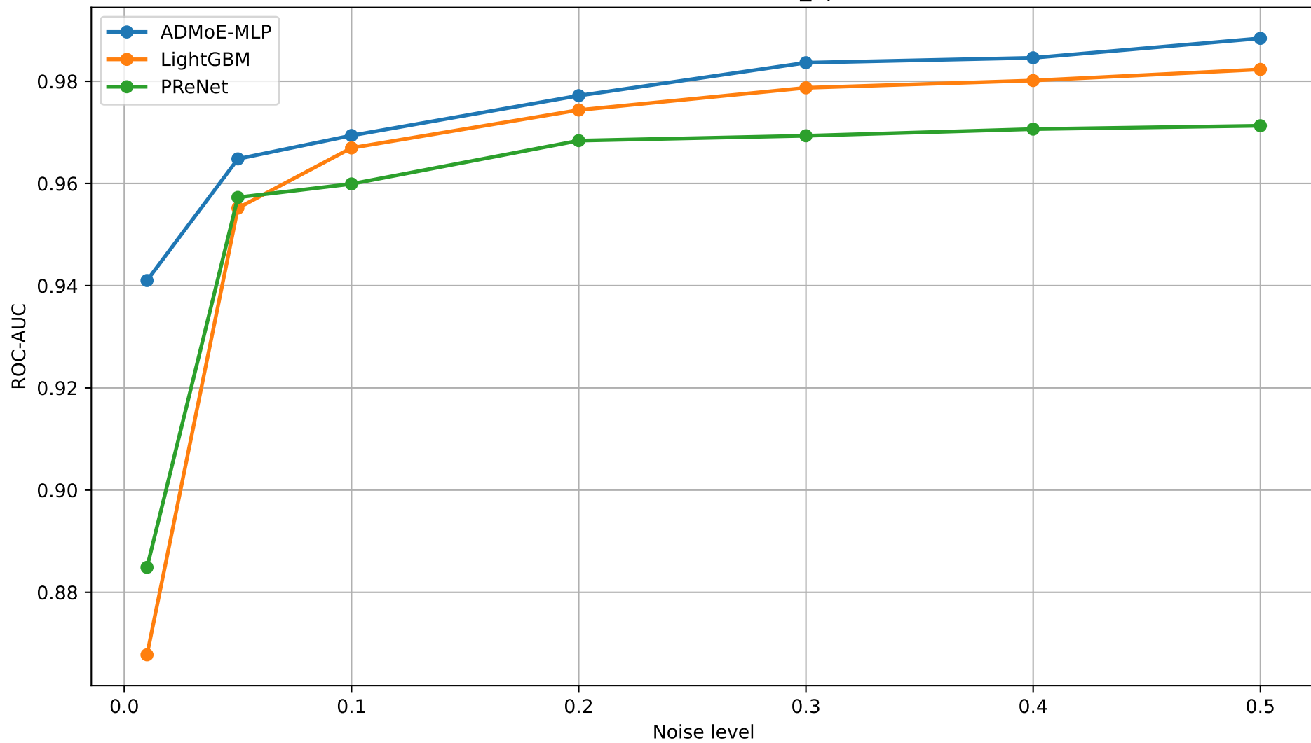
ROC-AUC vs Noise Level - 12_SpamBase
