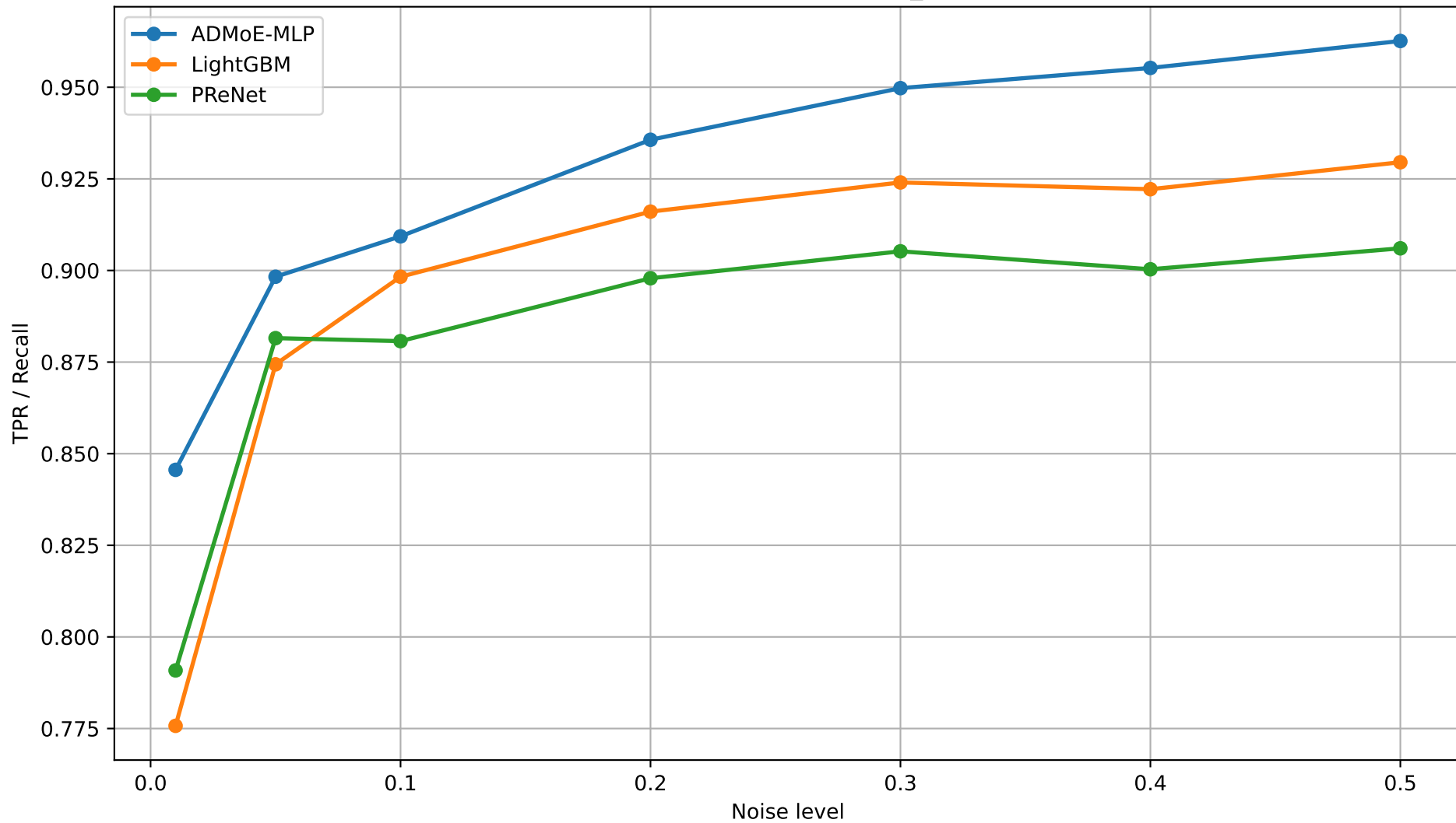
TPR / Recall vs Noise Level - 12_SpamBase
