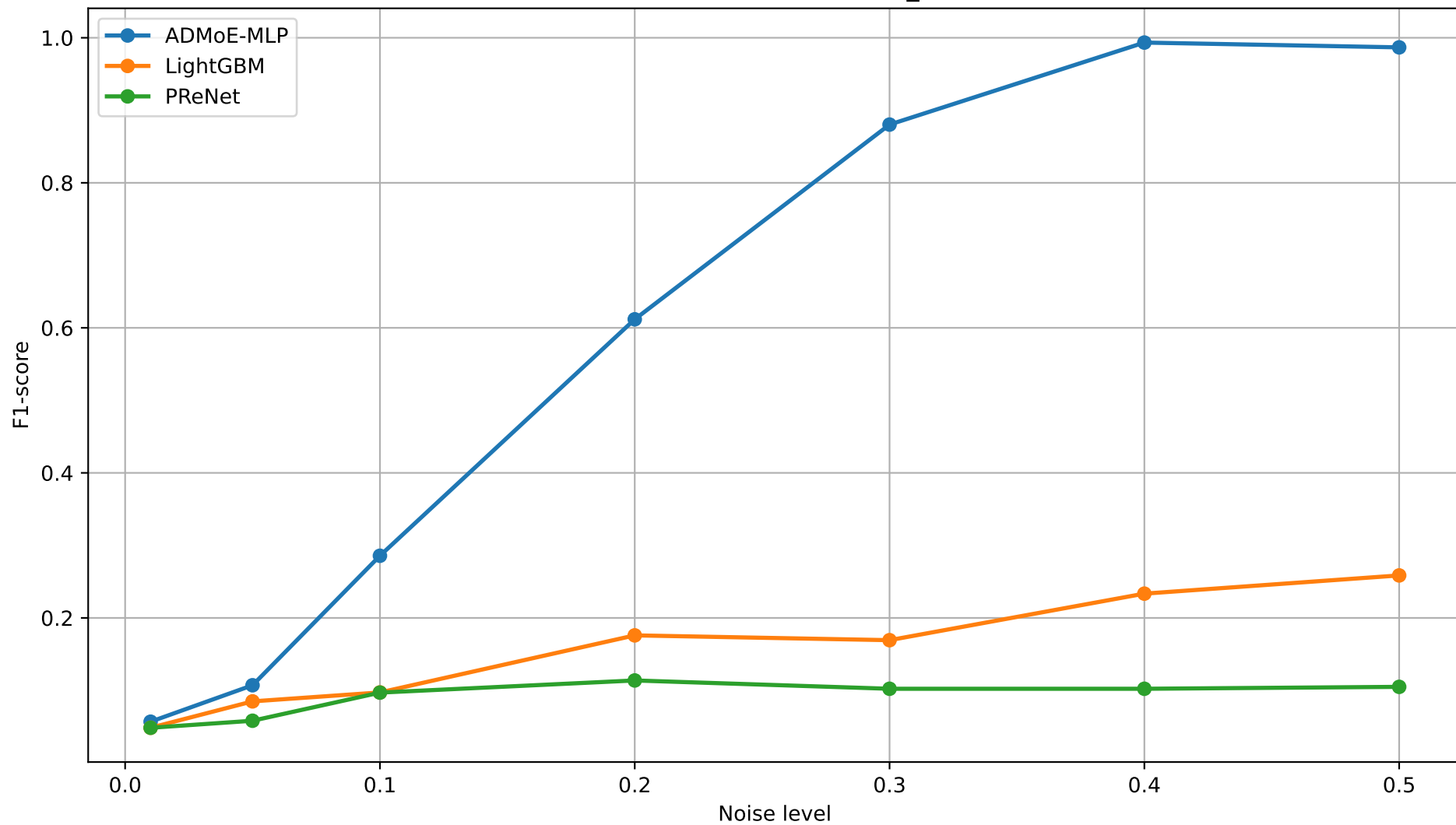
F1-score vs Noise Level - 1_ALOI
