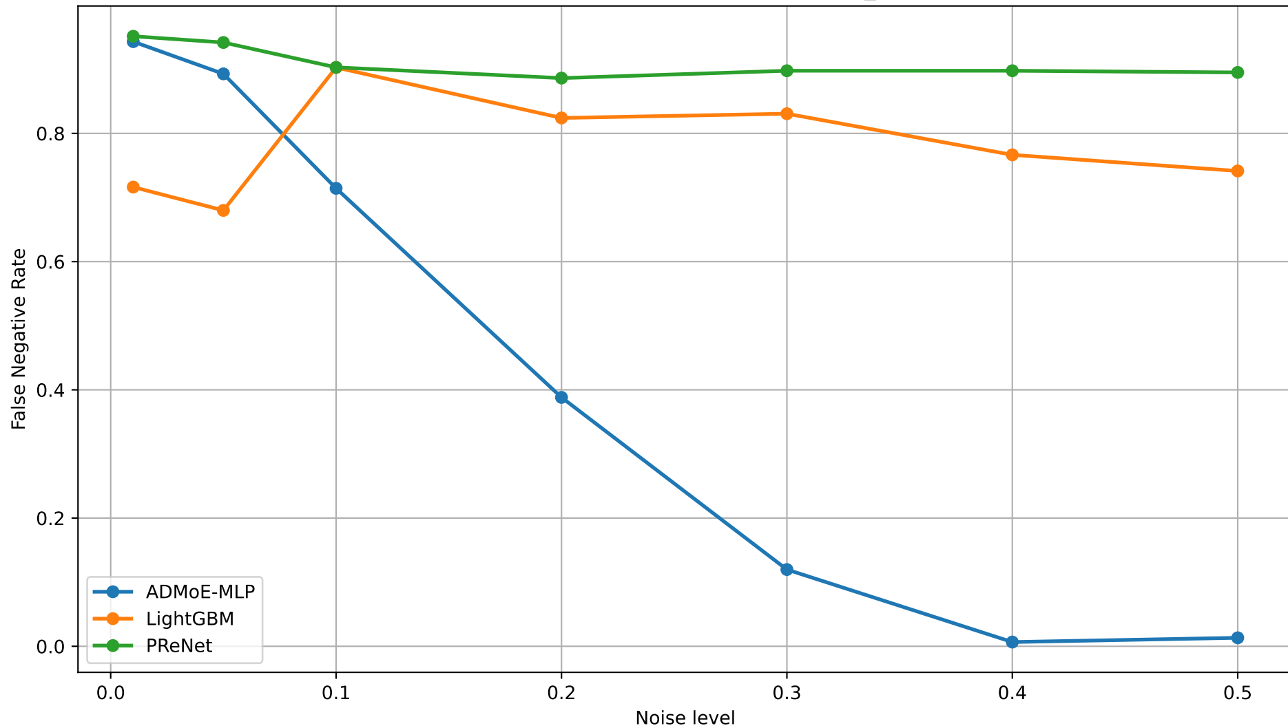
False Negative Rate vs Noise Level - 1_ALOI
