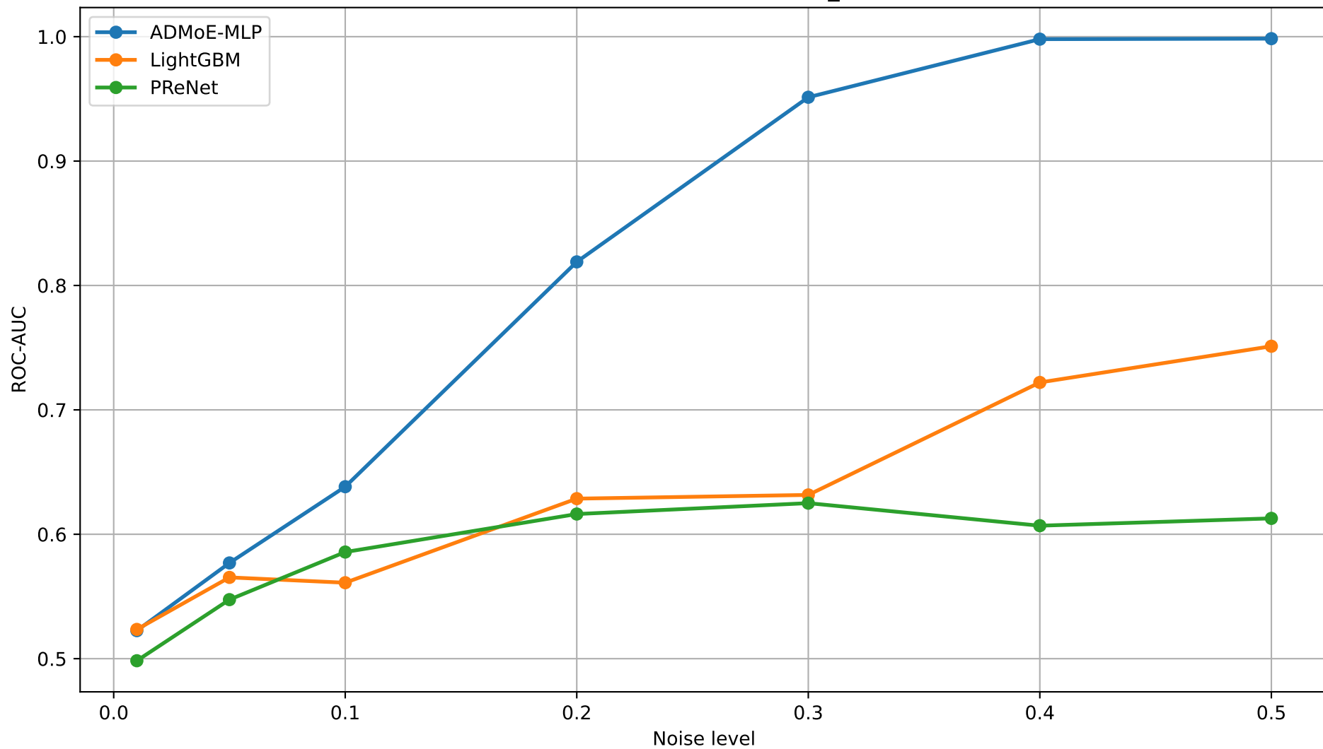
ROC-AUC vs Noise Level - 1_ALOI
