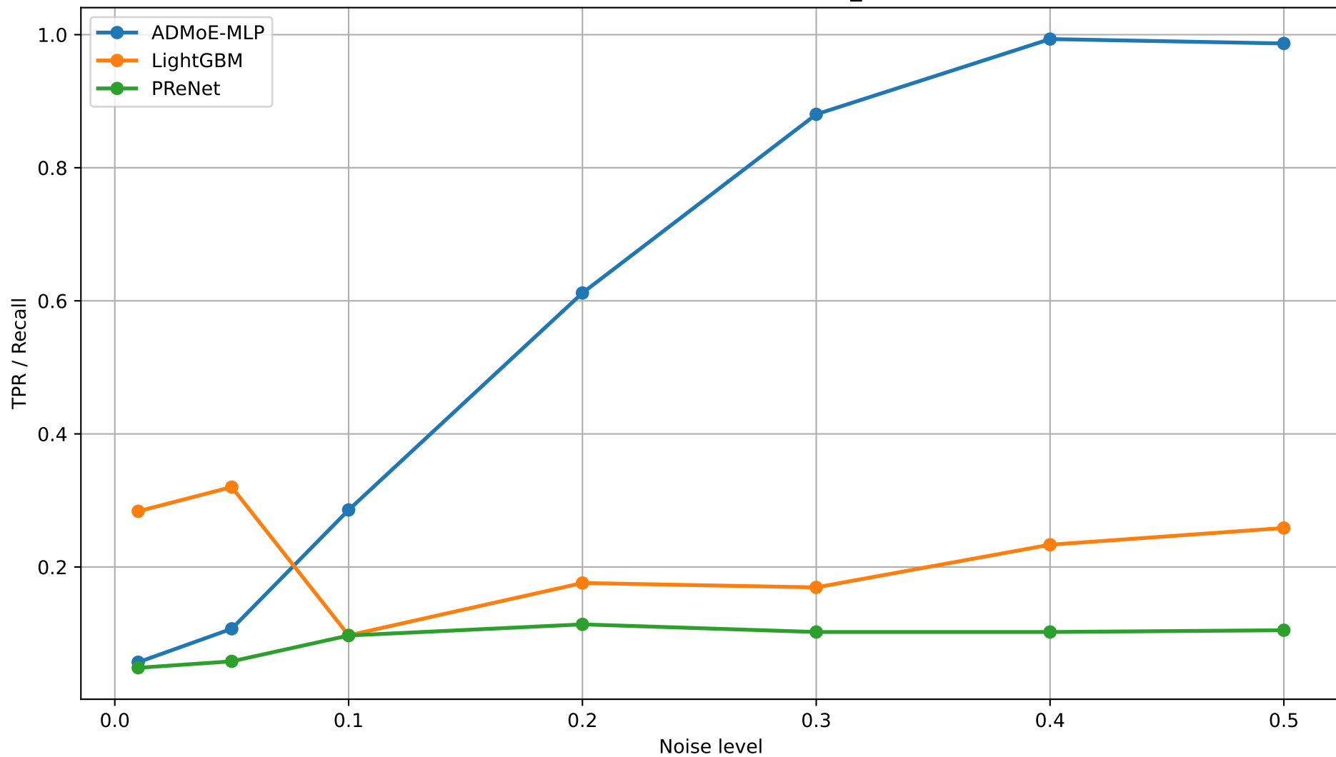
TPR / Recall vs Noise Level - 1_ALOI
