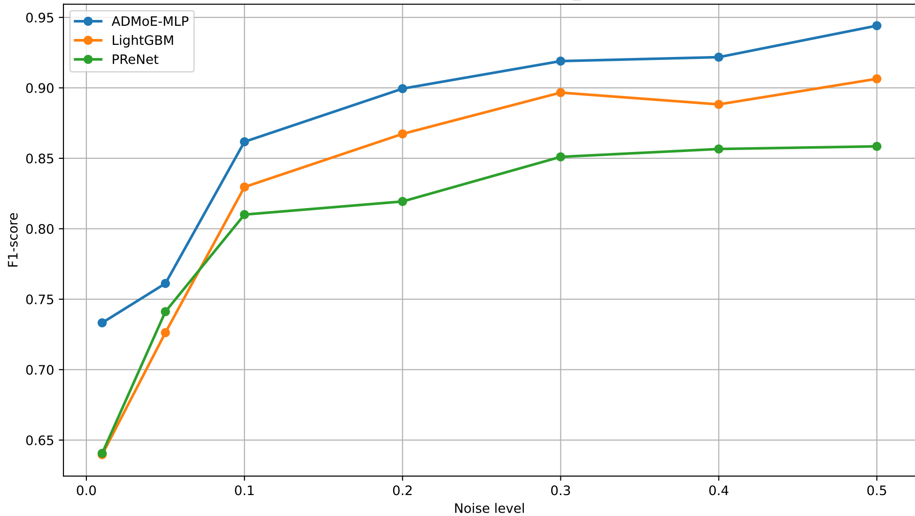
F1-score vs Noise Level - 27_mnist
