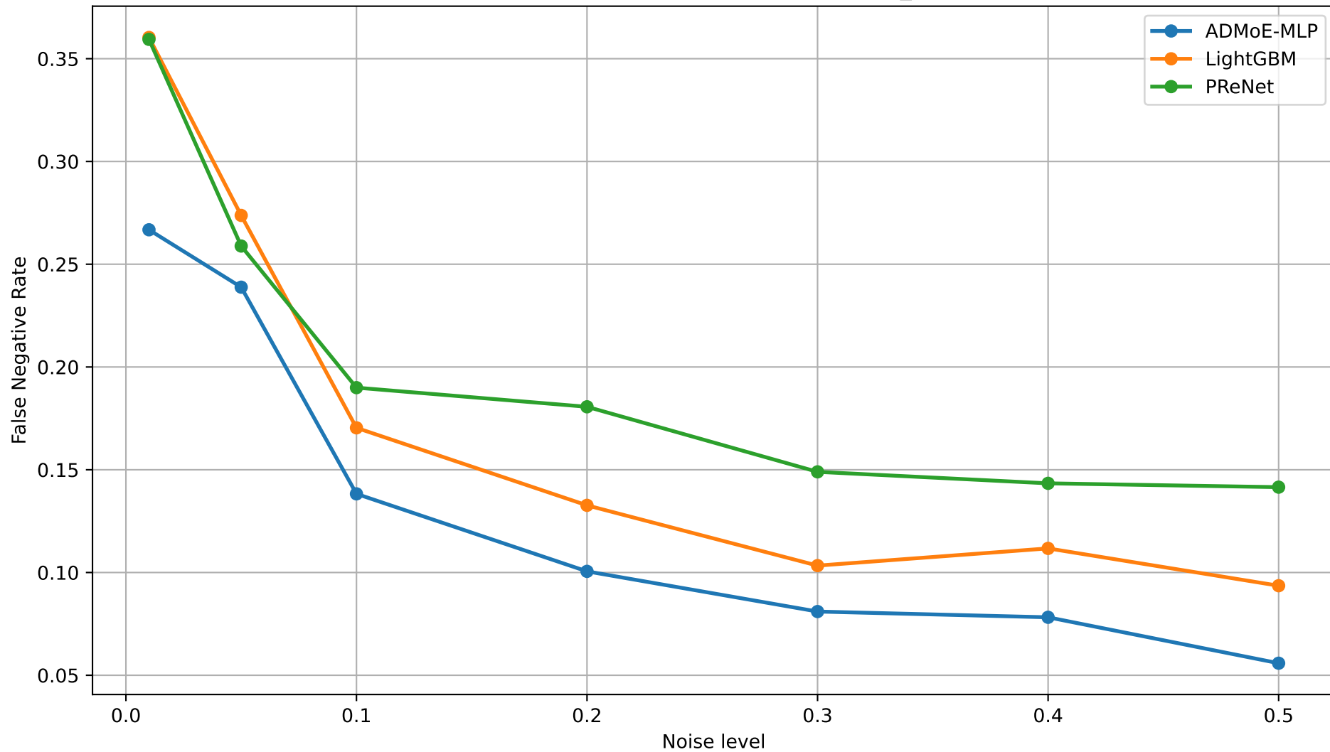
False Negative Rate vs Noise Level - 27_mnist
