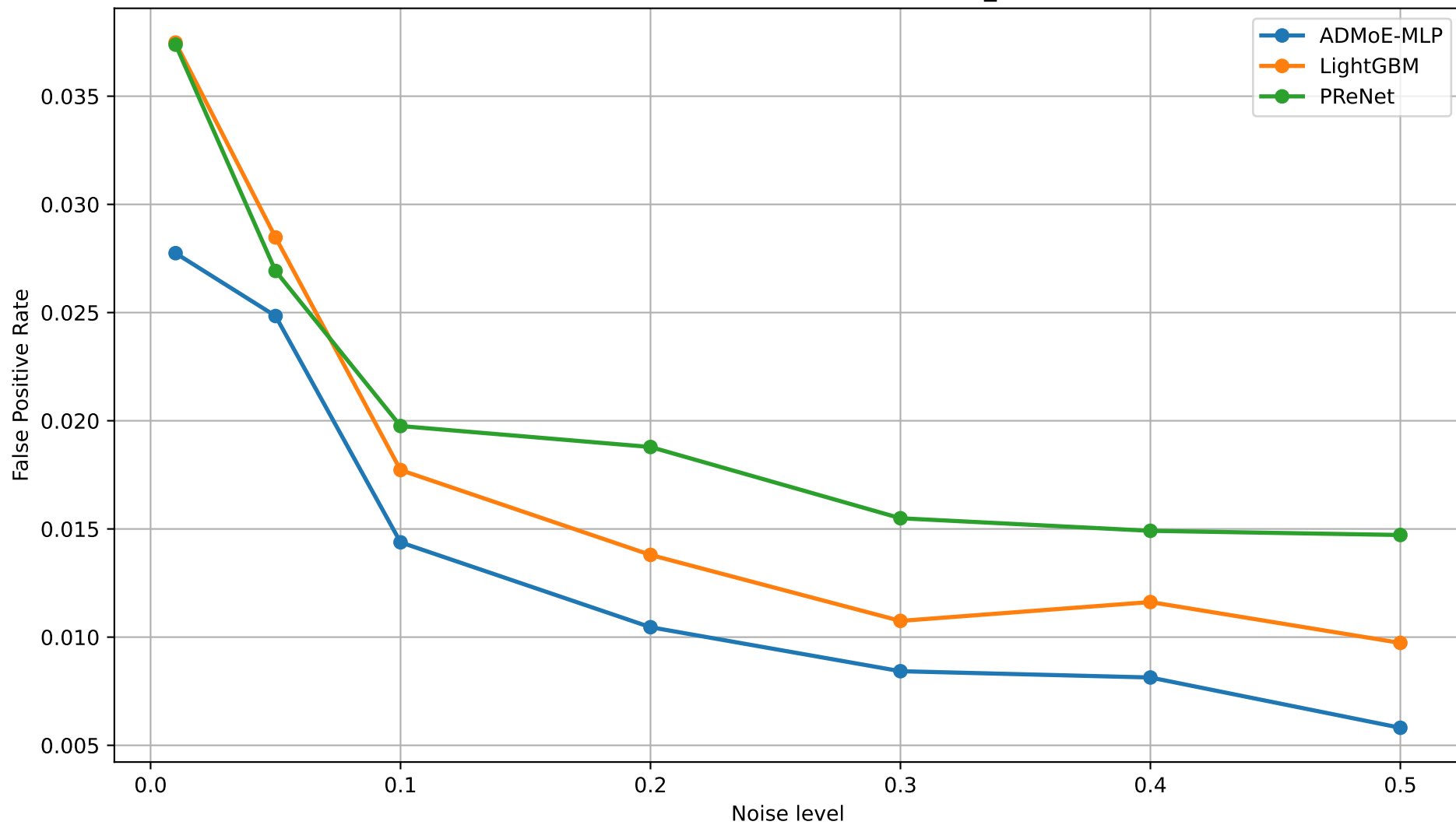
False Positive Rate vs Noise Level - 27_mnist
