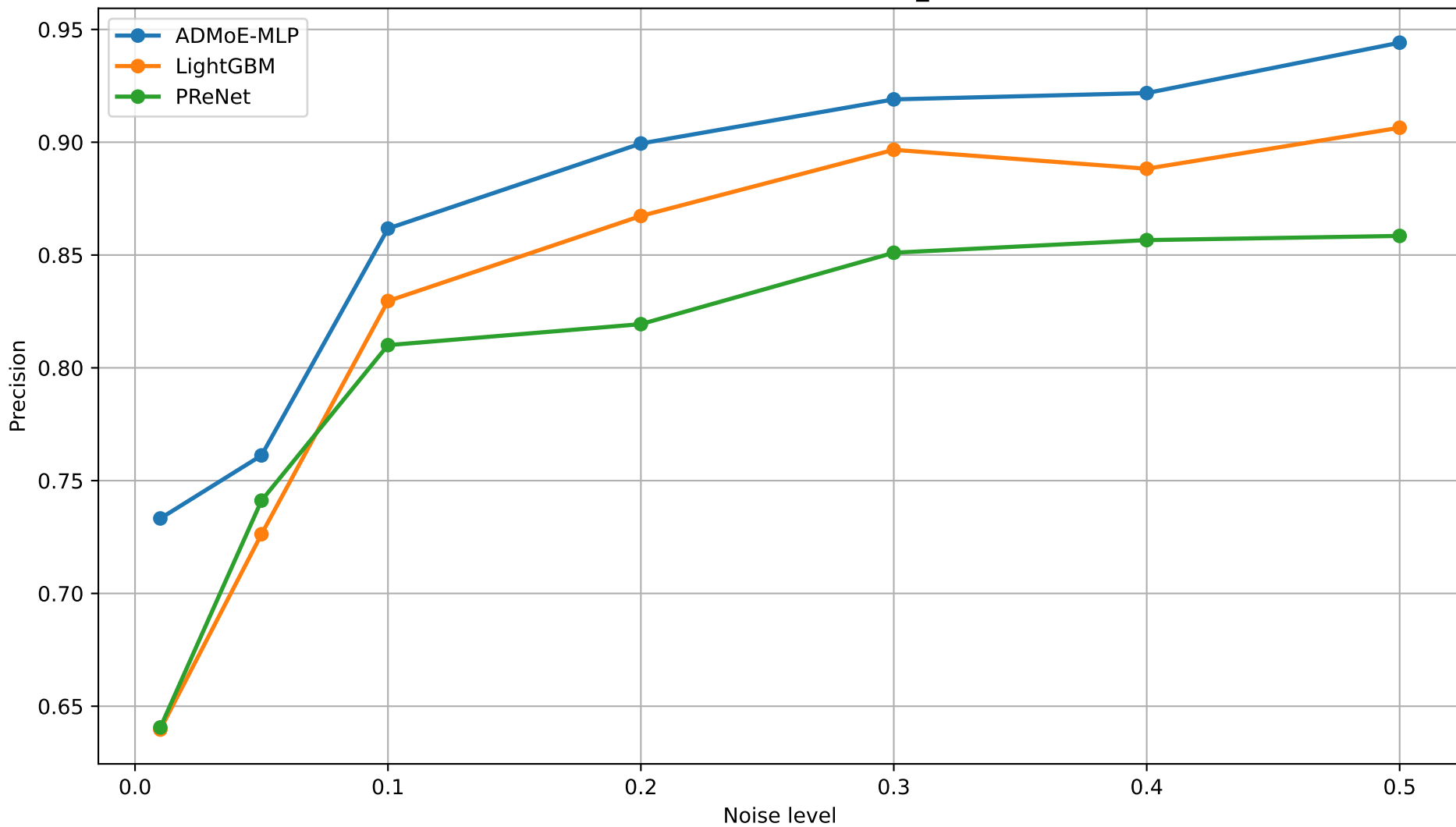
Precision vs Noise Level - 27_mnist
