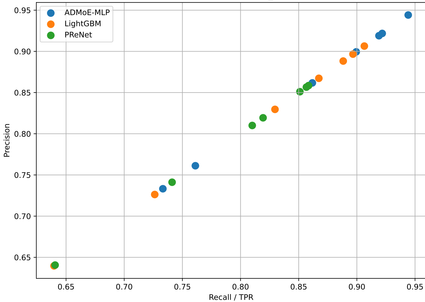
Precision vs Recall - 27_mnist
