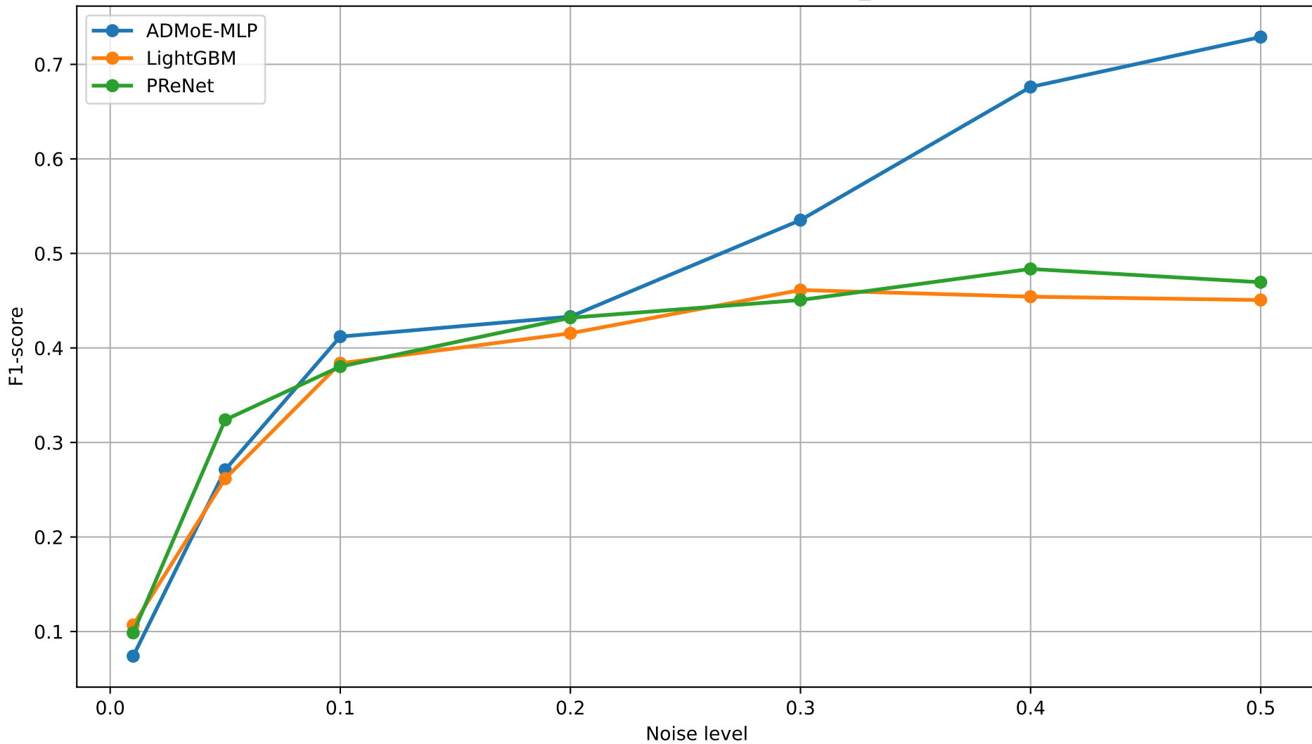
F1-score vs Noise Level - SVHN_0
