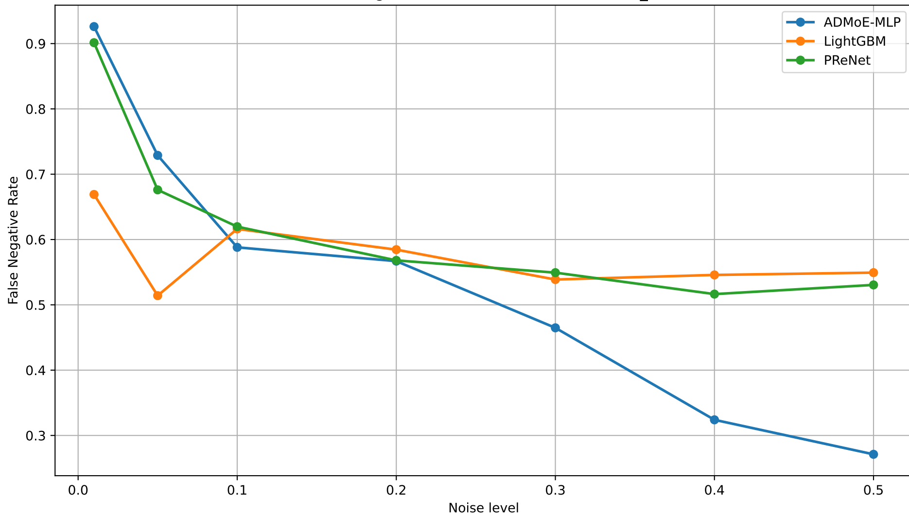
False Negative Rate vs Noise Level - SVHN_0
