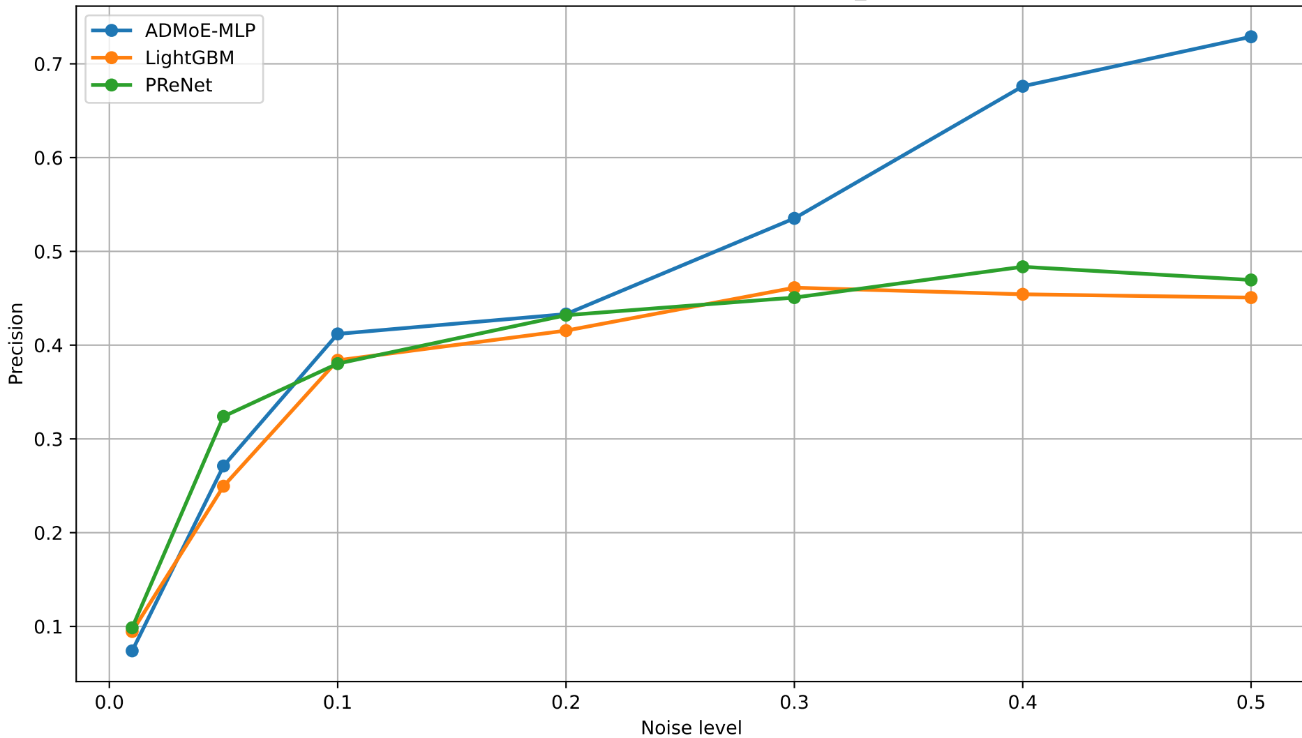
Precision vs Noise Level - SVHN_0
