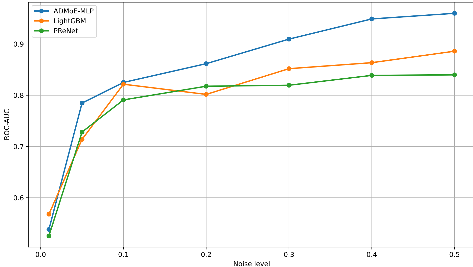
ROC-AUC vs Noise Level - SVHN_0
