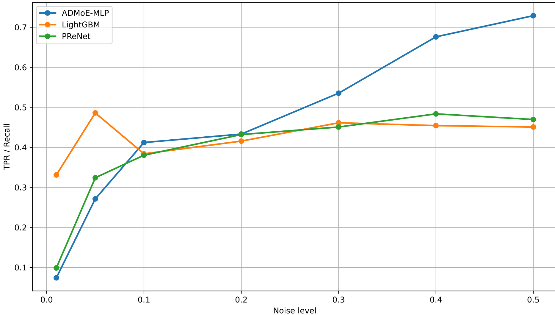
TPR / Recall vs Noise Level - SVHN_0
