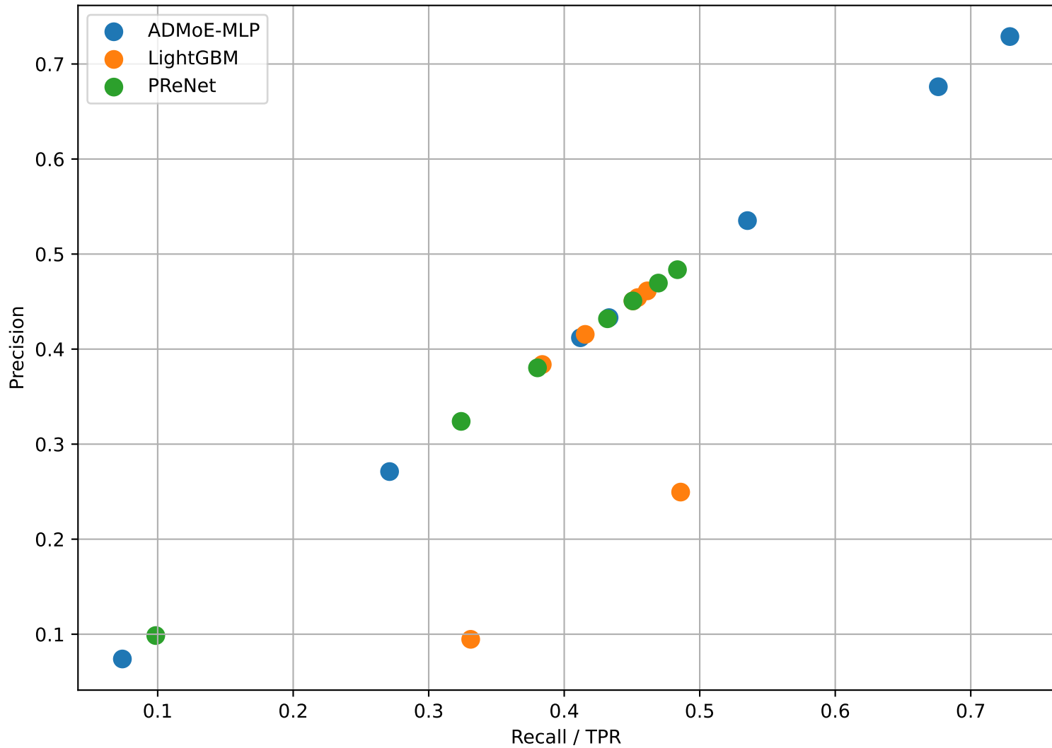
Precision vs Recall - SVHN_0
