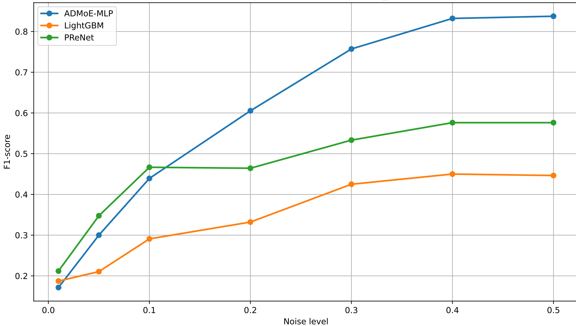
F1-score vs Noise Level - agnews_0
