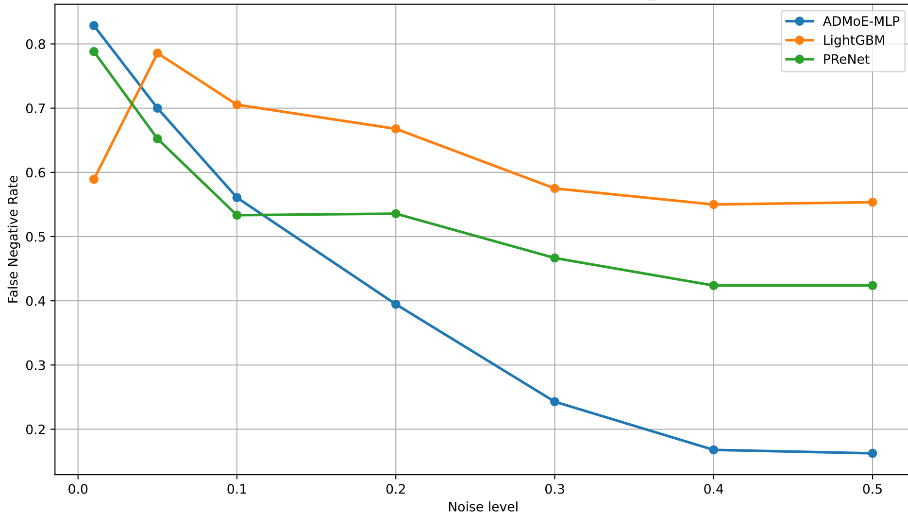
False Negative Rate vs Noise Level - agnews_0
