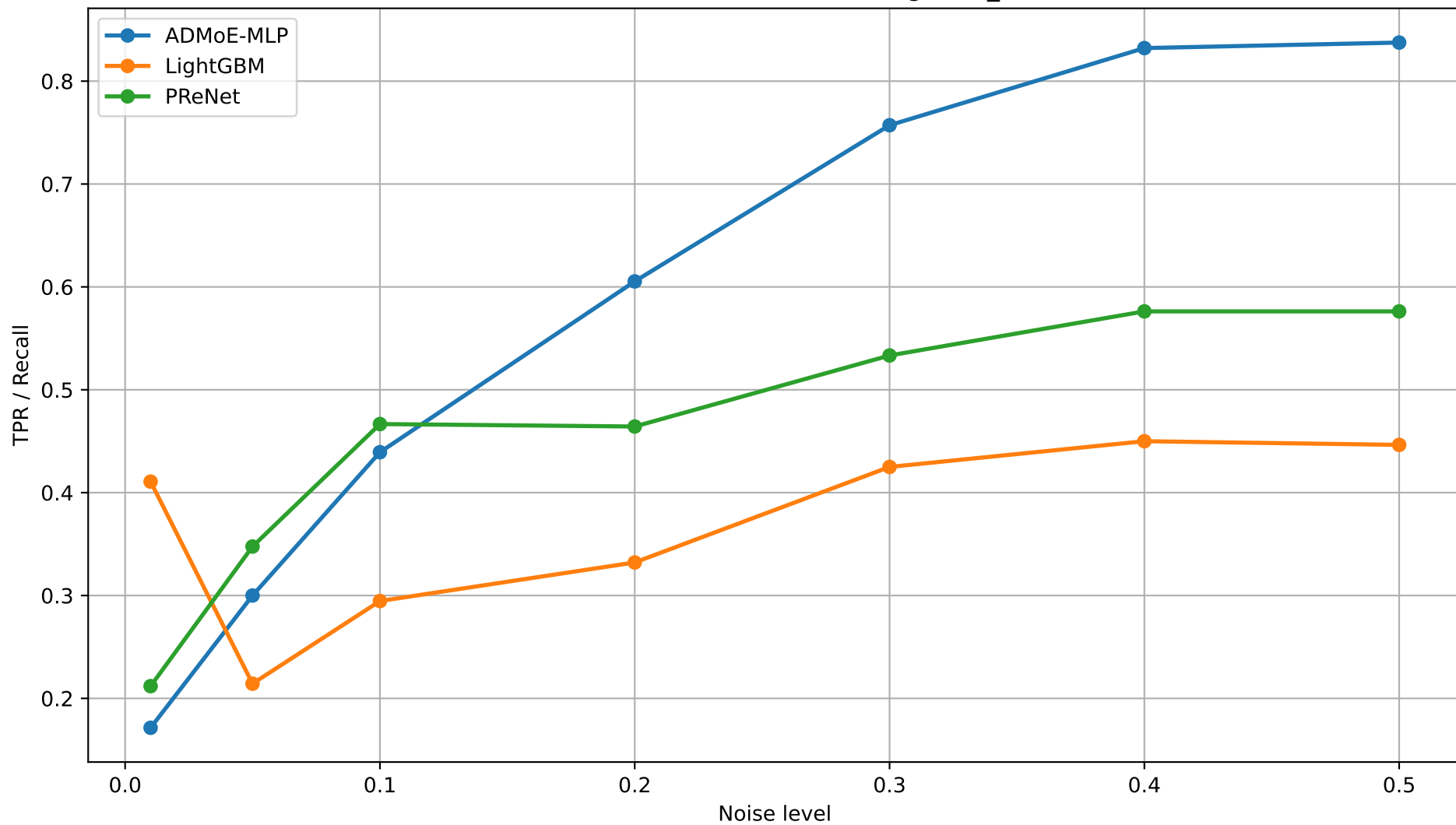
TPR / Recall vs Noise Level - agnews_0
