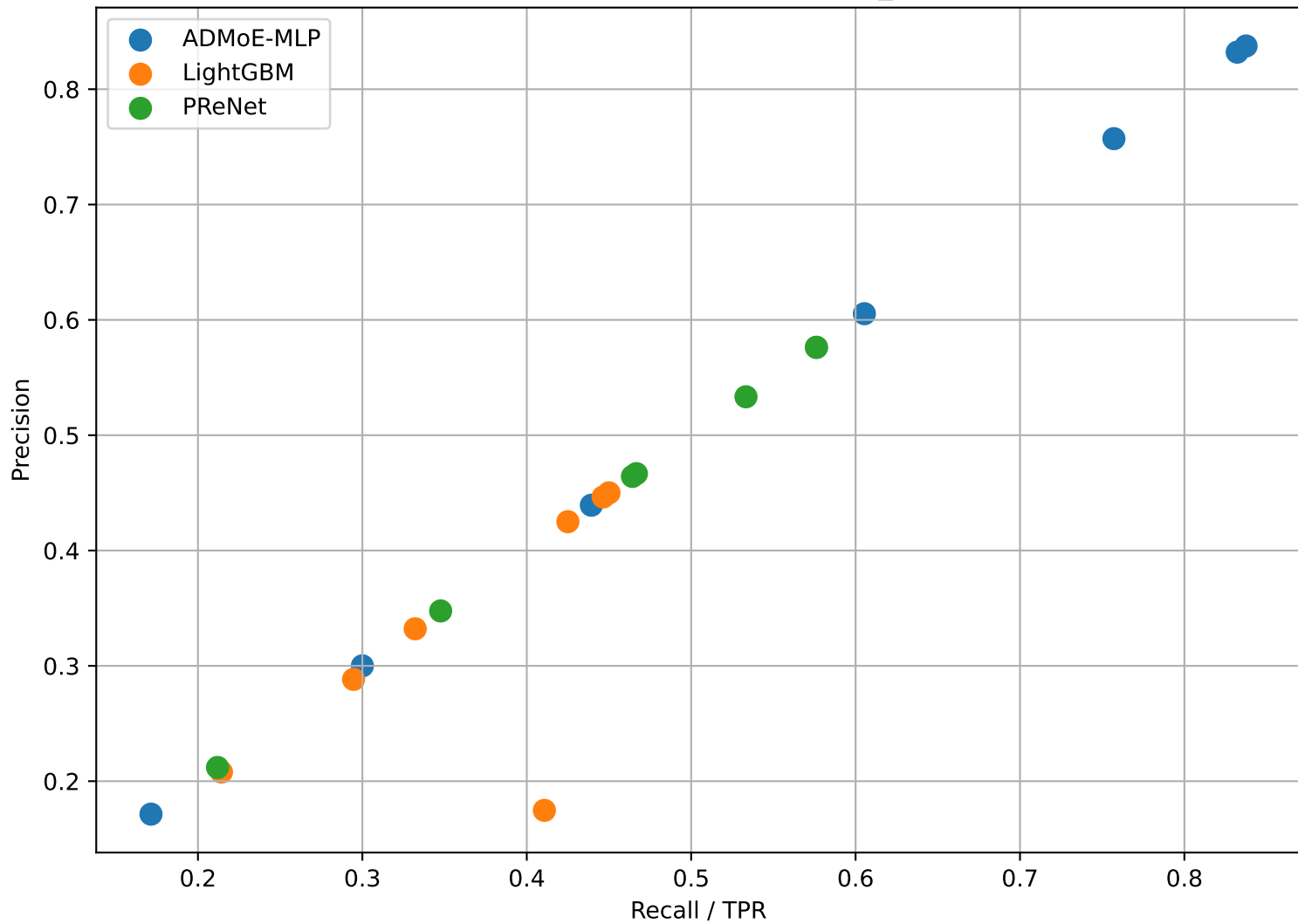
Precision vs Recall - agnews_0
