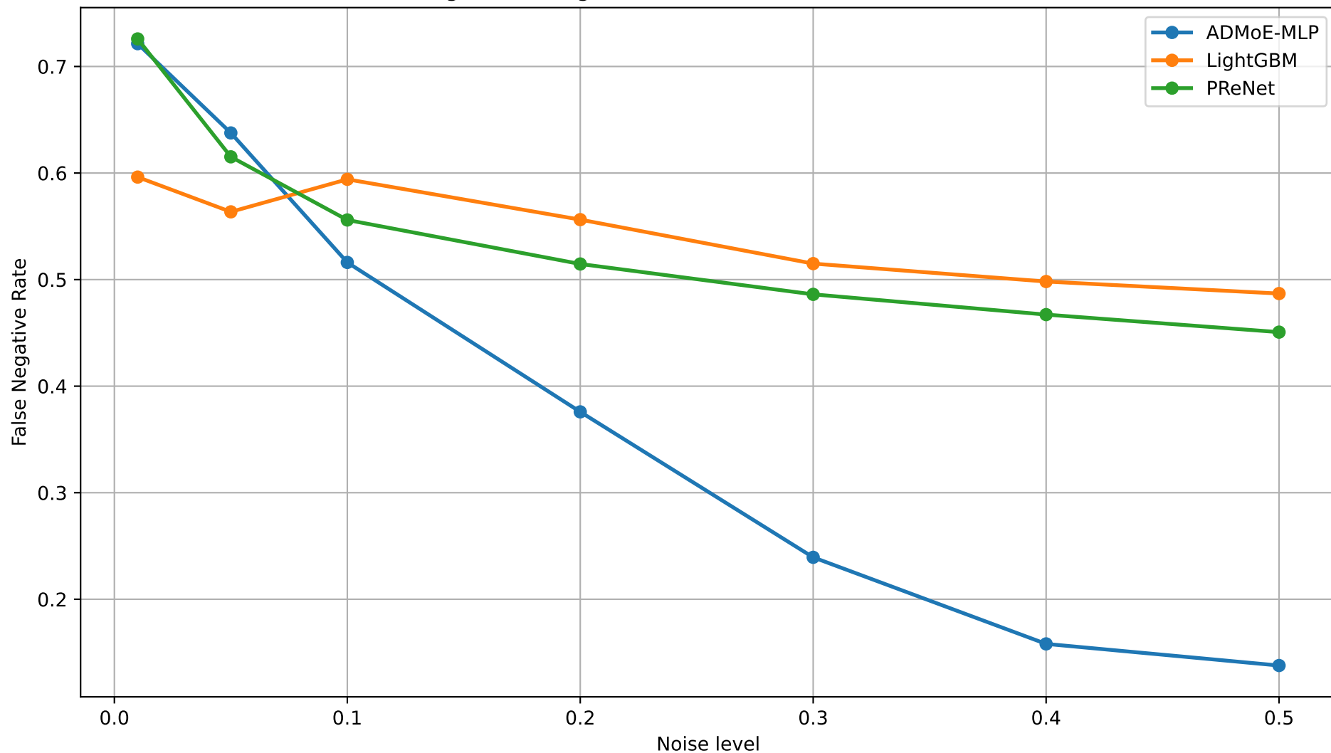
Average False Negative Rate vs Noise Level - All Datasets
