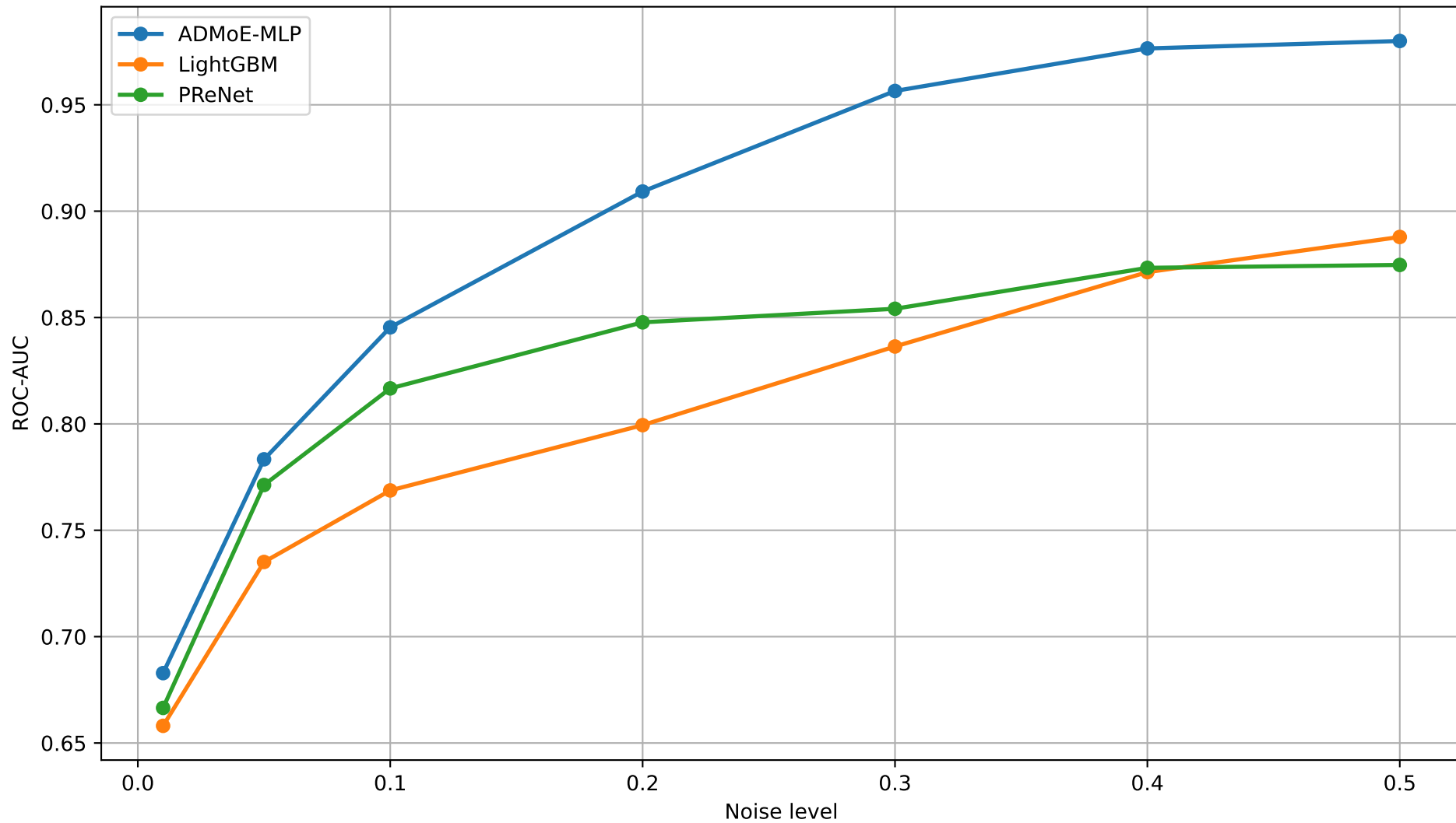
Average ROC-AUC vs Noise Level - All Datasets
