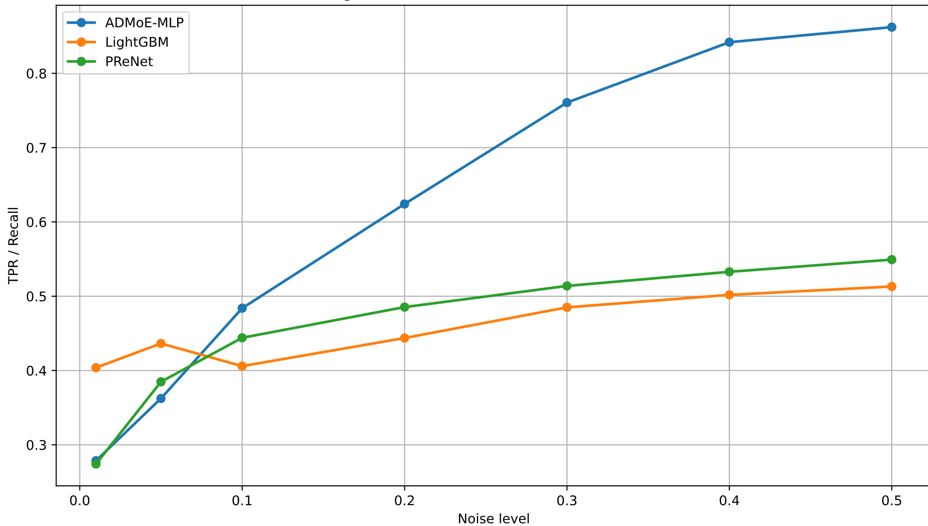
Average TPR / Recall vs Noise Level - All Datasets
